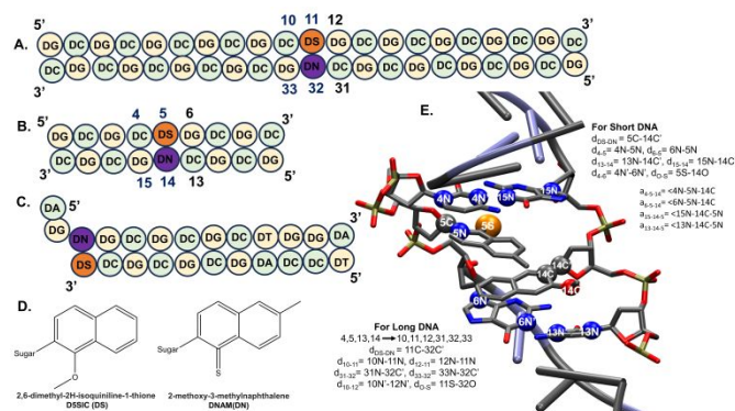
Scheme 1. Schematic representation of the sequence of DS-DN incorporated DNA duplex of A) MUD, B) MUDL and C) UUD. D. depicts the 2D representations of DS and DN. E. Distance and angles associated with DNA.
