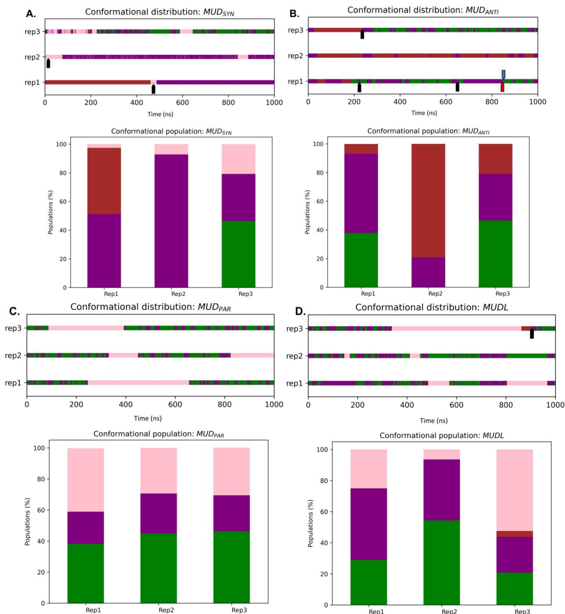
Figure 6. Distribution and population of the conformers for all the replications for A) MUD_{SYN} , B) MUD_{ANTI} , C) MUD_{PAR} and D) MUDL . WC, nWCP1, nWCP2, NWCO are designated by Green, Purple, Brown and Pink. Black pointer indicates inter-strand flipping with the change of SYN to ANTI and vice versa. Red pointer indicates inter-strand flipping with no conformational change. Blue pointer indicates intra-strand flipping.
