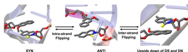
Figure 3. Conformational change through Intra- and Inter-strand flipping observed during the MD simulations.
