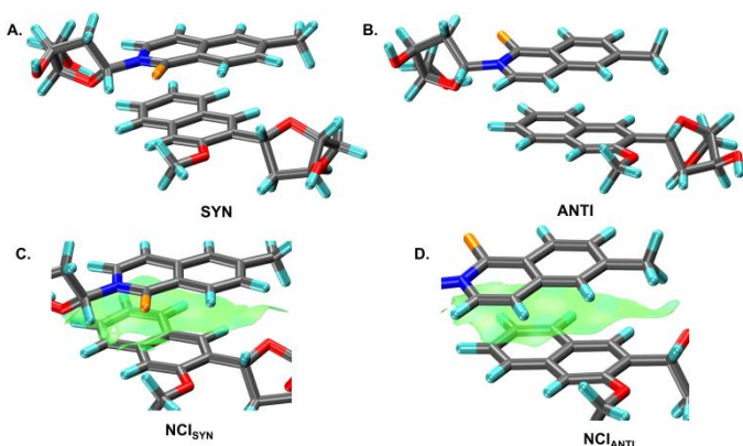
Figure 1. Optimized structures of A) SYN and B) ANTI conformers of DS-DN at \omega\text{B97x-D/6-311++g(d,p)} level. NCIPLOT of C) SYN and D) ANTI represented the non-covalent interactions between DS and DN in optimized structures.
