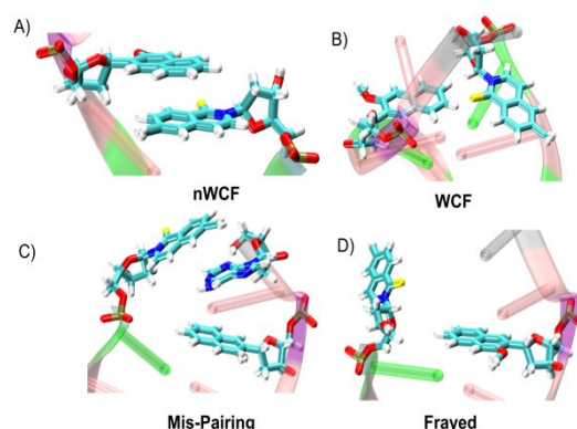
Figure 7. Snapshots of different geometries of UUD form of DNA duplex during simulations through intra and inter-strand flipping.
