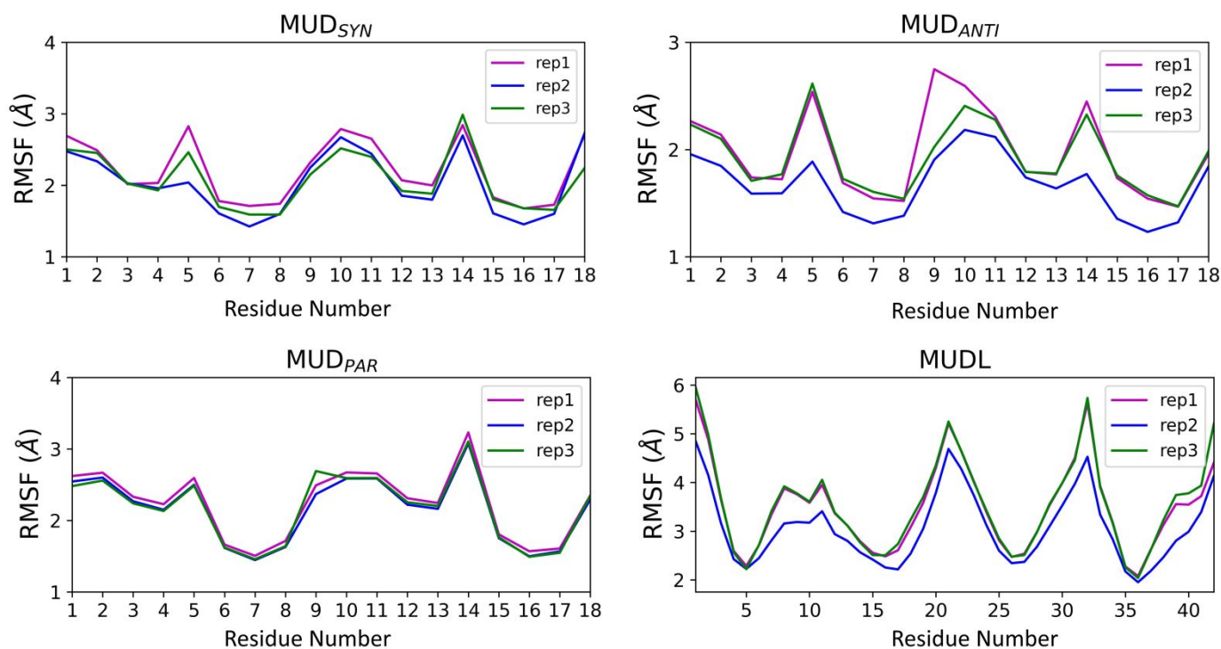
Figure 5. RMSF values for all the systems obtained from AMBER simulation.
