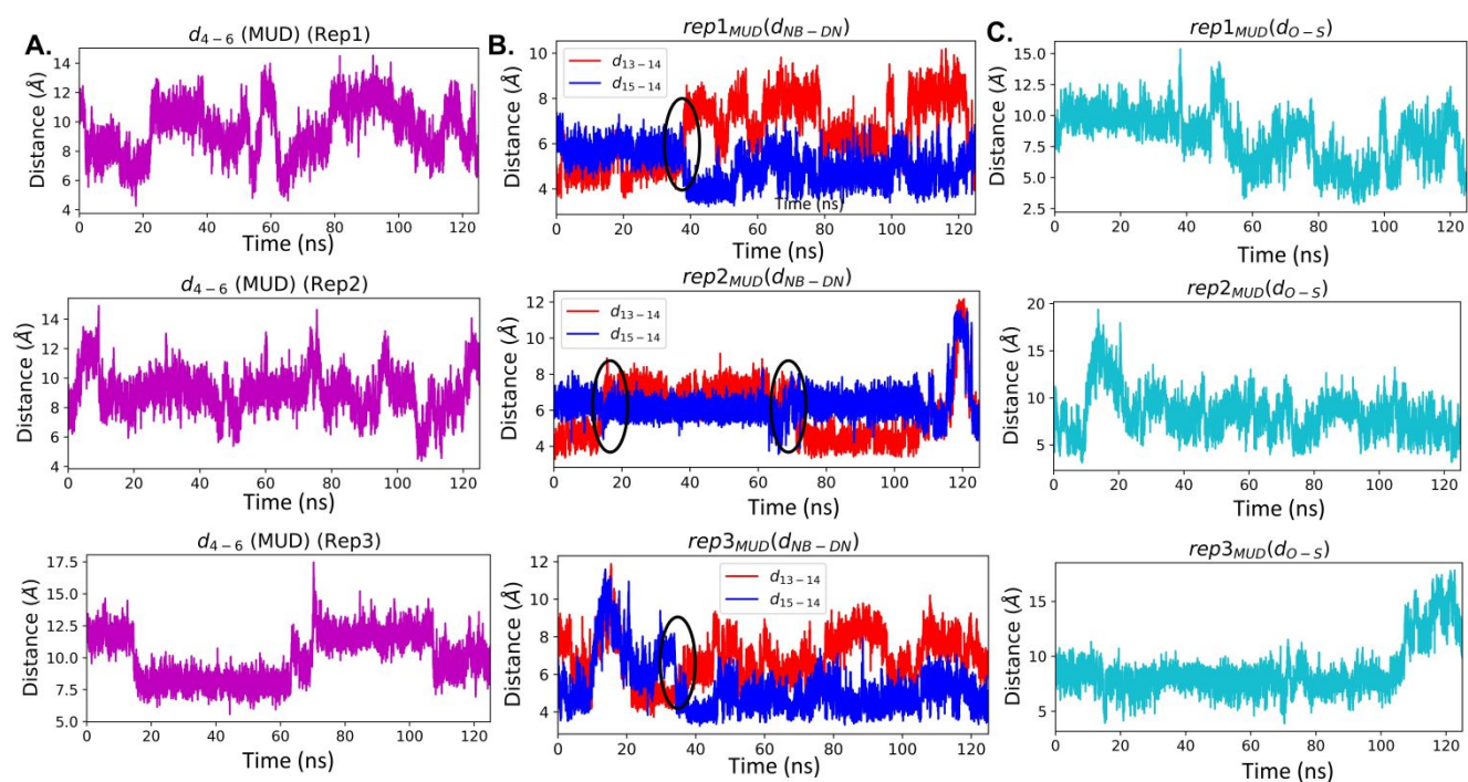
Figure 4. A) d_{4-6} value: high value depicts nWCP conformers, low values depict WC and nWCO conformers, B) DN-NB value: Circles point out inter-strand flipping, C) d_{O-S} values: Low value indicates DS and DN are in same phase, high-value DS and DN are in opposite phase for three replicates obtained from AMOEBA forcefield.
