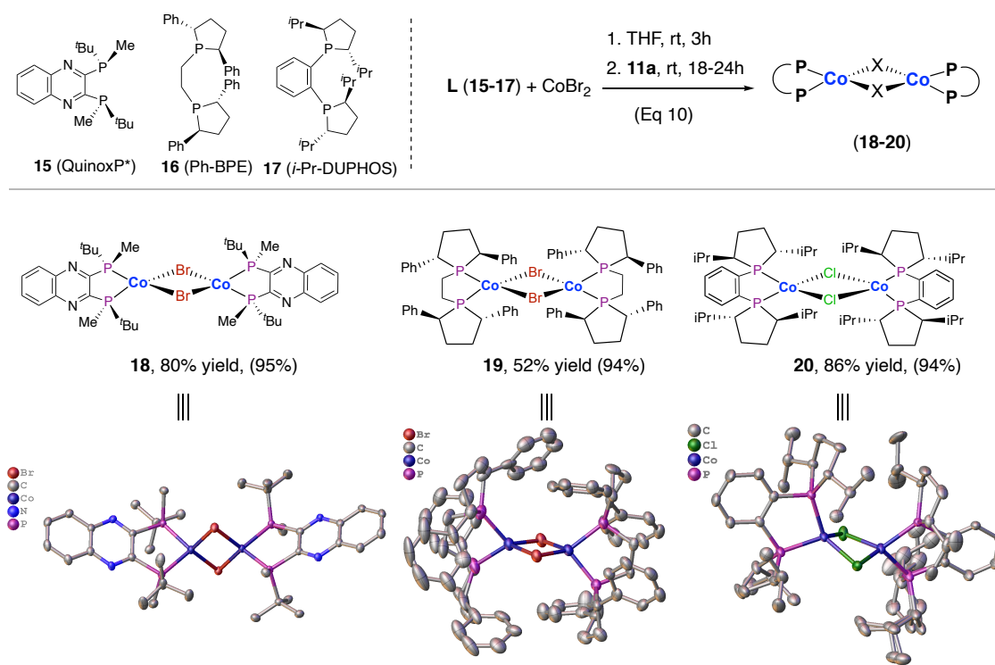
Figure 8. Co(I) complexes of chiral ligands 15 , 16 and 17 : \{[(R,R)\text{-QuinoxP}^*]\text{Co}^{\text{I}}(\mu\text{-Br})_2\}_2 ( 18 ) [Geometry around Co- tetrahedral, P-Co-P = 91.29°, Br-Co-Br = 111.50°, Co-P = 2.20 Å Co-Br (bridging) = 2.43, 2.44 Å; \{[(S,S)\text{-Ph-BPE}]\text{Co}^{\text{I}}(\mu\text{-Br})_2\}_2 ( 19 ) [Geometry around Co- tetrahedral P-Co-P = 88.70°, 89.05°, Br-Co-Br = 105.58°, 105.60°, Co-P = 2.21 Å, 2.23 Å, Co-Br(bridging) = 2.43 Å, 2.45 Å]; \{[(R,R)\text{-}i\text{-Pr-DuPhos}]\text{Co}^{\text{I}}(\mu\text{-Cl})_2\}_2 ( 20 ) [Geometry around Co- tetrahedral, P-Co-P = 89.02°, Cl-Co-Cl = 99.81°, 99.96°, Co-P = 2.21 Å, Co-Cl (bridging) = 2.32 Å, 2.34 Å]. Yields are reported after recrystallization. In brackets are the isolated yields before recrystallization. The Cl analog of 19 and the complex 20 has already been described in the literature (ref. 11b). At 50% probability ellipsoid with hydrogens omitted for clarity.
