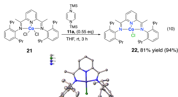
Figure 9: Solid-State structure of 22 at 50% probability ellipsoid with hydrogens omitted for clarity. Geometry around Co-square planar, N 1 -Co-N 2 = 81.63°, N 2 -Co-N 3 = 81.42°, Co-N 1 =1.91 Å, Co-N 2 =1.81 Å, Co-N 3 =1.90 Å, Co-Cl = 2.18 Å, Cl-Co-N 1 = 97.89°, Cl-Co-N 3 = 99.05°
