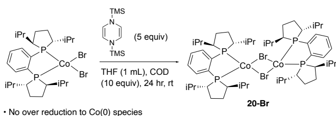
Figure 10. (Duphos)CoBr 2 reduction with excess bis-TMS-pyrazine (no over reduction)
