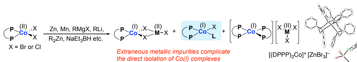
Figure 1. Reduction of (\text{P} \sim \text{P})\text{CoX}_2 for synthesis of Co I precatalysts
