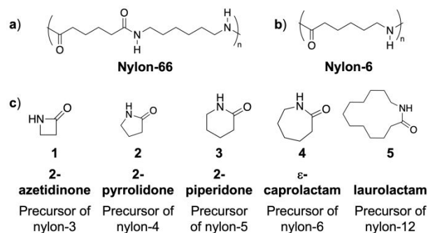
Figure 1. A) Nylon-66 polymer structure; B) Nylon-6 polymer structure; C) Precursors of common nylon polymers.
