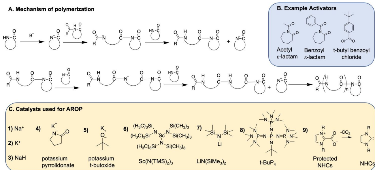
Figure 3: A) Mechanism of AROP; B) example activators; and C) the catalysts used for AROP.
