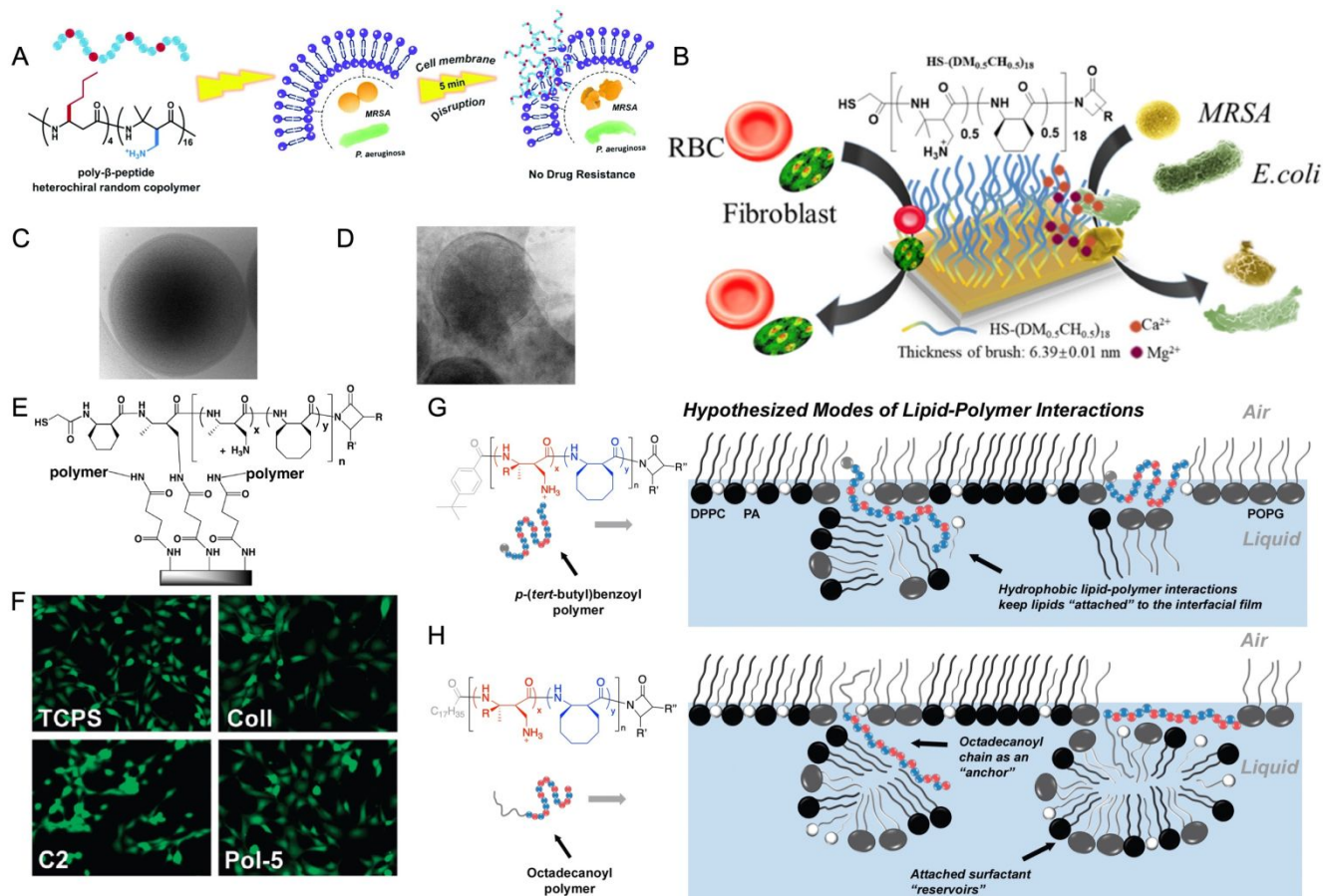
Figure 7: A. Mechanism of action HDP-mimicking nylon-3 polymers. Adapted with permission from Reference 93. Copyright © Royal Society of Chemistry. B. Thiol-terminated amphiphilic nylon 3 polymers prepared from monomers 7 and 15 are attached gold surface. The polymer coatings are non-cytotoxic against NIH-3T3 cells and are non-haemolytic but kill gram-negative E. coli and gram-positive MRSA bacterial strains. Adapted with permission from Reference 42. Copyright © American Chemical Society; C & D. Cryo-TEM images of untreated control bacteria, with cell envelope intact and cryo-TEM image of polymer-treated (co-block polymers prepared from monomers 19 and 8 bacteria resulting in cell lysis, respectively. B and C adapted with permission from Reference 45. Copyright © 2019, The Author(s); E. Amphiphilic nylon 3 polymers are immobilized on glass slides using terminal amines. F. Copolymer prepared from monomers 6 and 16 (Pol-5 in figure) display cell adhesion similar to tissue culture-treated polystyrene (TCPS in figure) and collagen coated glass slides (Coll in figure), and improved cell adhesion than amine modified glass surface (C2 in figure) in the presence of serum. E and F adapted with permission from Reference 74. Copyright © American Chemical Society; G. Mechanism of action of SP-B mimicking polymers for polymers without an octadecanoyl chain. Polymers adopt an amphiphilic conformation and insert into the lipid film, where they are able to retain attached lipids via Coulombic interactions between cationic subunits and charged lipid head groups or hydrophobic interactions between lipophilic subunits. H. Mechanism of action of SP-C mimicking polymers for polymers with an octadecanoyl chain. Octadecanoylated copolymers act as lipid “anchors” and inserts into lipid acyl chains through hydrophobic hydrocarbon chain-chain interactions, leading to enhanced surface activity. In subfigures G and H, blue spheres represent the lipophilic units while red spheres indicate cationic units. The gray sphere in the “polymer sequence” of A represents the p-(tert-butyl)benzoyl end group, while the gray line extending from the “polymer sequence” in B represents the octadecanoyl chain. G and H adapted with permission from Reference 108. Copyright © American Chemical Society.
