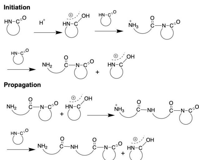
Figure 6: Mechanism of cationic ring opening polymerization.
