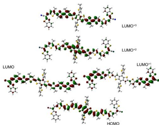
Figure 1. Contour plots of Kohn-Sham molecular orbitals of SMCN calculated with DFT as described in the text. Displayed are the HOMO, LUMO, LUMO +1 , LUMO +2 and LUMO +3 levels for contours at \pm 0.02 a.u.
