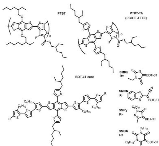
Chart 1. Common benzo[1,2-b:4,5-b']dithiophene (BDT) polymers and molecules synthesized for photobleaching and chemical degradation studies.
