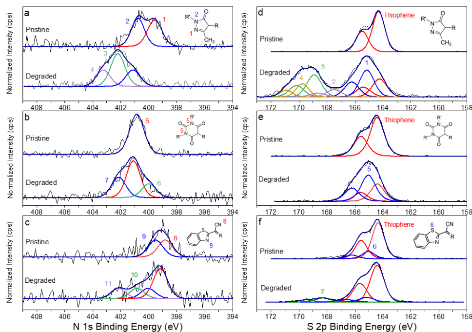
Figure 5. N 1s and S 2p core level XPS spectra with peak fits for pristine and degraded (a,d) SMPy (b,e) SMBA (c,f) SMCN.
