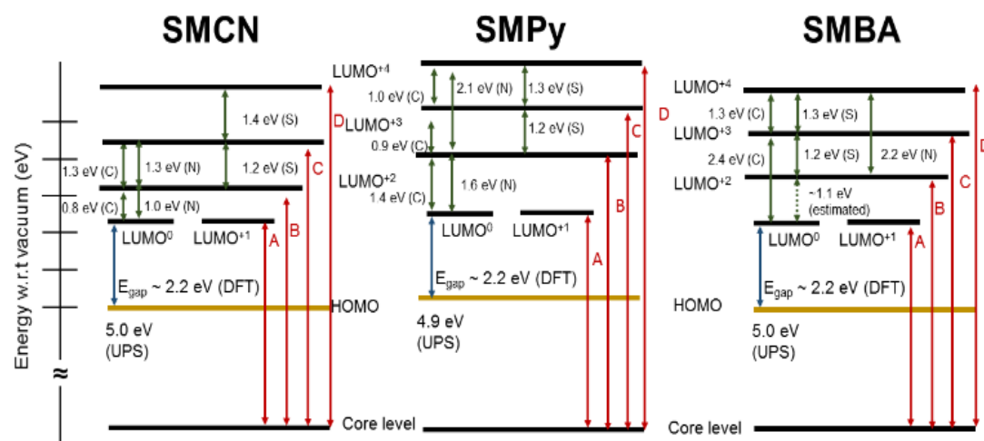
Figure 3. Energy band diagrams of the three molecules synthesized, incorporating results from UPS, XAS, and DFT. LUMO xx and LUMO xx+1 gaps were estimated from different element core transitions specified next to the value.
