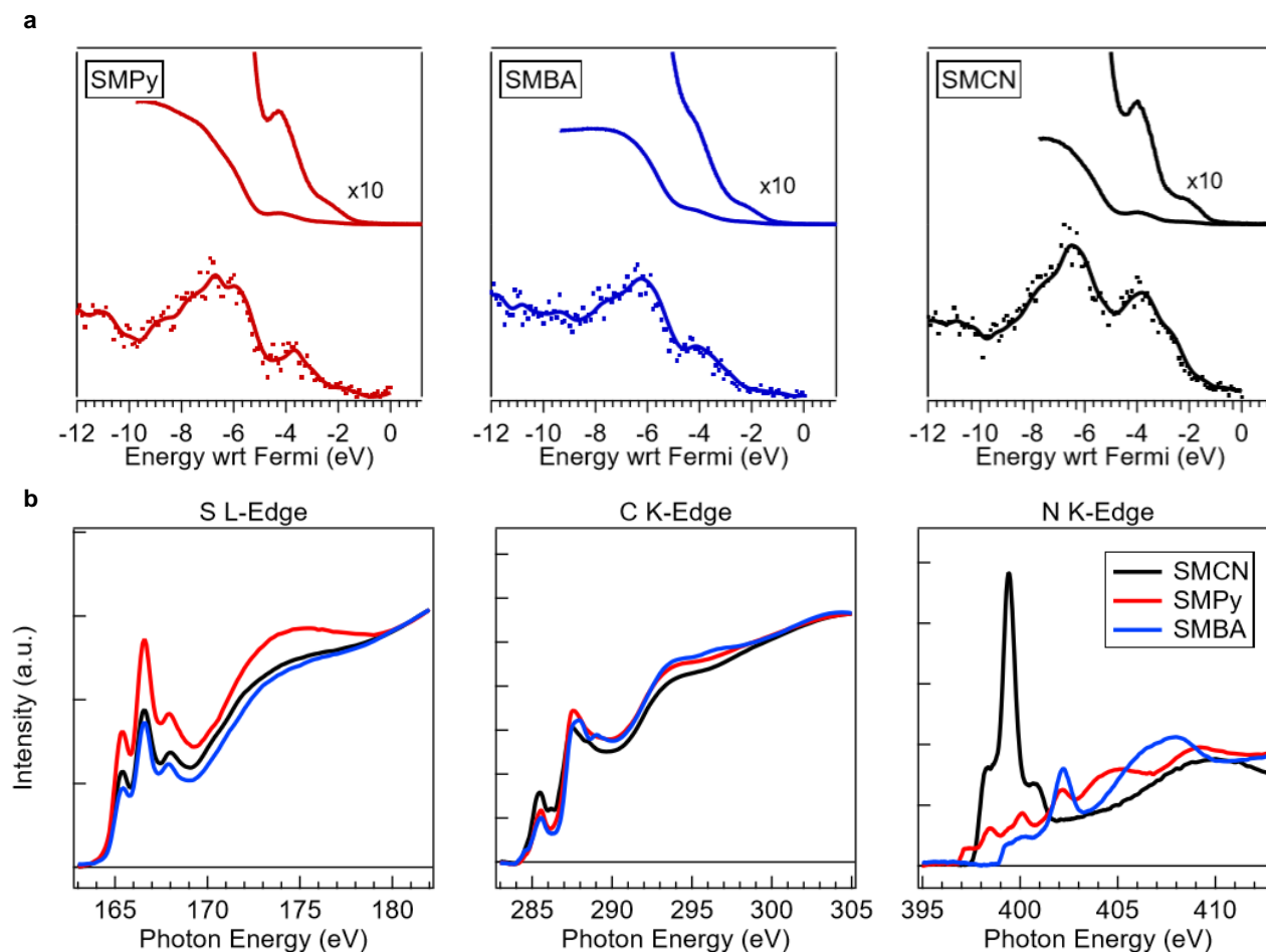
Figure 2. Photoelectron spectra of occupied and unoccupied molecular orbitals. a) Valence region collected using He I ultraviolet (top) and monochromatic Al K- \alpha x-ray (bottom) sources and b) near-edge x-ray absorbance photoelectron spectra of pristine SMPy, SMBA, and SMCN films.
