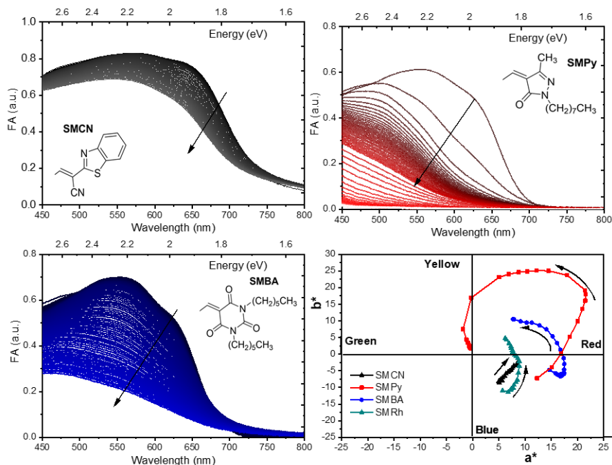
Figure 4. : UV-Vis absorbance (FA) spectra taken over a period of 11 days for (a) SMCN (b) SMPy and (c) SMBA. (d) CIE L*a*b* coordinate system representation of the UV-Vis for four molecules including SMRh.
