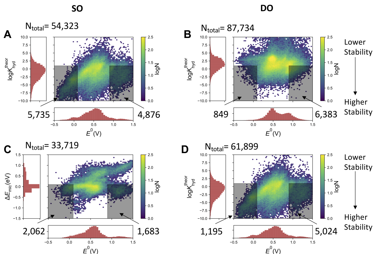
Figure 3 Correlations between calculated nucleophilic attack susceptibility and half-cell reduction potential for quinone-hydroquinone pairs. The quinone pairs are divided into two groups. The SO group contains pairs of molecules where a fully reduced hydroquinone is oxidized through a single two-proton two-electron oxidation to a quinone. The DO group contains pairs of singly two-proton two-electron oxidized quinones that may undergo a second two-proton two-electron oxidation process. N_{\text{total}} indicates the number of molecules in each plot. Shaded regions indicate molecules that have both satisfactory reduction potentials to be viable negolytes or posolytes and have relatively high thermodynamic stability with respect to the specified reaction with water.
