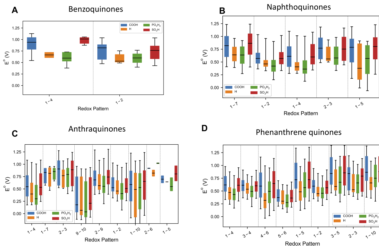
Figure 2 Reduction potential dependence on both relative ketone positions and functional groups. The numbers refer to the topology of the redox-active ketones and correspond to the labels in Figure 1. The median of each set of data is indicated with a black line. The regions bounded by the colors indicate the range of the 5th and 95th percentile of reduction potentials. The lines extend out to the maximum and minimum reduction potential for each substitution and ketone topology.
