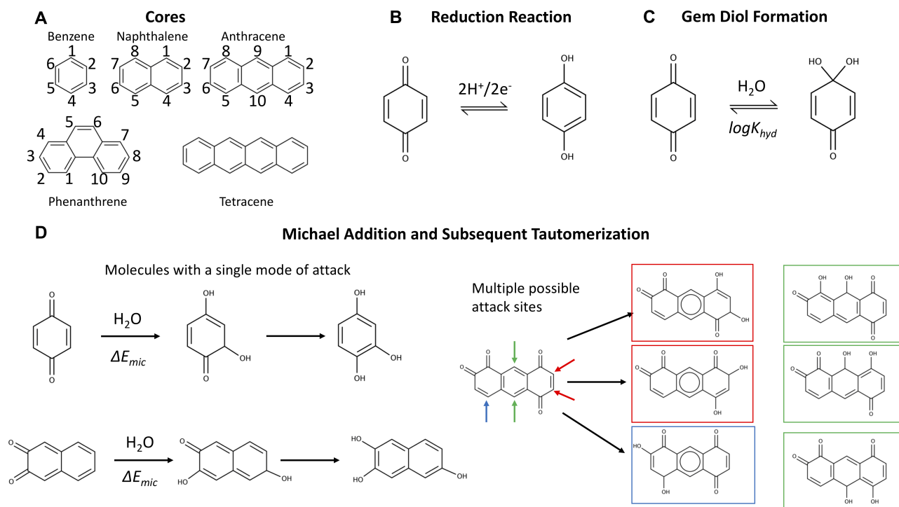
Figure 1 A) All backbones (without oxidation topologies indicated) considered in this study. The molecules discussed in detail are labeled to give a short description of the redox-active sites in a given molecule. B) The redox reaction of quinones in acidic aqueous flow batteries: the two-proton two-electron reduction of two ketones to two hydroxyl groups C) Mechanism for gem-diol formation, which is reversible but hampers kinetics. D) Illustrations of Michael addition (irreversible) on molecules with a single vulnerable site (with subsequent tautomerization shown) and on molecules with multiple vulnerable attack sites. Michael addition can also occur on substituted sites, where it becomes a substitution reaction.
