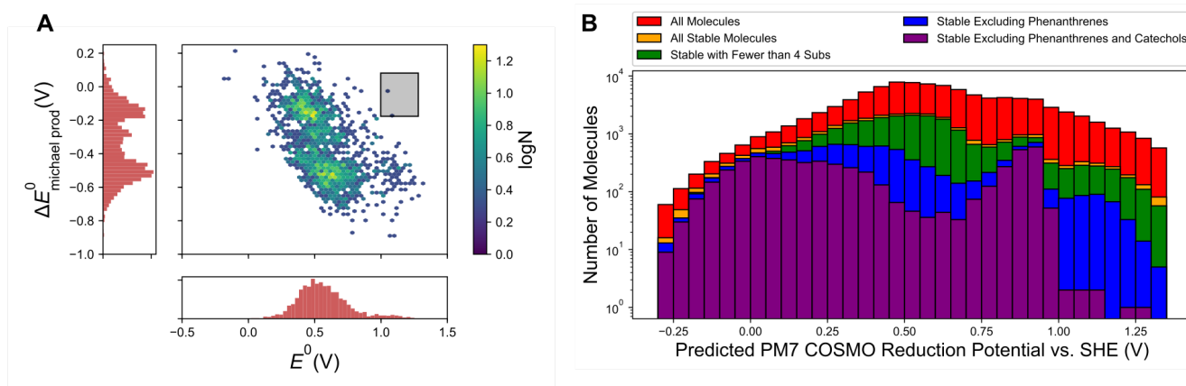
Figure 4 A) Change in the reduction potential of a molecule upon Michael addition, 1763 molecules pictured. The desired region, high potential molecules that show almost no change in reduction potential upon Michael addition, is shaded in the black box and contains only two molecules (sulfonated 1-4 benzoquinones), which are shown in Figure S8. B) Plot of the redox potential distributions of various sets of molecules, as indicated in the legend. Molecules are defined as “stable” if they have the following criteria 1) PM7 COSMO Michael addition energy < 0.03 eV and 2) \log K_{hyd} < 1.0 .
