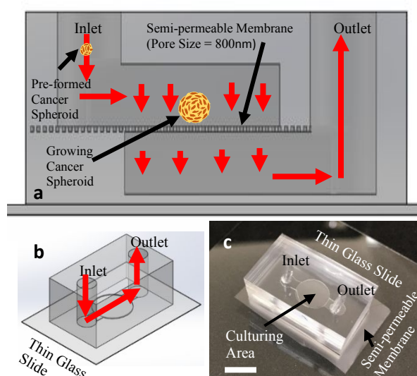
Figure 1 Microfluidic device schema depicting device structure and cancer cell capture function utilizing semi-permeable membrane. Flow direction indicated by red arrows. (a), Device schema cross-section. (b), Device schema overview. (c), Image of sample microfluidic device utilized in experimental testing (white scale bar is 3mm long).
