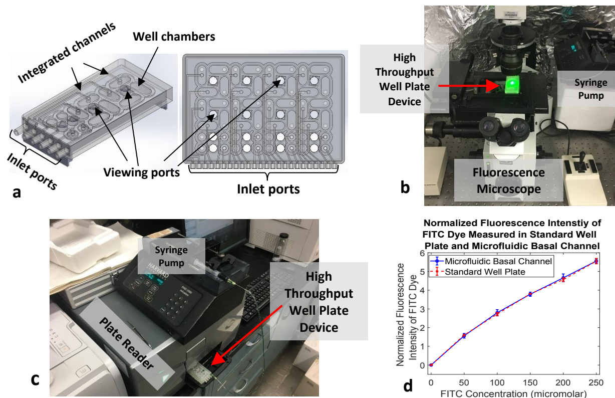
Figure 5. Representative prototype of high-throughput array microfluidic system allowing 16 therapeutic screening tests to be run simultaneously. a , 3D model of high-throughput array microfluidic well plate designed for use with high-throughput imaging and data collection systems. b , Prototype well plate system manufactured via 3D printing being used to test data collection from a fluorescent microscope. c , Prototype well plate system being tested with a plate reader to verify data collection. d , Normalized fluorescence intensity data of FITC dye flow through the prototype high-throughput array system. Fluorescence intensity was measured at various dye concentrations while passing through the device and compared to fluorescence intensities at the same concentrations in standard well plates. The data collected by both methods are in good agreement, indicating that the prototyped system functions well plate reader data collection. Data collection tests were run five times ( n=5 ) to achieve statistical significance.
