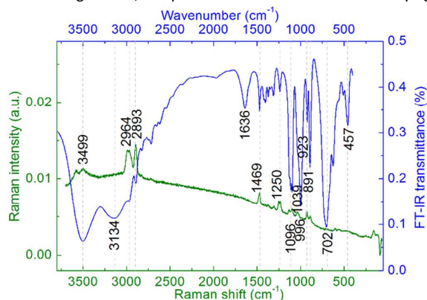
Figure 3. FT-IR and Raman spectra of single-crystal gl-\epsilon-Al_{13} .
