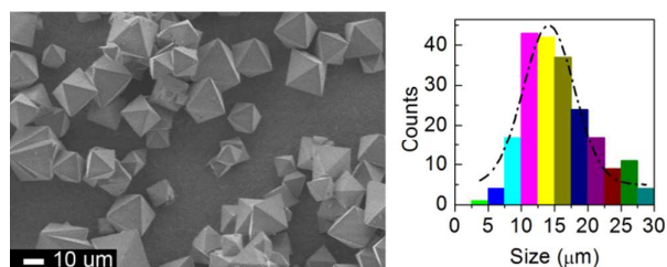
Figure 1. SEM and particle-size distribution of single-crystal gl-\epsilon-Al_{13} .
