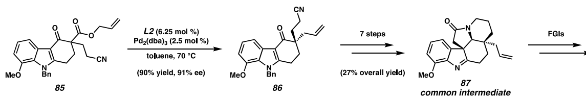
Scheme 11 Shao's total synthesis of (-)-Limaspermidine (6)
