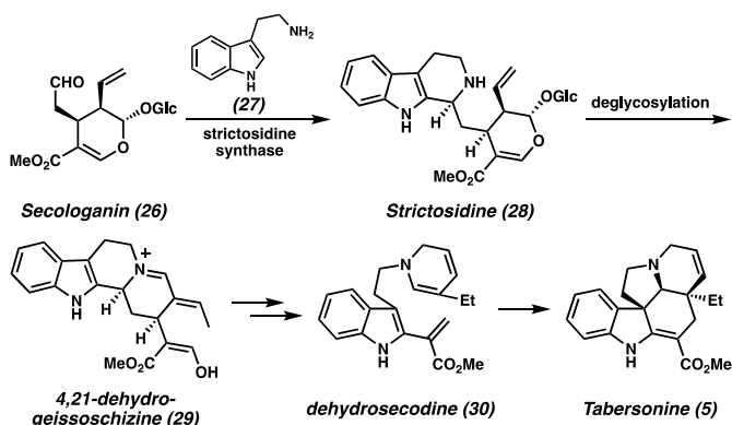
Scheme 1 Proposed biosynthetic pathway to Aspidosperma alkaloids
