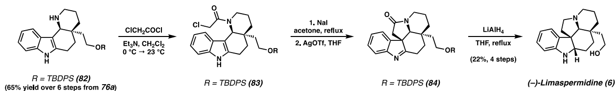
Scheme 11 Shao's total synthesis of (-)-Limaspermidine (6)
