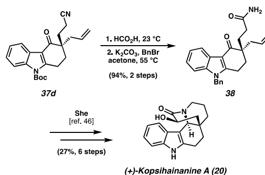
Scheme 4 Enantioselective formal synthesis of (+)-Kopsihainanine A ( 20 )
