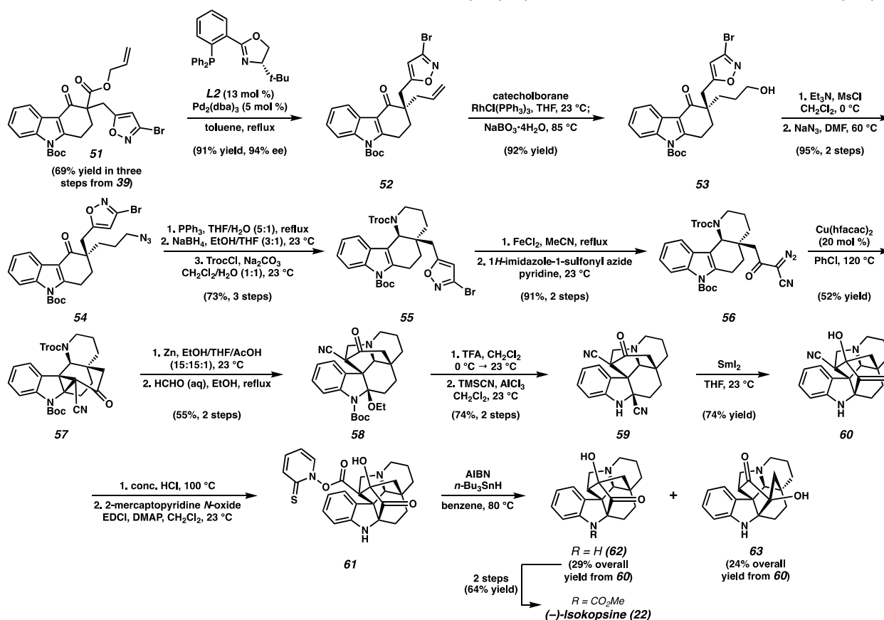
Scheme 7 Qin's highly stereoselective core construction enabled by early enantioselective Pd-catalyzed allylic alkylation
