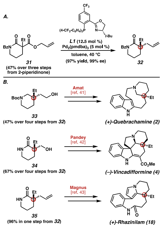
Scheme 2 A) Pd-catalyzed allylic alkylation; B) Chiral building blocks in the formal synthesis of Aspidosperma alkaloids
