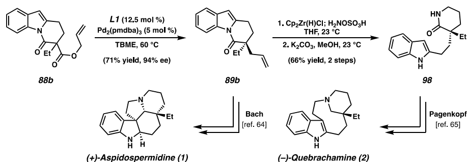
Scheme 15 Asymmetric formal syntheses of (+)-Aspidospermidine ( 1 ) and (–)-Quebrachamine ( 2 )
