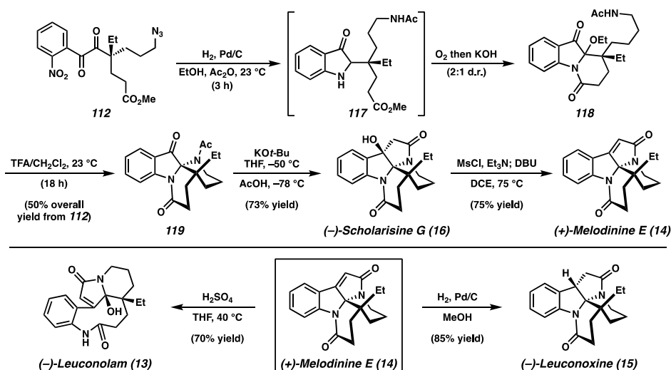
Scheme 20 Zhu's unified approach to alkaloids 13–16
