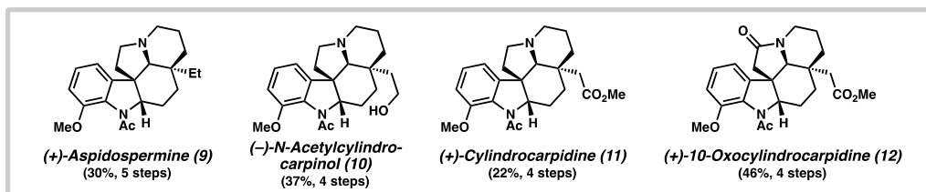
Scheme 12 Shao's total syntheses of C12-methoxy alkaloids 9–12
