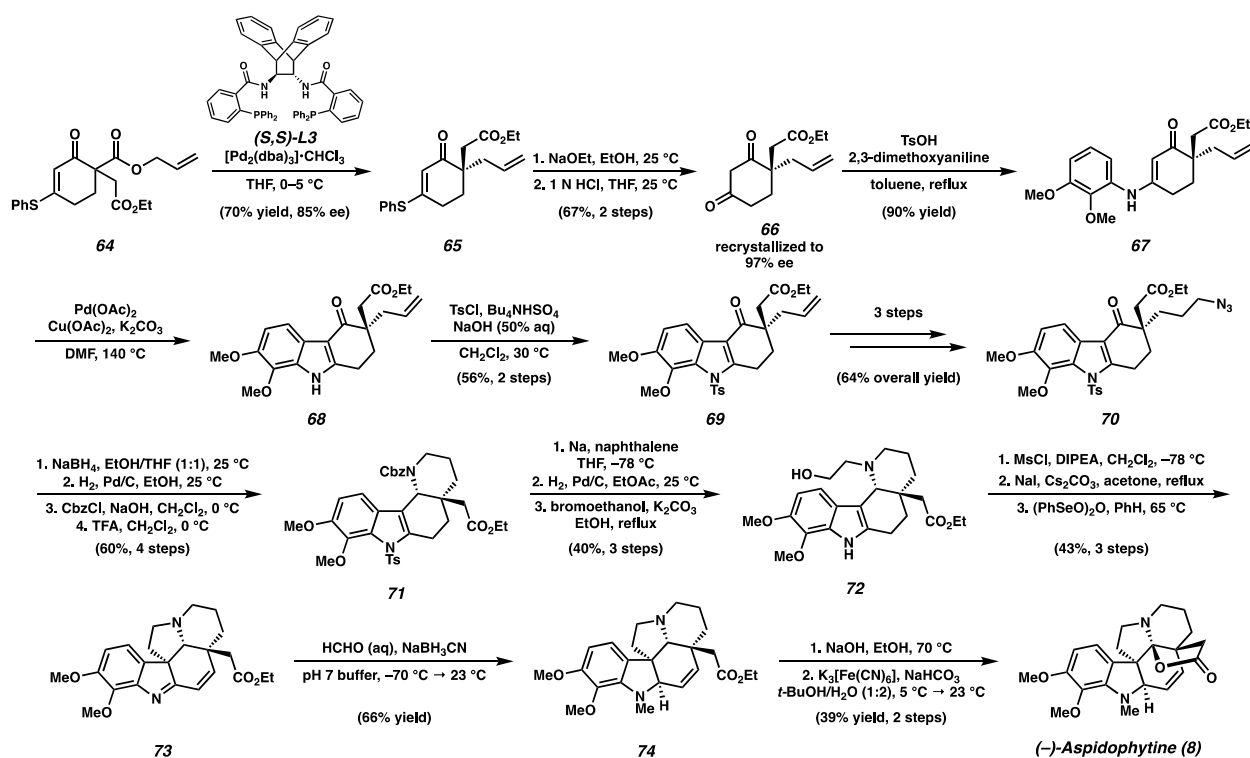
Scheme 9 Qiu's total synthesis of (-)-Aspidophytine ( 8 )
