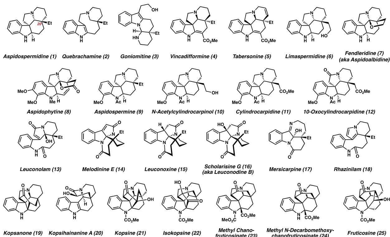
Figure 1 Representative Aspidosperma and related alkaloids.
