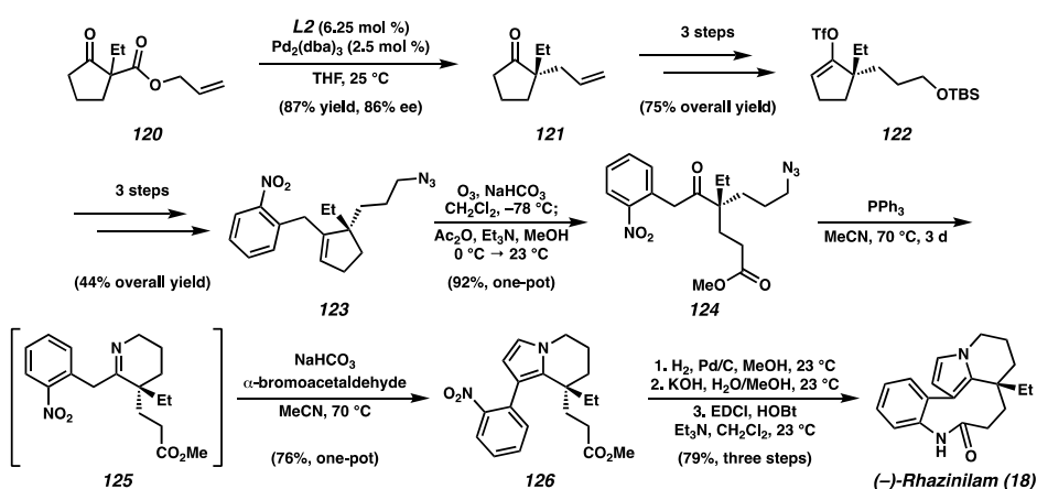
Scheme 21 Zhu's total synthesis of (-)-Rhazinilam (18)
