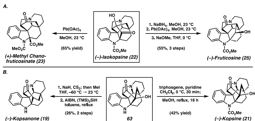
Scheme 8 Qin's divergent syntheses of multiple Kopsia alkaloids
