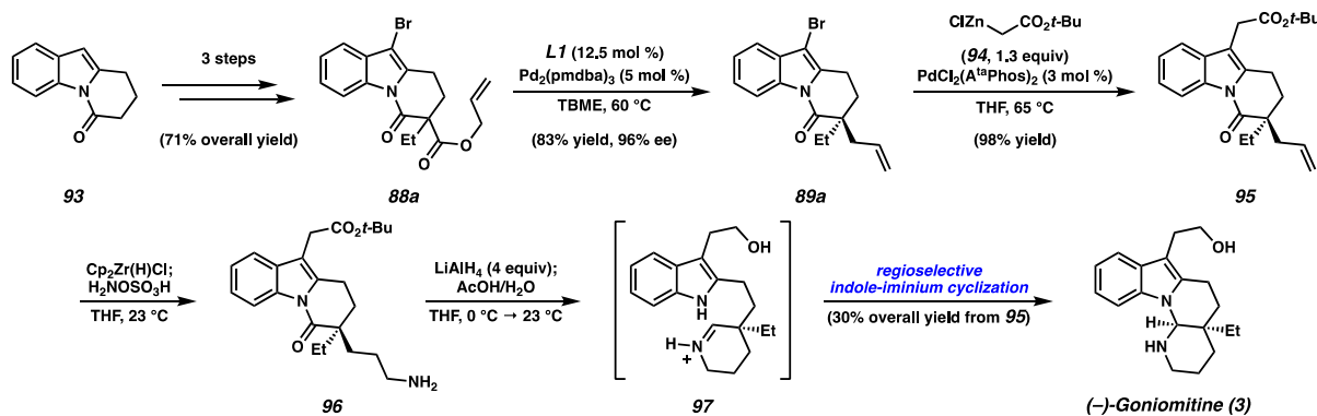
Scheme 14 Stoltz's catalytic enantioselective synthesis of (–)-Goniomitine ( 3 )
