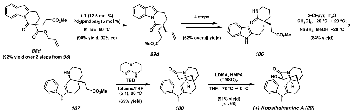
Scheme 18 Stoltz's formal synthesis of (+)-Kopsihainanine A ( 20 )
