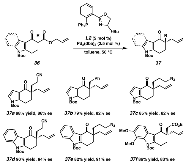
Scheme 3 Selected examples from Lupton's enantioselective Pd-catalyzed allylic alkylations of indolone and carbazolone substrates
