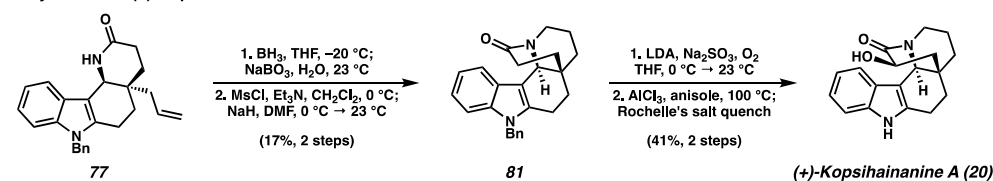
Scheme 10 Shao's initial report on the Pd-catalyzed allylic alkylation of carbazolone substrates
