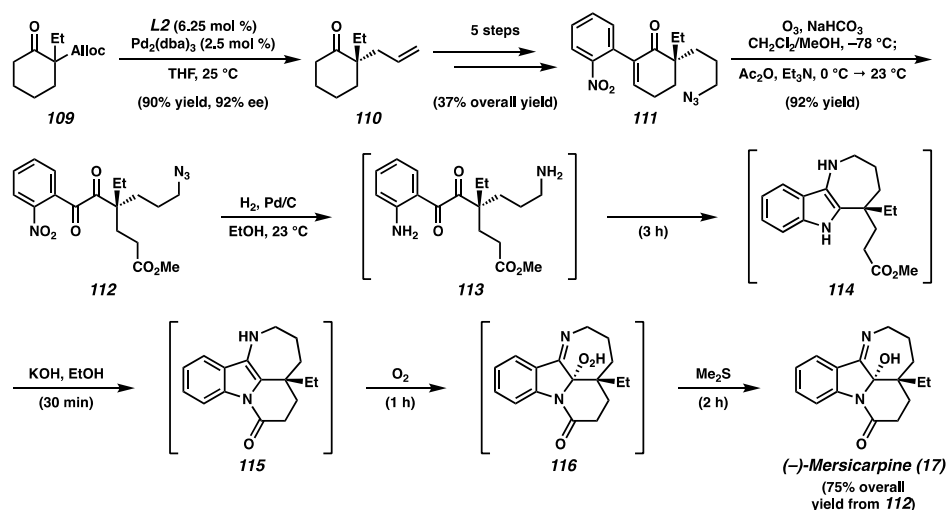
Scheme 19 Zhu's total synthesis of (–)-Mersicarpine ( 17 )
