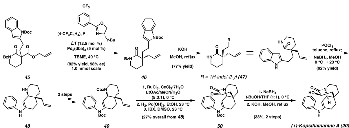
Scheme 6 Mukai's total synthesis of (+)-Kopsihainanine A ( 20 )
