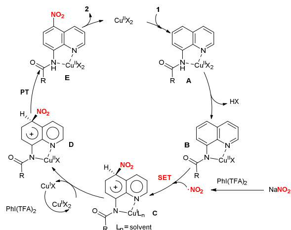
Scheme 5 plausible mechanism
