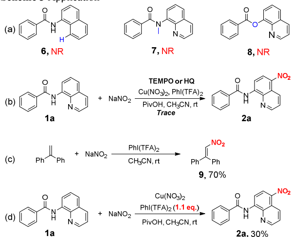
Scheme 4 control experiments
