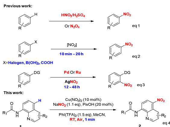
Scheme 1 A series of strategies leading to nitroarenes
