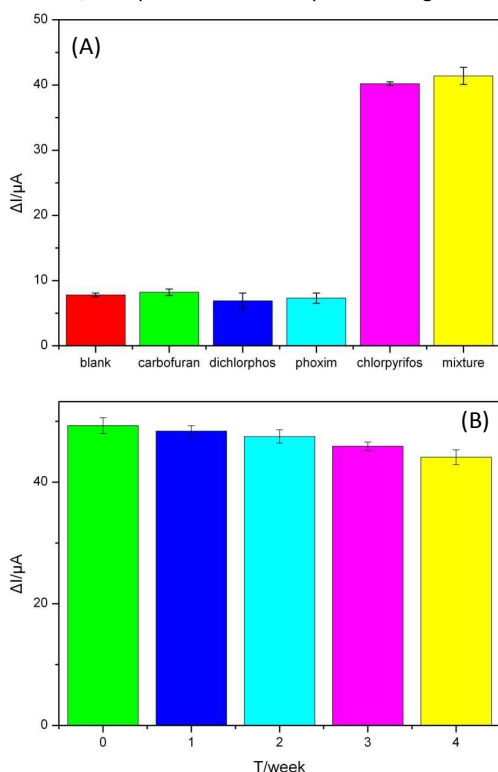
Fig. 6. (A) Selectivity evaluation of the aptasensor detection of chlorpyrifos (50 ng/mL) against the interference molecules, carbofuran, dichlorphos, phoxim and the mixture consisting of the above interference and chlorpyrifos. (B) The stability assessment of the proposed aptasensor.
