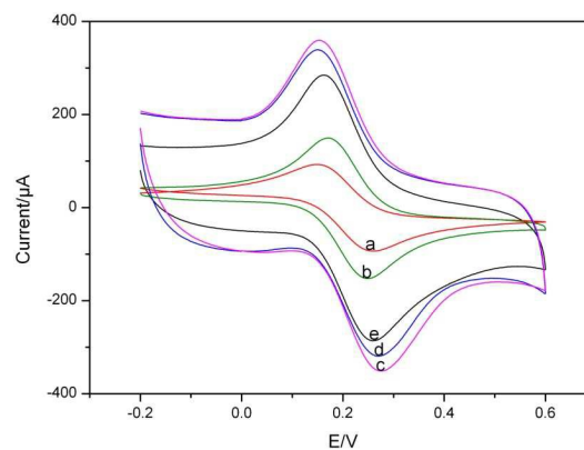
Fig. 2 CVs of modified GCE recorded in 0.1 M PBS (pH 7.0) containing 5.0 mM [Fe(CN)_6]^{3-/4-} and 0.1 M KCl: (a) bare GCE; (b) OMC/GCE; (c) Fc@MWNTs/OMC/GCE; (d) Apt/Fc@MWNTs/OMC/GCE; (e) BSA/Apt/Fc@MWNTs/OMC/GCE.
