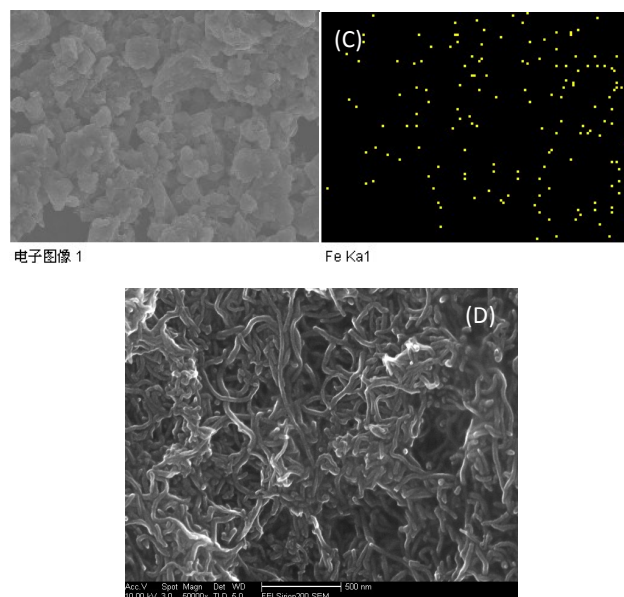
Fig. 1 SEM images of (A) OMC, (B) Fc-MWNTs, (D) Fc-MWNTs/OMC; (C) EDS for Fe elemental distribution on the surface of Fc@MWNTs
