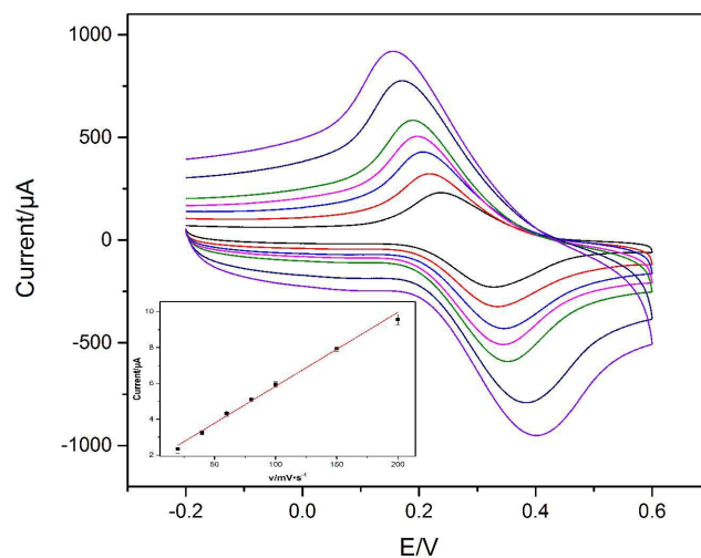
Fig. 3 Cyclic voltammograms of the Apt/Fc@WMCNTs/OMC/GCE in 0.1 M PBS (pH 7.0) at scan rates (from inner to outer) 20, 40, 60, 80, 100, 150 and 200 mV s -1 , respectively. Inset: the relationship between scan rates and peak currents.
