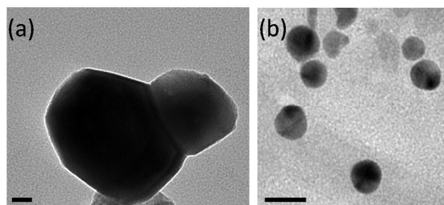
Fig. 2 TEM images of \text{Eu}^{3+} , \text{Ti}^{4+} , \text{Mg}^{2+} doped \text{Gd}_2\text{O}_2\text{S} nanoparticles after 2h annealing at 700^{\circ}\text{C} under argon. Scale bars are 20 nm.
