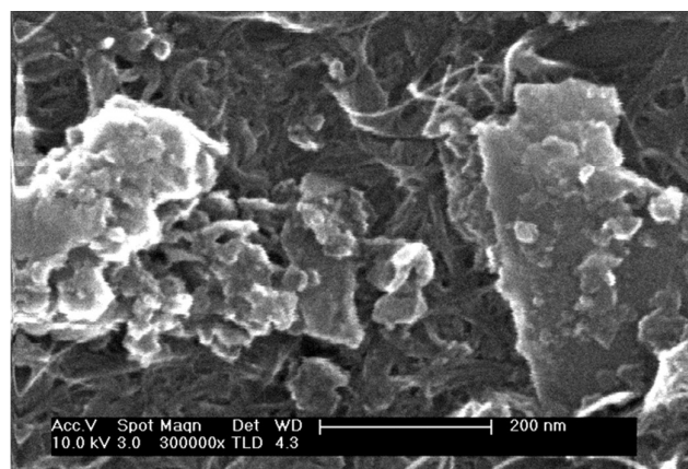
Fig. 3 FE-SEM image of a hybrid GNPs/SWCNTs-OTE fabricated by filtration of 0.3 mL of the GNPs and 0.58 mL of the SWCNTs dispersions.
