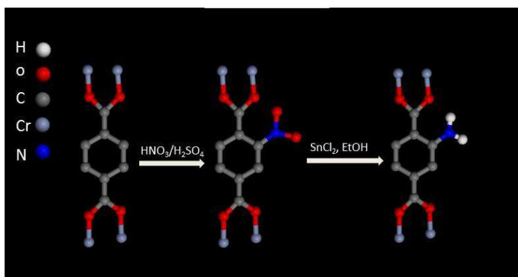
Fig. 3 Representation of the route for preparing \text{NH}_2\text{-MIL-101}(\text{Cr}) from \text{MIL-101}(\text{Cr}) via PSM.
