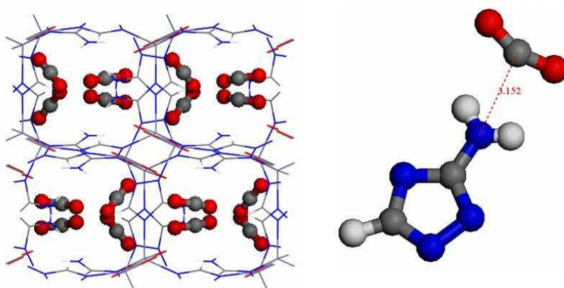
Fig. 6 Locations of CO 2 adsorbed in the Zn 2 (Atz) 2 . Ball: blue, N; white, H; gray, C.
