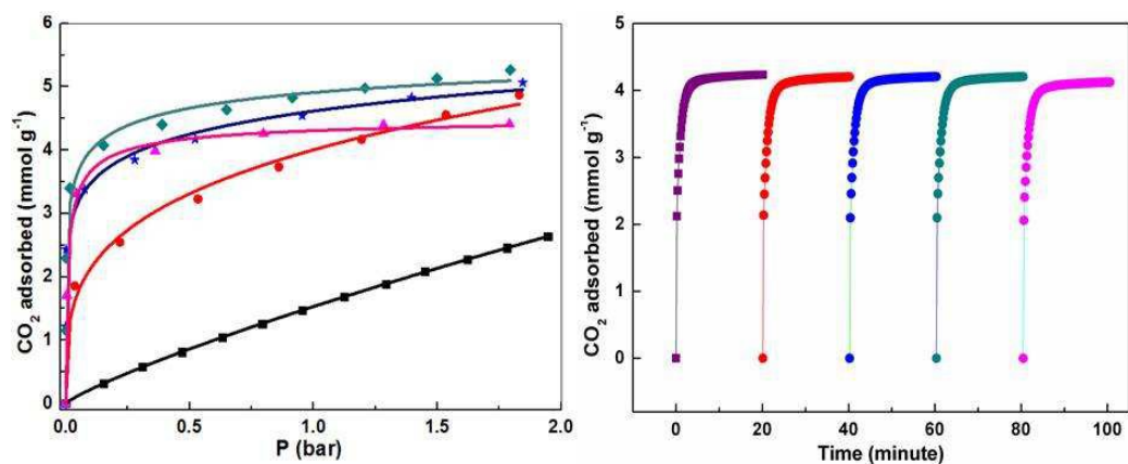
Fig. 9 (left) \text{CO}_2 adsorption isotherms of MIL-101(Cr) before and after PEI loading at 25 °C. Symbol: ■MIL-101, ● PEI-MIL-101-50, ★PEI-MIL-101-75, ◆PEI-MIL-101-100 and ▲PEI-MIL-101-125. (right) Cycling \text{CO}_2 adsorption kinetics of PEI-MIL-101-100. Reproduced from ref. 62 with permission of Nature Publishing Group.
