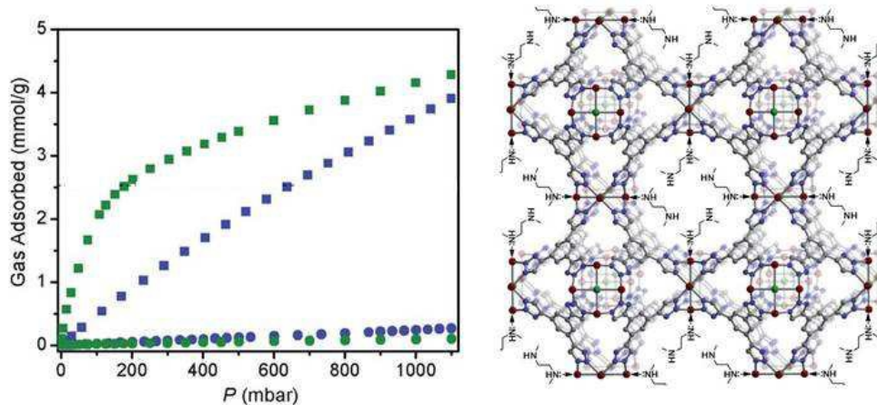
Fig. 8 Isotherms for \text{CO}_2 (squares) and \text{N}_2 (circles) adsorption at 25 °C for mmen-CuBTTri (green) and CuBTTri (blue). Reprinted from ref. 58 with permission from Royal Society of Chemistry.
