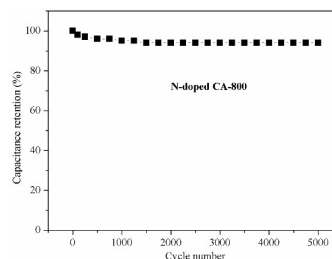
Figure 9. The cycling stability of N-doped CA-800 at a current density of 1.0 A g -1 .
