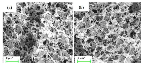
Figure 1. SEM of N-free CA-800 (a) and N-doped CA-800 (b).
