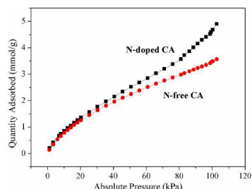
Figure 6. \text{CO}_2 adsorption isotherms of N-free CA-800 and N-doped CA-800.
