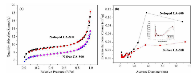
Figure 5. N_2 adsorption-desorption isotherms (a) and pore size distributions calculated from the adsorption isotherms (b) of N-free CA-800 and N-doped CA-800.
