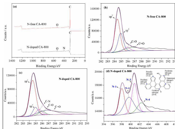
Figure 4. Surveys of N-free CA-800 and N-doped CA-800 (a), high-resolution C1s spectra of N-free CA-800 (b) and N-doped CA-800 (c), high-resolution N1s spectrum of N-doped CA-800 (d).
