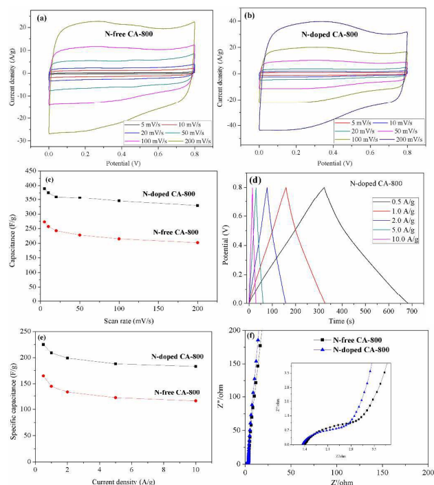
Figure 8. Electrochemical behaviours of N-free CA and N-doped CA: CV curves at different scan rates (a, b), specific capacitances as a function of scan rate (c), galvanostatic charge/discharge curves at different current densities (d), specific capacitances as a function of current density (e), and Nyquist plots (f).
