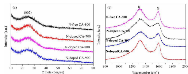
Figure 3. XRD pattern (a) and Raman spectra (b) of N-free CA and N-doped CA.
