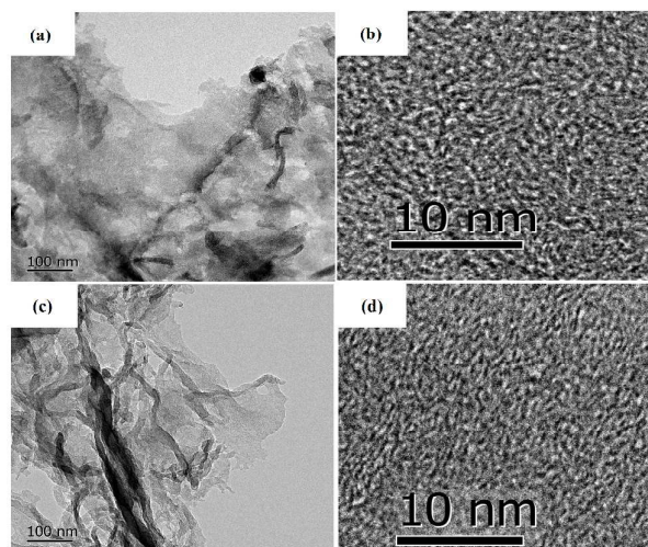
Figure 2. TEM images of N-free CA-800 (a, b) and N-doped CA-800 (c, d).
