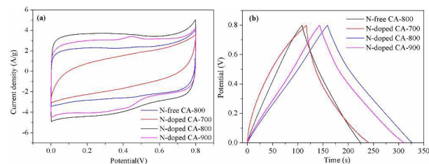
Figure 7. CV curves at 20 \text{ mV s}^{-1} (a) and galvanostatic charge/discharge curves at 1.0 \text{ A g}^{-1} (b) of carbon aerogels.
