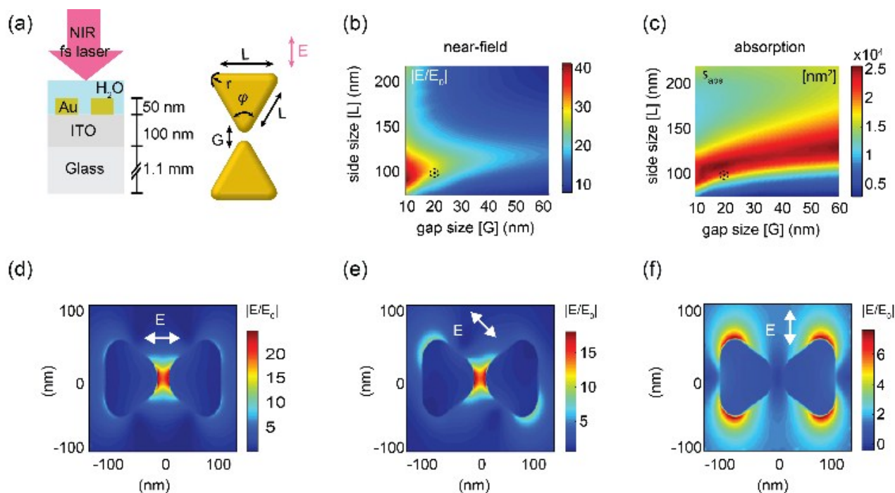
FIGURE 1 Designing a AuBT array for efficient pressure and bubble generation. (a) Cross-section and top view of the AuBT structure used in the modelling. Irradiation was applied from the top in water environment. The radii of curvature was fixed to r = 20 nm, while the edge length ( L ) and the gap distance ( G ) were variables in the design study. The flare angle ( \phi ) was fixed at 60 degrees. (b) Maximum near-field enhancement at mid-height and (c) AuBT absorption cross-section as a function of G and L for LP excitation. The black dot indicates the selected geometry. Figures (d), (e) and (f) represent the calculated near-field enhancement at mid-height for three different polarizations for G = 20 nm and L = 100 nm.
