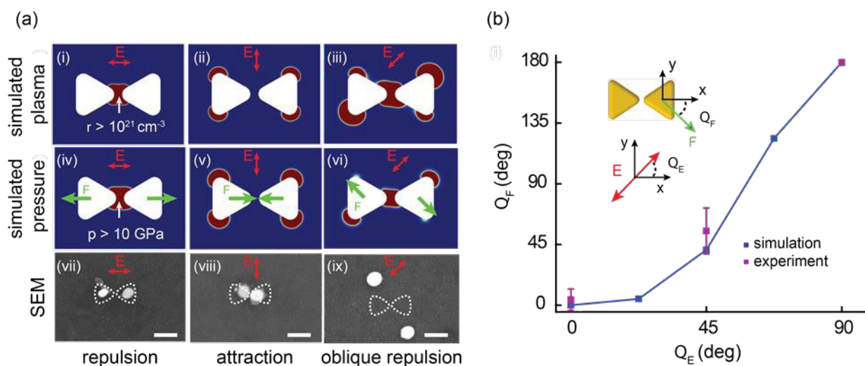
FIGURE 4 Polarization-dependent generation of pressure stimuli following fs laser excitation of AuBT. (a) (i-iii) Nano-plasma simulations at 120 \text{ mJ/cm}^2 . The red areas indicate regions where the electronic density reaches the optical breakdown threshold in water ( n > 10^{21} \text{ cm}^{-3} ) at the pulse maximum. (iv-vi) Isochoric pressure reached in water after irradiation at 120 \text{ mJ/cm}^2 . The red area shows the region where pressure is larger than 10 \text{ GPa} . The green arrows indicate the equivalent force acting on the nano-triangle center of mass. Torque is not shown. (vii-ix) SEM pictures showing polarization-dependent alteration of AuBT morphology at 120 \text{ mJ/cm}^2 . Scale bars correspond to 100 \text{ nm} . (b) Simulated force direction acting to the nano-triangle center of mass for various polarizations (blue line). Experimentally observed displacement of the nano-triangle due to the polarization-controlled directional pressure stimuli (purple squares). The error bar corresponds to the standard deviation of 4 measurements.
