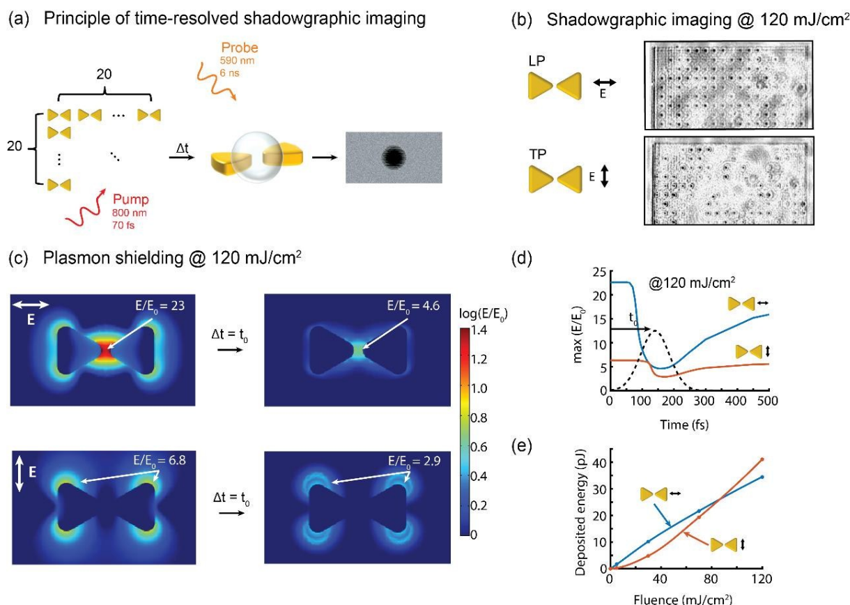
FIGURE 3 Principle of time-resolved shadowgraphic imaging. The sample is a 20 x 20 array of AuBT (periodicity: 5 \mu m). (b) Arrays of nanobubbles generated by fs laser irradiation with LP and TP polarizations. Bubbles were detected 15 ns after their generation. (laser fluence 120 mJ/cm 2 ) (c) Simulated field enhancement distribution for LP (top) and TP (bottom) polarizations at t=0 and t=t_0 , corresponding to the peak incident intensity. Field enhancement is shown at the nano-triangle mid-height plane. (laser fluence 120 mJ/cm 2 ) (d) Simulated time-evolution of the maximal near-field enhancement for LP and TP polarizations. The dashed line shows the fs laser pulse. (laser fluence 120 mJ/cm 2 ) (e) Total energy deposited in the system as a function of the laser fluence for LP and TP excitation.
