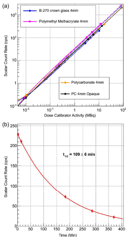
Fig. 5 (a) Study of the linearity of the SiPM signal over four orders of magnitude of [ ^{18}\text{F} ]fluoride activity in 4 mm thick substrates. The uncertainties comprise the \sqrt{n} statistical component as well as a 10 % systematic error. (b) Determination of [ ^{18}\text{F} ]fluoride half-life based on multiple measurements taken over several half-lives.
