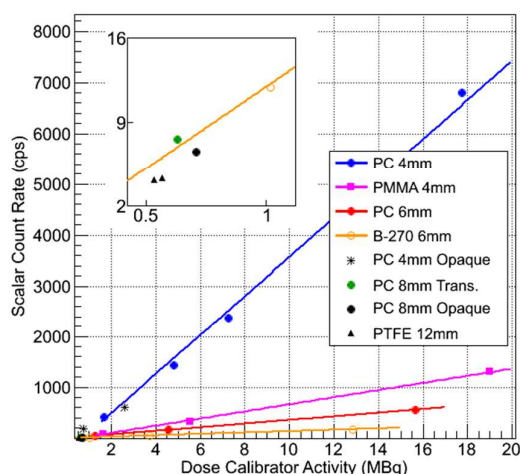
Fig. 7 Activity of the PET radiotracer, [ ^{68}\text{Ga} ]gallium-citrate, versus the SiPM count rate for a variety of microfluidic chip substrates and thicknesses. The inset results highlight measurements taken using opaque chips.
