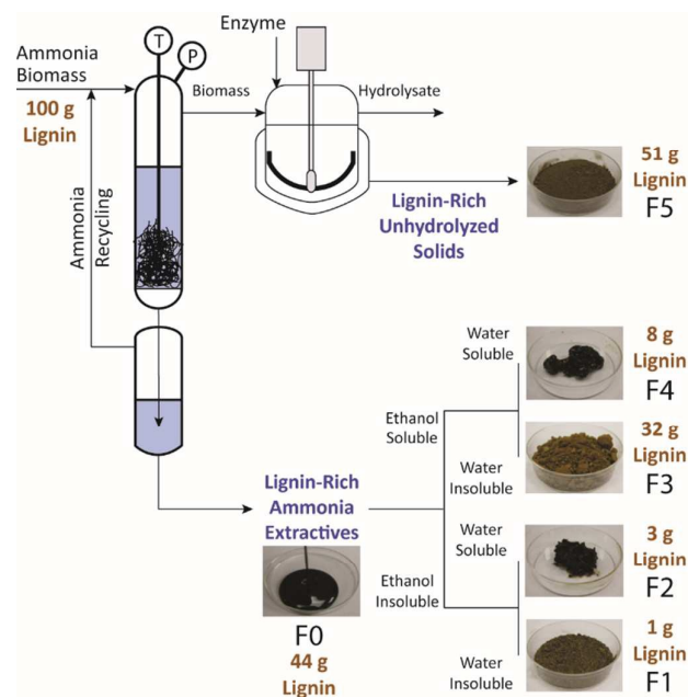
Scheme 2 Biomass fractionation process based on ammonia extraction of corn stover, followed by sequential ethanol and water precipitation of lignin-rich ammonia extractives. Mass yields of lignin for each fraction are given based on 100 g lignin input.
