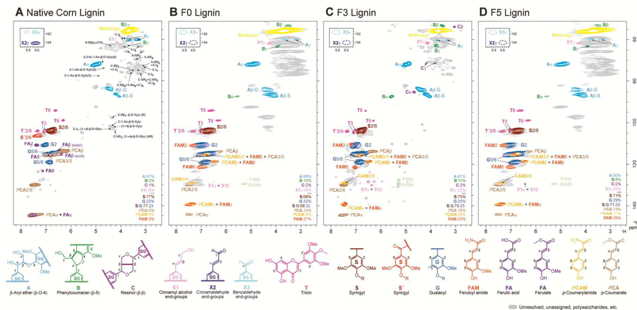
Fig. 1 2D-HSQC NMR of A) Native corn lignin; B) F0; C) F3, and D) F5. Legend: C-I, cellulose internal unit; C-NR, cellulose non-reducing end unit; C-R \alpha , cellulose reducing end unit, \alpha -anomer; C-R \beta , cellulose reducing end unit, \beta -anomer; X-I, xylose internal unit; X-NR, xylan non-reducing end unit; X-R \alpha , xylan reducing end unit, \alpha -anomer; X-R \beta , xylan reducing end unit, \beta -anomer; R, reducing end; NR, non-reducing end 44 . NMR spectra have correlation contours color-coded to match those of the aromatics and lignin structures shown here. Percentages are integrals of key component correlation contours and are not absolute quantifications; they are for comparative purposes only. 40 The aliphatics are based on A+B+C = 100%; similarly, aromatics are based on S+G = 100%. Note that some correlations are not evident at the contour level plotted, but are visible at lower contour levels and can still be integrated.
