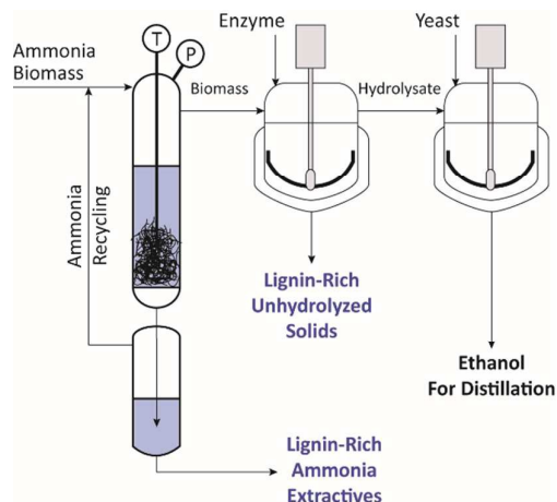
Scheme 1 Major steps in the Extractive-Ammonia (EA) process.
