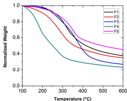
Fig. 2 Thermogravimetric curves for the various biomass fractions (F1-F5) derived from the EA pretreatment of corn stover. The heating ramps for all the samples were set at 10 °C/min.
