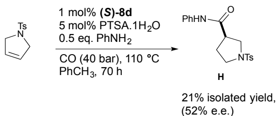
Scheme 5. Palladium catalysed enantioselective intermolecular hydroaminocarbonylation is possible, but is significantly more challenging than alkoxycarbonylations.
