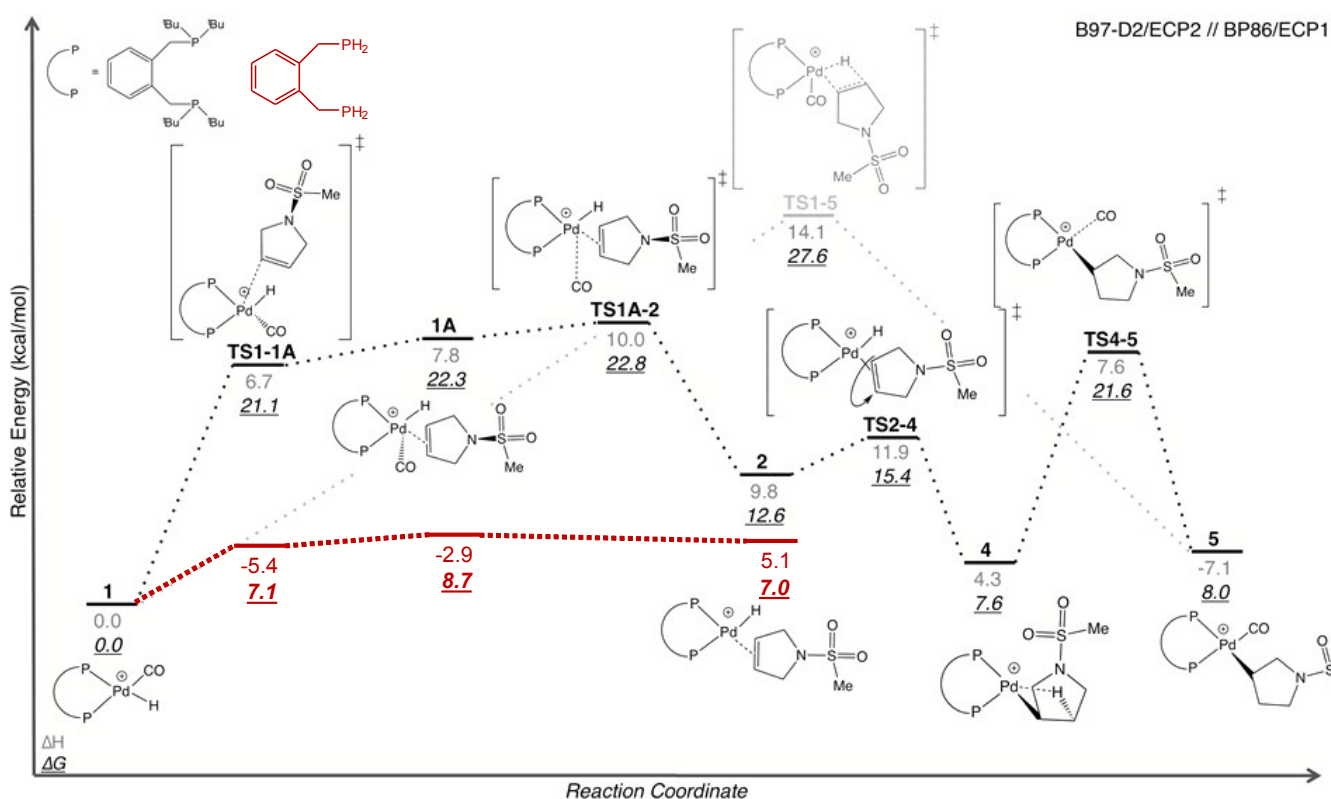
Scheme 2: Routes leading to alkylpalladium species 4 and 5 from CO coordinated resting state 1 . Ms-3-Py may approach the transition metal centre with the methylsulfonyl moiety orientated towards the hydride or away. Both routes were tested and only the most stable, the sulfonyl unit orientated away from the complex, is presented throughout. Energies in kcal/mol and relative to 1 (in dark red: analogs with the much less bulky parent phosphine (PH 2 -substituted) model).
