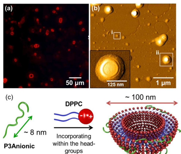
Figure 3. (a) Epi-fluorescence images of DPPC multilamellar vesicles (MLV) ( 2.6 \times 10^{-5} M) titrated with P3Anionic ( 1.3 \times 10^{-5} M (r.u.)), \lambda_{\text{ex}} = 435 nm. (b) AFM tapping mode images of P3Anionic - DPPC at 1:1 charge ratio ( 2.0 \times 10^{-5} M): (i) undoped DPPC vesicle, (ii) P3Anionic -doped vesicle. Inset: Superfine image of doped vesicle structure. (c) Schematic representation of the proposed self-assembly mechanism of P3Anionic with zwitterionic DPPC vesicles.
