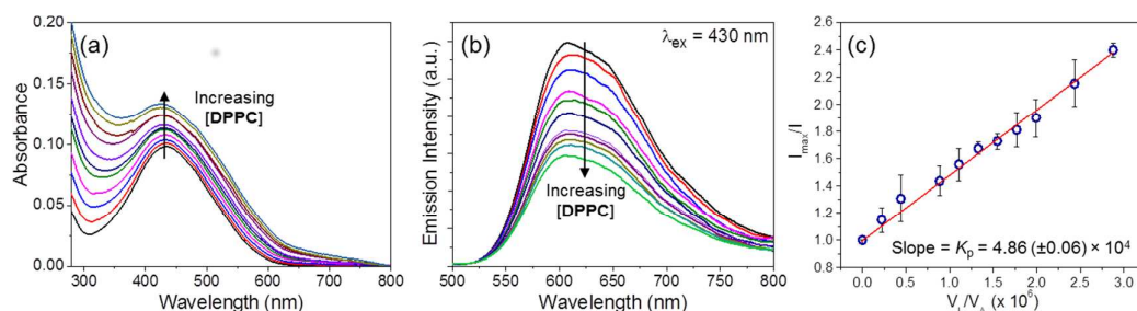
Figure 2. (a) UV/Vis absorption and (b) fluorescence spectra of P3Anionic ( 1.93 \times 10^{-5} M (r.u.)) titrated with DPPC vesicles ( 0-4.08 \times 10^{-5} M) in pH 7.3 HEPES buffer (30 mM NaCl). (c) Plot of I_{\max}/I vs. lipid volume fraction to determine the partition coefficient, K_p .
