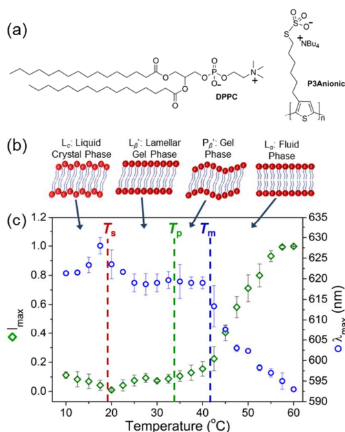
Figure 1. (a) Chemical structures of the phospholipid, DPPC , and the polythiophene, P3Anionic . (b) Schematic representations of the expected structure of the bilayer phases at different temperatures. (c) Temperature dependence of the maximum emission intensity (green diamonds) and the emission maximum, \lambda_{\text{max}} (blue circles) of P3Anionic-DPPC at 2.0 \times 10^{-5} M (r.u.). The dashed lines indicate the sub- ( T_s ), pre- ( T_p ) and main transition temperature ( T_m ).
