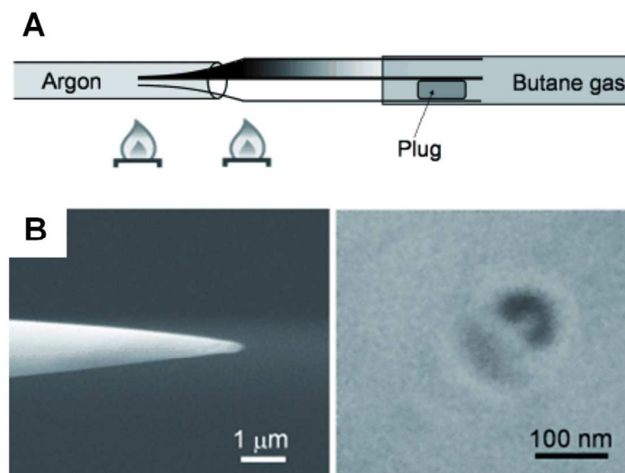
Fig. 3 A) Schematic illustration of the fabrication of a double-barrel carbon nanoprobe (DBCNP) using CVD method. A quartz theta capillary was pulled and one barrel was blocked while carbon deposition inside another barrel. B) Field emission scanning electron microscopy (FESEM) images of the side (left) and the top (right) of the DBCNP. Adapted with permission from Takahashi et al. 40 Copyright 2011 WILEY-VCH Verlag GmbH & Co. KGaA, Weinheim.
