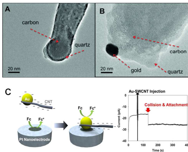
Fig. 8 (A) TEM image of a pulled quartz nanopipette filled with carbon. B) TEM image of a 20 nm AuNP attached to a carbon nanoelectrode tip. A) and B) are adapted with permission from Yu et al. 109 Copyright 2015 WILEY-VCH Verlag GmbH & Co. KGaA, Weinheim. C) Schematic illustration of the collision of a carbon nanotube (CNT)-modified Au NP at a Pt nanoelectrode (left). Upon CNT-modified Au NP attachment, an increase in current could be observed in the amperometric curve due to the increase in electrode area (right). C) and D) are adapted with permission from Park et al. 114 Copyright 2013 American Chemical Society.
