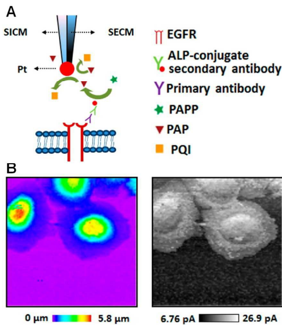
Fig. 6 A) Schematic illustration for the electrochemically sensitive high-resolution imaging of EGFR proteins using a double barrel SECM-SICM probe with deposited Pt. B) Topographic (left) and electrochemical (right) images of A431 cells obtained using Pt deposited probes. The scanned area is 75 × 75 μm. Adapted with permission from Sen et al. 80 Copyright 2015 American Chemical Society.
