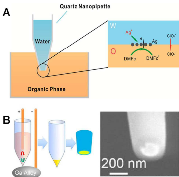
Fig. 5 A) Schematic illustration of the formation and self-assembly of Ag NPs at the liquid/liquid interface at the nanopipette tip. A disk-shape nanoelectrode could be produced. Adapted with permission from Zhu et al. 47 Copyright 2014 American Chemical Society. B) Nanopipette-based electroplated nanoelectrodes. Left: Schematic illustration for fabricating nanopipette-based electroplated nanoelectrodes. A quartz nanopipette tip was immersed in a liquid gallium/indium alloy electrode to electrochemically deposit metal inside the pipette. FIB milling was then used to expose the metal. Right: SEM image of a RG 2 gold nanoelectrode prepared using this method. Adapted with permission from Hao et al. 48 Copyright 2016 American Chemical Society.
