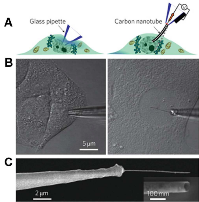
Fig. 2 A) Schematic representation of a conventional glass pipette (left) and a nanotube endoscope (right) for intracellular probing. The nanotube endoscope could penetrate the membrane of a cell without greatly disrupting the cell. B) A 1 µm glass pipette in a HeLa cell (left) and a 100 nm nanotube endoscope interrogating a primary rat hepatocyte nucleus. C) SEM image of a nanotube endoscope with a 100 nm tip. The inset shows that the end of the nanotube remain open for fluid transfer. Adapted with permission from Singhal et al. 26 Copyright 2010 Nature Publishing Group.
