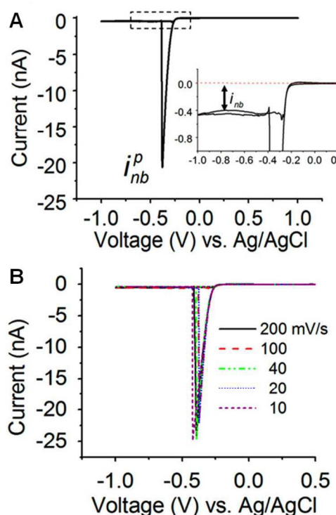
Fig. 9 A) Cyclic voltammogram of a 27-nm-radius Pt electrode in a 0.5 M H_2SO_4 solution at a scan rate of 100 mV/s. As the potential is scanned cathodically, the current firstly increased due to proton reduction and then suddenly dropped at \sim -0.4 V due to the nucleation and quick growth of a hydrogen bubble at the
