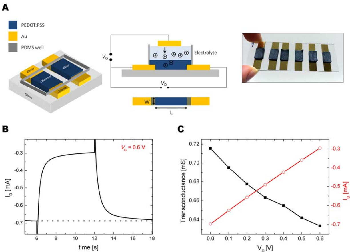
Figure 2. A) 3D, cross sectional, and top view schematics of the OEFT structure where W = 6 mm and L = 6 mm (figure not to scale). The conductivity of the PEDOT:PSS scaffold interfacing the source and drain electrodes decreases by the injection of cations from the electrolyte, triggered by an applied bias through the second scaffold which acts as the gate electrode. B) Transient characteristics of a transistor ( W = 6 mm, L = 6 mm, d = 2 mm) prepared from a porous scaffold. The length of the pulse at the gate electrode ( V_G = 0.6 V) was 6 s. V_D was constant at -0.6 V. C) Transfer characteristics of an OEFT comprised of a porous scaffold, and corresponding transconductance values at V_D = -0.6 V.
