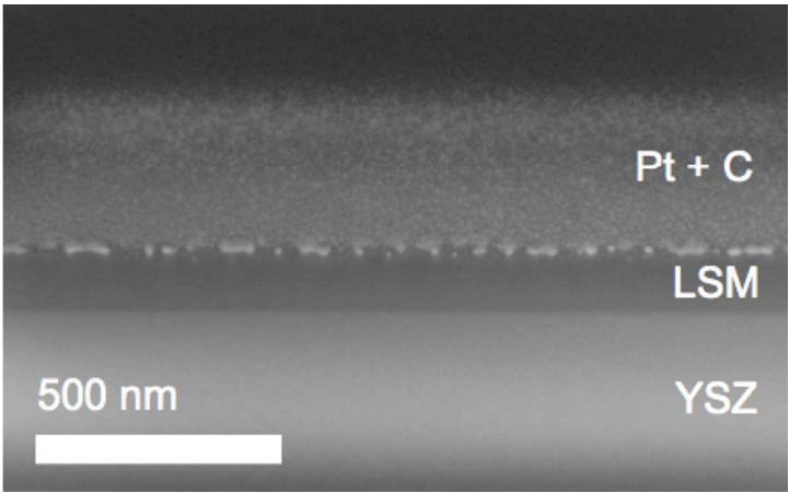
Figure 4. FIB-SEM cross-section acquired from Library 2 after impedance measurements. The sample was coated with conductive and protective layers of carbon and platinum prior to FIB milling to facilitate imaging. The top surface is tilted 52° away from the viewer.
