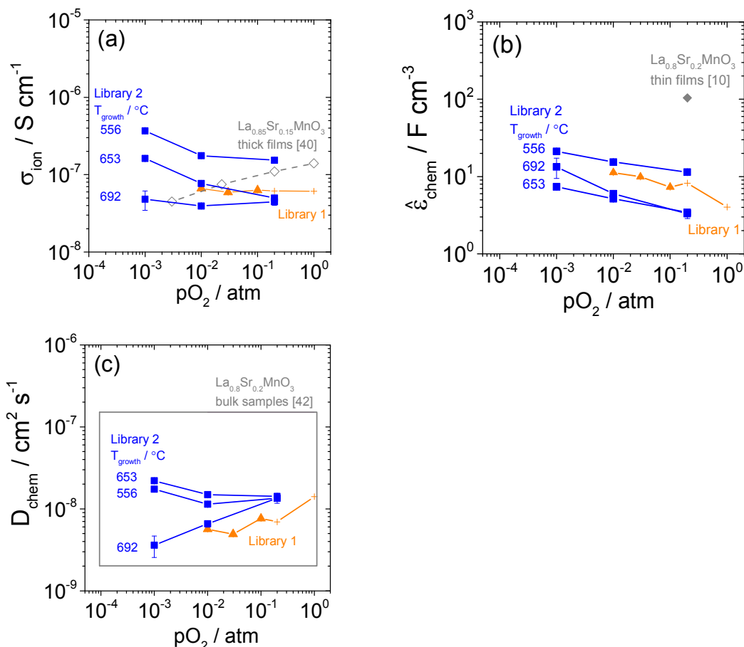
Figure 18. Through-film ionic conductivity \sigma_{ion} (a), volume-normalized chemical capacitance \hat{\epsilon}_{chem} (b), and ambipolar diffusivity D_{chem} (c) of (La_{0.8}Sr_{0.2})_{0.95}MnO_{3+\delta} obtained from 200 \mu m diameter microelectrodes at \sim 710^\circ C . 95% confidence intervals are shown except where smaller than the markers. For Library 1, negligible thickness dependence was observed, and the data shown are an average over the eighteen measured film thicknesses. The data at 0.2 and 1 bar are shown with different markers because the values of R_{ion} were fixed in the impedance fits at those conditions. For Library 2, data at three growth temperatures are shown. Comparable literature data are shown in (a) for La_{0.85}Sr_{0.15}MnO_{3+\delta} thick films, 40 (b) for La_{0.8}Sr_{0.2}MnO_{3+\delta} thin films, 10 and in (c) for La_{0.8}Sr_{0.2}MnO_{3+\delta} bulk samples as a box that bounds the range of values reported. 42
