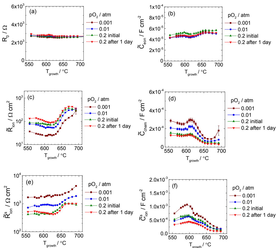
Figure 16. Growth temperature dependence of six parameters obtained from fits to impedance spectra acquired from 200 \mu\text{m} diameter microelectrodes in Library 2 under various oxygen partial pressures as indicated ( T \sim 710 ^\circ\text{C} ): (a) offset resistance; (b) interfacial electronic capacitance; (c) bulk ionic resistance; (d) bulk chemical capacitance; (e) surface reaction resistance; and (f) surface ionic capacitance. 95% confidence intervals from the impedance analysis are shown, except where they are smaller than the data points. Lines connect the points as guides for the eye.
