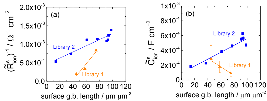
Figure 17. Dependence of surface electrochemical parameters on surface-terminated grain boundary length as measured from 200 \mu\text{m} diameter microelectrodes in Libraries 1 and 2 (varied thickness for Library 1 and varied growth temperature for Library 2) under 0.01 bar \text{O}_2 ( T \sim 710^\circ\text{C} ). (a) Electrochemical activity, defined as the inverse of the area-specific surface reaction resistance, and (b) area-normalized surface ionic capacitance.
