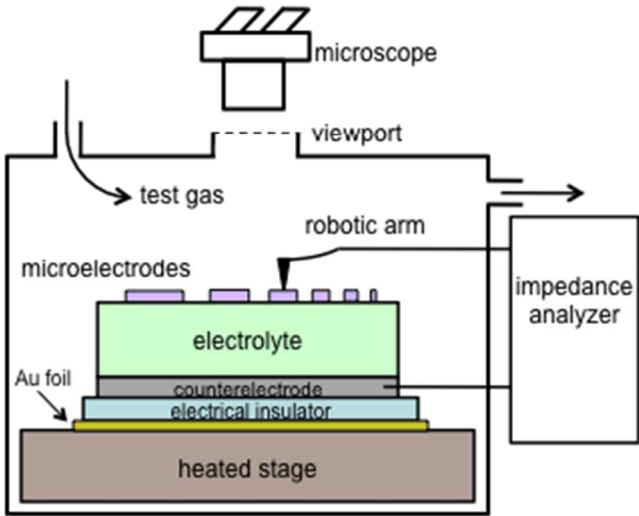
Figure 1. Schematic of the measurement configuration in the automated impedance microprobe. Dimensions are not to scale.
