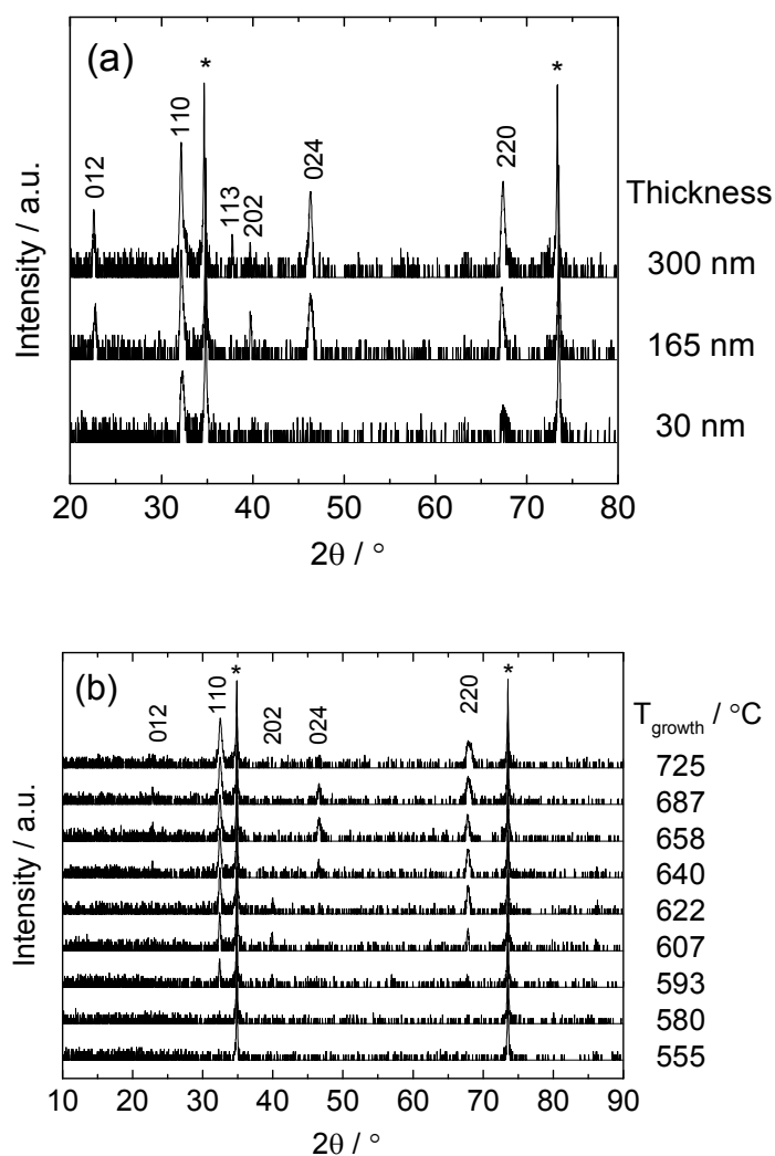
Figure 3. X-ray diffraction patterns acquired from various regions of (a) Library 1, and (b) Library 2 (see Table 1 for library details). The Miller indices of each LSM reflection are indicated. Reflections marked with an asterisk are from the YSZ substrate.
