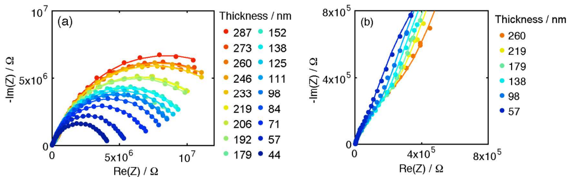
Figure 13. Thickness dependence of impedance spectra of 200 μm diameter microdot electrodes from Library 1 under 0.01 bar O 2 ( T \sim 710 C). (a-b) Nyquist plots at two different scales. Curves are fits to the data according to Equation 1.
