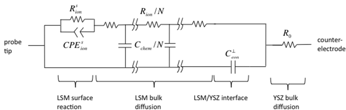
Figure 9. Equivalent circuit corresponding to the reaction pathway shown in Figure 8. The subset of the circuit between the break symbols is repeated N times, where N approaches \infty .
