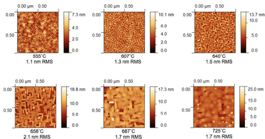
Figure 6. Atomic force micrographs of selected microelectrodes from Library 2 acquired after patterning. The corresponding growth temperature and root-mean-squared roughness values are listed below each image.
