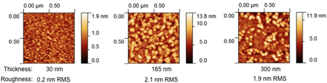
Figure 5. Atomic force micrographs of selected microelectrodes from Library 1 acquired after patterning. The corresponding thickness and root-mean-squared roughness values are listed below each image.
