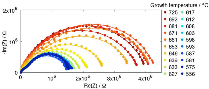
Figure 15. Growth temperature dependence of impedance spectra from 200 \mu\text{m} diameter microelectrodes in Library 2 under 0.01 bar \text{O}_2 ( T \sim 710\text{ C} ), shown in the Nyquist representation. Points are raw data, curves are fits according to Equation 1.
