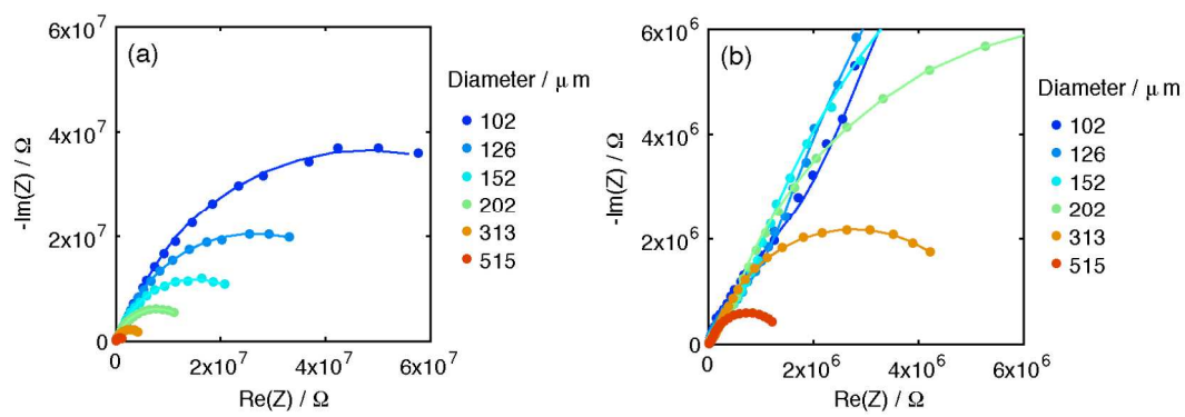
Figure 11. Diameter dependence of impedance spectra of 246 nm thick microelectrodes of Library 1 under 0.01 bar \text{O}_2 ( T \sim 710 \text{ C} ). (a-b) Nyquist plots at two different scales. Curves are fits to the data according to Equation 1.
