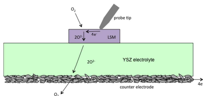
Figure 8. Schematic of the proposed through-film reaction pathway.
