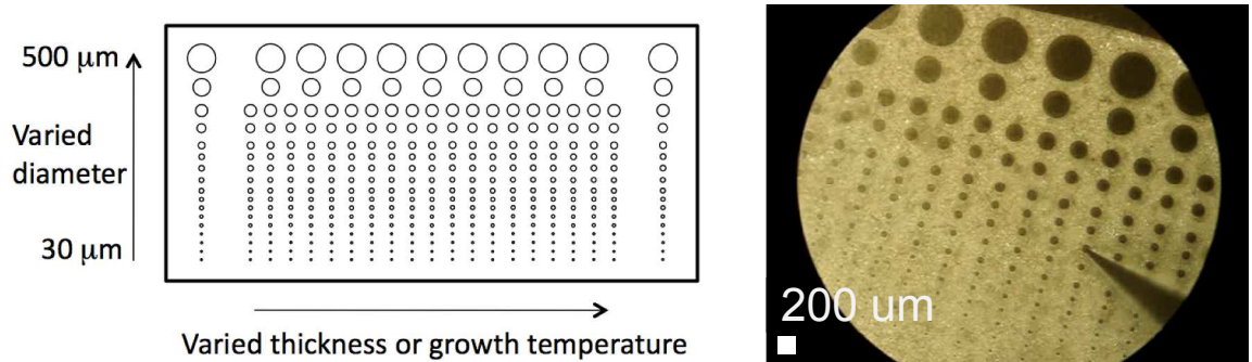
Figure 2. Layout of a library of (\text{La}_{0.8}\text{Sr}_{0.2})_{0.95}\text{MnO}_{3+\delta} thin film microelectrodes grown on a 5 \times 10 mm substrate. Left: Schematic. Right: Optical microscope image of Library 1 during impedance testing.
