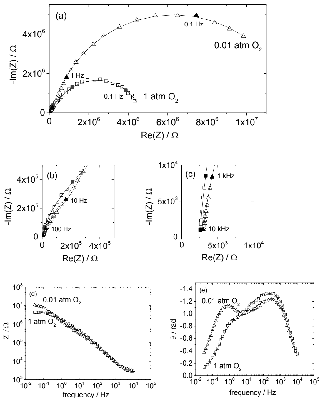
Figure 10. Representative impedance spectra acquired from (\text{La}_{0.8}\text{Sr}_{0.2})_{0.95}\text{MnO}_{3+\delta} microelectrodes (Library 1, 200 \mu\text{m} diameter, 192 \text{ nm} thickness, T \sim 710^\circ\text{C} ) under 1 \text{ bar O}_2 (square markers) or 0.01 \text{ bar O}_2 (triangles): (a-c) Nyquist plots at various scales, (d) magnitude plot, and (e) phase plot. Curves are fits to the data according to Equation 1.
