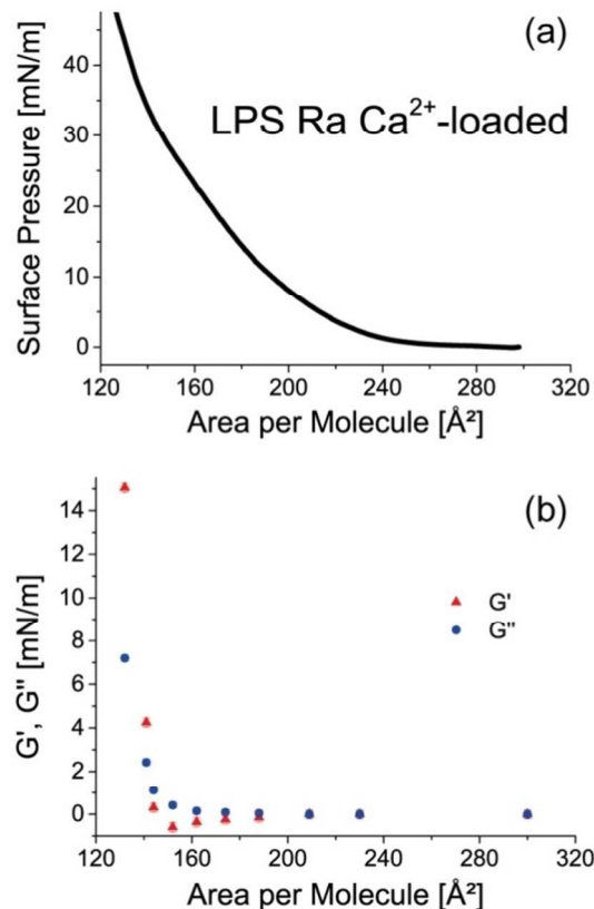
Fig 4 (a) Pressure-area isotherm of LPS Ra monolayer on \text{Ca}^{2+} -loaded subphase at 12 h. (b) Viscous and elastic modulus of LPS Ra monolayers on \text{Ca}^{2+} -loaded subphase. Error bars are comparable to the symbol size and therefore not visible.
