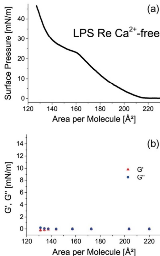
Fig 1 (a) Pressure-area isotherm of LPS Re monolayer on \text{Ca}^{2+} -free subphase. (b) Viscous and elastic modulus of LPS Re monolayer on \text{Ca}^{2+} -free subphase. Error bars are comparable to the symbol size and therefore not visible.
