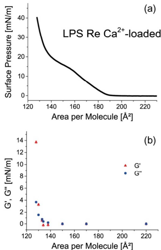
Fig 2 (a) Pressure-area isotherm of LPS Re monolayer on \text{Ca}^{2+} -loaded subphase. (b) Viscous and elastic modulus of LPS Re monolayer on \text{Ca}^{2+} -loaded subphase. Error bars are comparable to the symbol size and therefore not visible.
