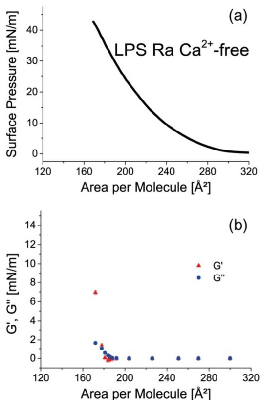
Fig 3 (a) Pressure-area isotherm of LPS Ra monolayer on \text{Ca}^{2+} -free subphase at 12 h. (b) Viscous and elastic modulus of LPS Ra monolayers on \text{Ca}^{2+} -free subphase. Error bars are comparable to the symbol size and therefore not visible.
