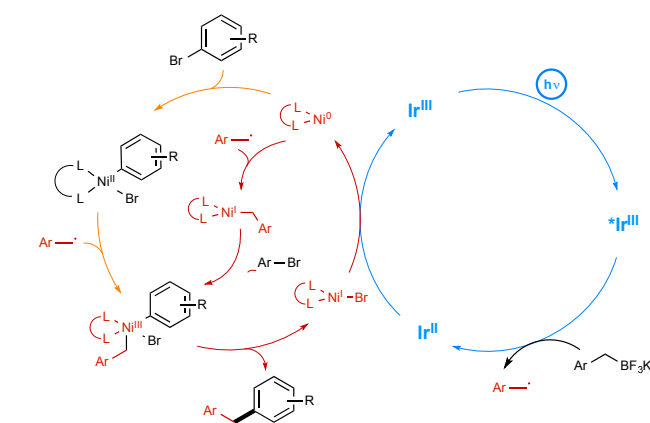
Scheme 12. Hypothetical mechanism of the photoredox/nickel cross-coupling
