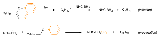
Scheme 15. Barton-type decarboxylative experiment with dipp-lmd-BH 3 as a hydrogen donor
