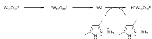
Scheme 16. Visible-light-mediated formation of 3,5-dimethylpyrazole-boryl radical
