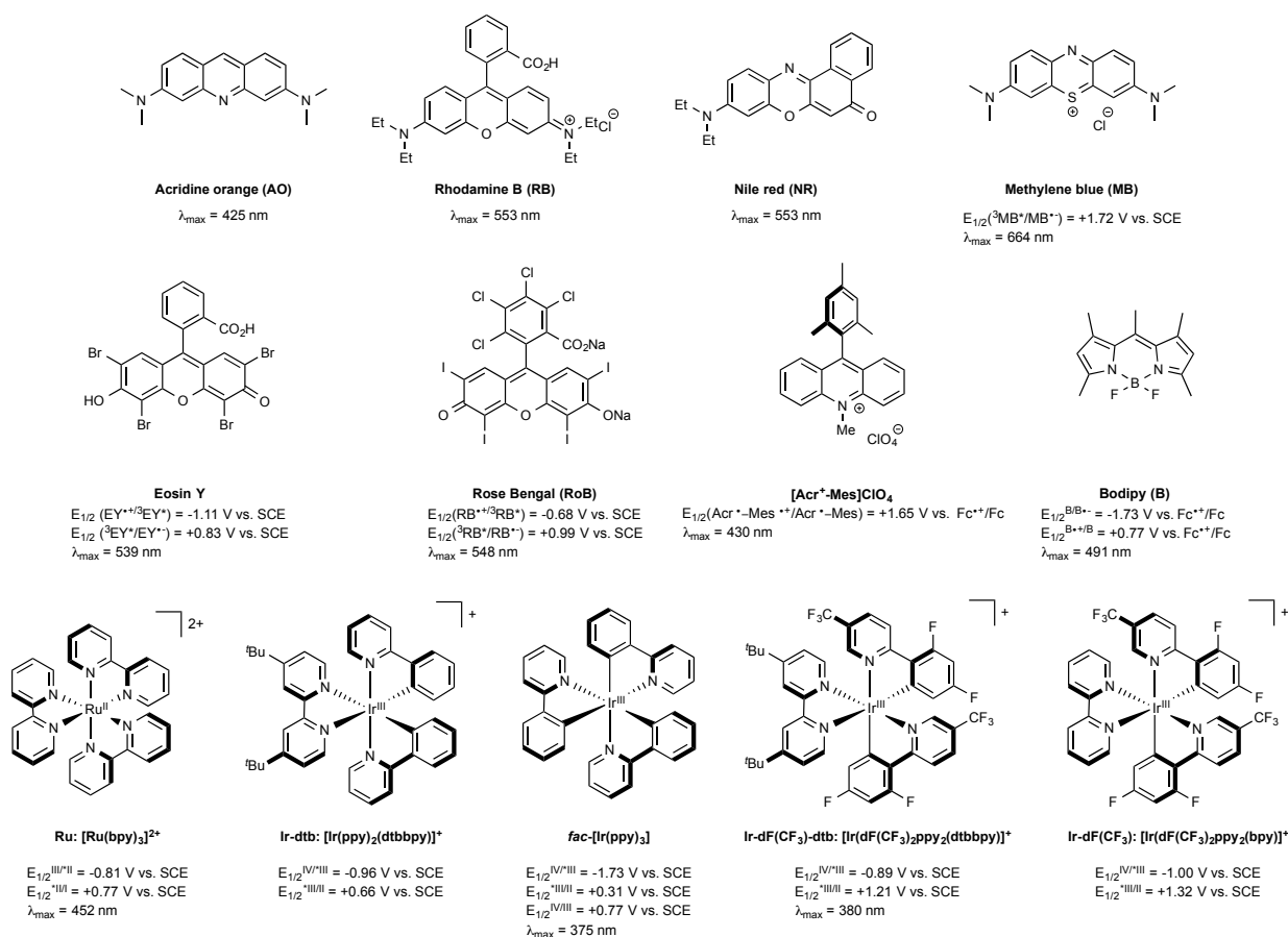
Figure 1. Selected examples of catalysts used in visible-light photoredox chemistry and their excited-state potentials.
