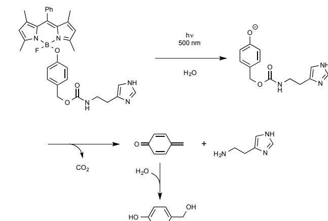
Scheme 27. Uncaging reaction of BODIPY-caged histamine derivative
