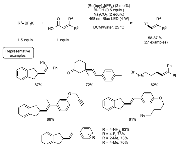
Scheme 10. Deboronative/decarboxylative alkenylation reaction
