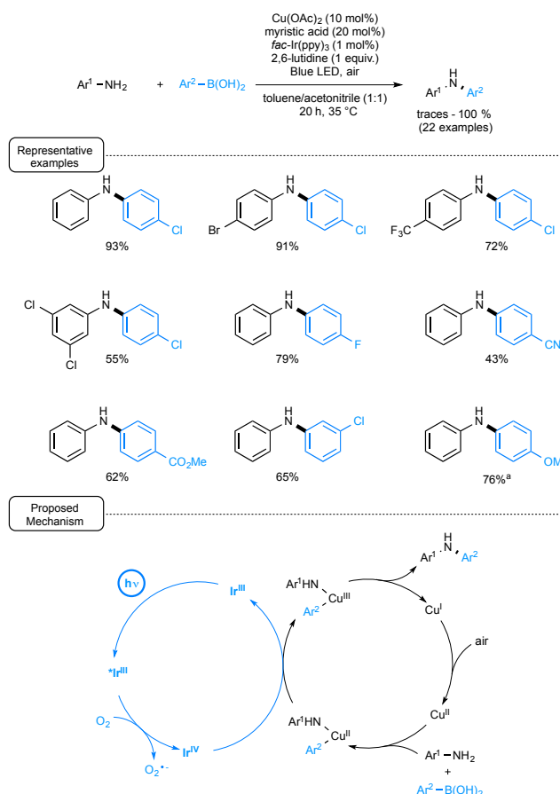
Scheme 29 Cu/Ru-Catalyzed trifluoromethylation of boronic acids and plausible mechanism
