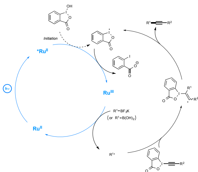
Scheme 9. Mechanistic pathway of the deboronative alkynylation
