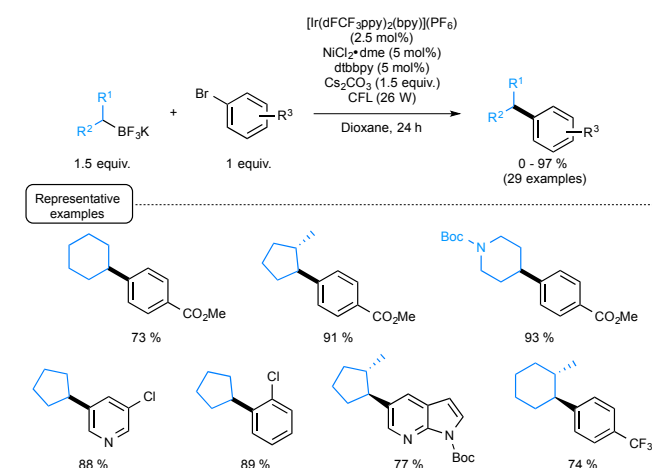
Scheme 14. Photoredox cross-coupling of secondary alkyl trifluoroborates and aryl bromides
