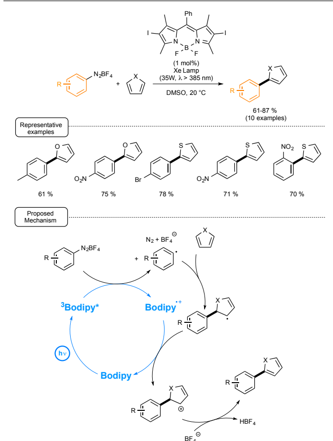
Scheme 25. BODIPY-photocatalyzed arylation of furan and thiophene and proposed mechanistic pathway
