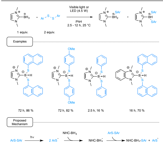
Scheme 18. First synthesis of NHC-boryl sulfides and proposed mechanistic pathway
