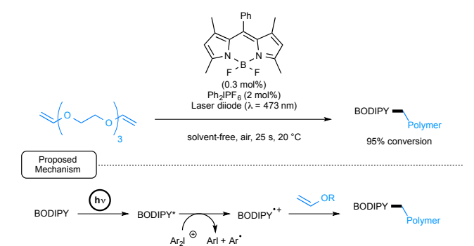
Scheme 26. BODIPY-mediated photopolymerization of divinylether monomer and proposed mechanism
