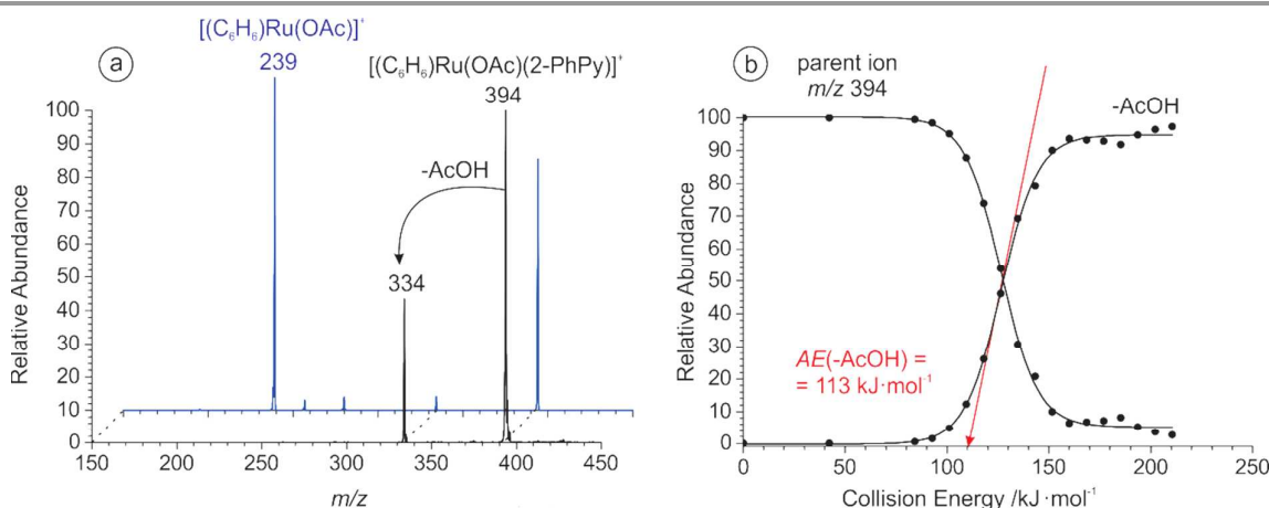
Fig. 1. a) CID spectra of the mass selected peak at m/z 394 for 2-PhPy (black) and 3-PhPy (blue); b) the breakdown curve for m/z 394 (2-PhPy). The appearance energy for acetic acid loss was determined to be AE(-AcOH) = 113 \pm 3 \text{ kJ} \cdot \text{mol}^{-1} .
