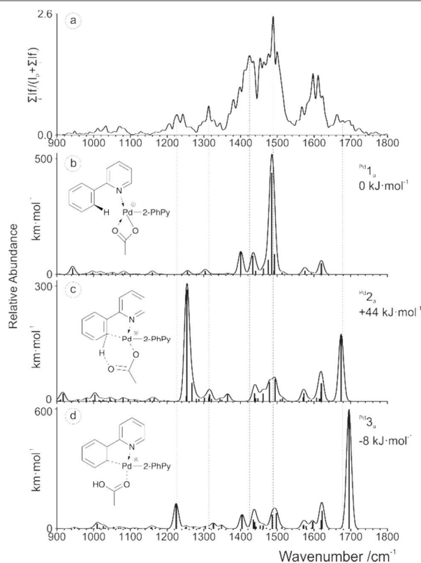
Fig. 4. a) IRMPD spectrum of the mass-selected [(2\text{-PhPy})_2\text{Pd}(\text{OAc})]^+ complex and theoretical IR spectra of b) \text{Pd}1_a , c) \text{Pd}2_a and d) \text{Pd}3_a . The line spectra are presented along with a Gaussian function with \text{fwhm} = 16 \text{ cm}^{-1} . Corresponding calculated structures can be seen in Fig. S12 of the Supporting Information.
