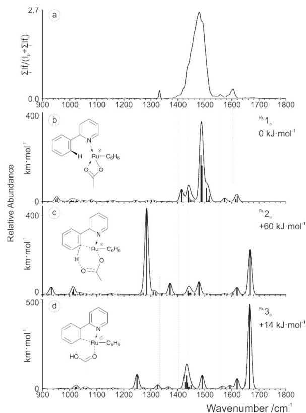
Fig. 3. a) IRMPD spectrum of the mass-selected [(2\text{-PhPy})\text{Ru}(\text{C}_6\text{H}_6)(\text{OAc})]^+ complex and theoretical IR spectra of b) \text{Ru}1_a , c) \text{Ru}2_a and d) \text{Ru}3_a . The line spectra are presented along with a Gaussian function with \text{fwhm} = 16 \text{ cm}^{-1} . Corresponding calculated structures can be seen in Fig. S10 of the Supporting Information.
