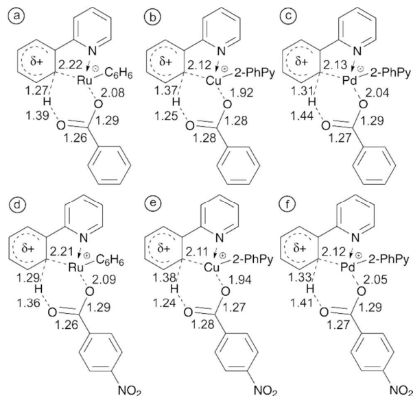
Fig. 6. 6-membered transition structures showing key bond lengths for a) RuTS 2a-3a , b) CuTS 1a-3a and c) PdTS 2a-3a with a benzoate counter ion and d) RuTS 2a-3a , e) CuTS 1a-3a , and f) PdTS 2a-3a with a 4-nitrobenzoate counter ion. All distances are in Å.
