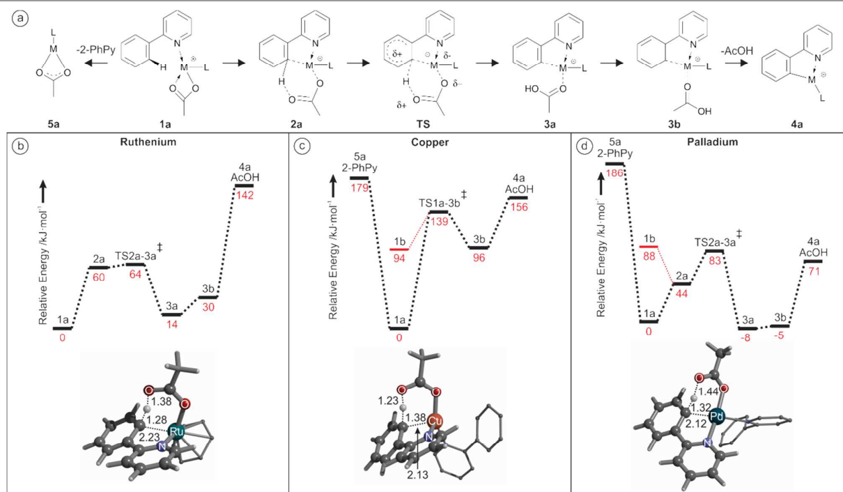
Fig. 2. a) structural representations of the different calculated species involved in the C-H activation reactions (structure 1b the monodentate isomer, was omitted for clarity); b) potential energy surface (B3LYP/cc-pVTZ:cc-pVTZ-pp(Ru)) for the Ru assisted C-H activation of 2-PhPy.; c) potential energy surface (B3LYP/cc-pVTZ:cc-pVTZ-pp(Cu)) for the Cu assisted C-H activation of 2-PhPy.; d) potential energy surface (B3LYP/cc-pVTZ:cc-pVTZ-pp(Pd)) for the Pd assisted C-H activation of 2-PhPy. All energies are at 0 K and the depicted structures represent the transition structures; distances are in Å.
