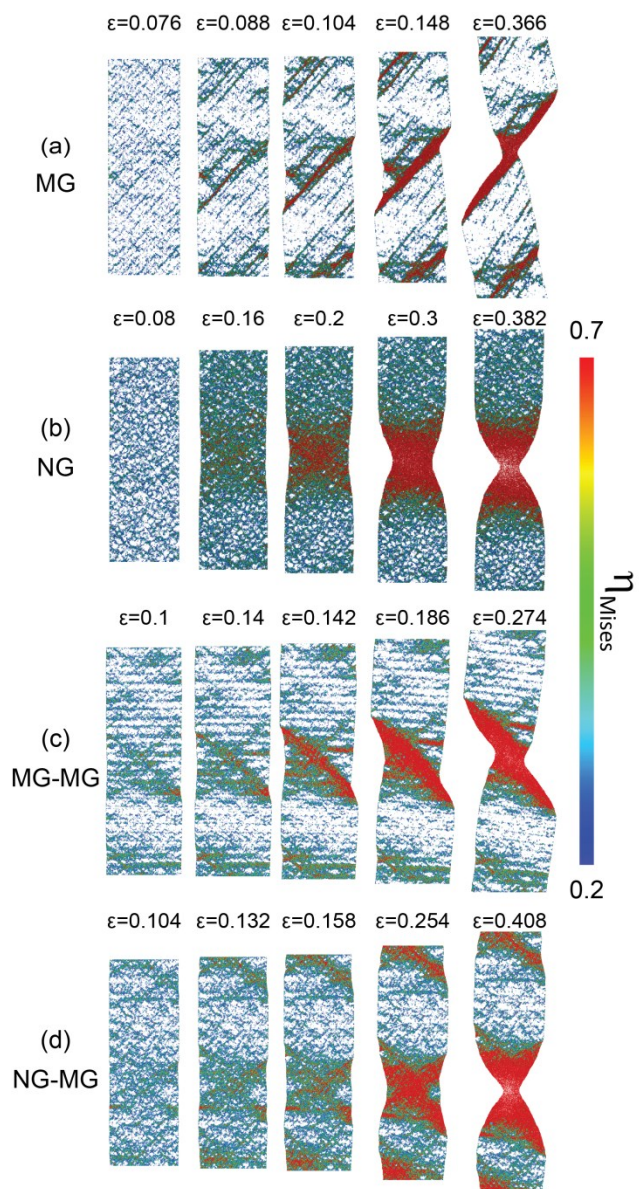
Fig. 3 Illustrations of the deformation and failure of (a) MG, (b) NG, (c) nanolaminate MG, and (d) nanolaminate NG-MG nanopyllars. The color indicates the von Mises local atomic shear strain, \eta_{\text{Mises}} . For clarity, only atoms with \eta_{\text{Mises}} > 0.2 are shown. Illustrations are produced from visualizations of a 1 nm thick slice along the nanopyllars cutting their cross section.
