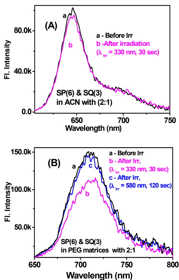
Figure 4: Fluorescence switching behaviour of the mixture of SP(6) and SQ(3) in 2:1 ratio upon alternate application of UV and Vis/ \Delta in ACN solution and in PEG polymer matrices at room temperature. (A) in ACN at 300K, (B) in PEG polymer matrices at 300K.
