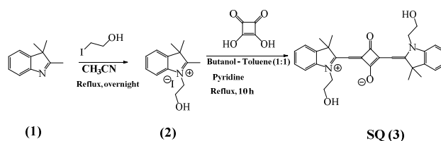
Scheme 1: Synthetic route of the Squaraine SQ ( 3 ) dye.
