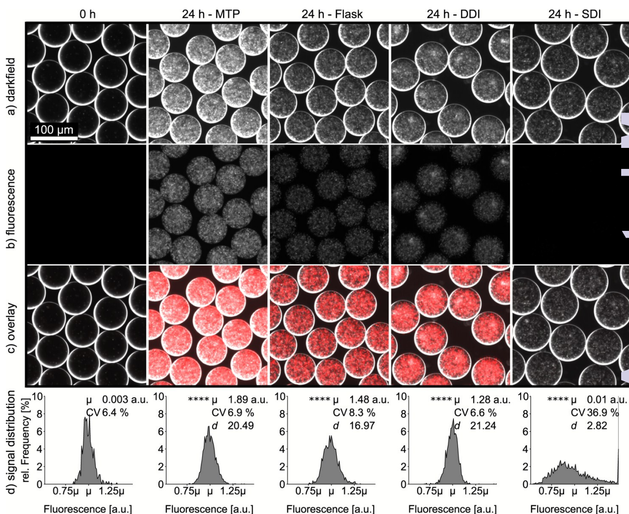
Fig. 6. mCherry fluorescence intensity of droplets either re-injected after 24 h of DDI and SDI or generated from 24 h MTP and shaking flask cultures. Images were recorded in darkfield (a) and fluorescence mode (b) at 10x magnification. The fluorescence images were enhanced in brightness and false colored for the overlay (c). Frequency distributions of fluorescence intensity of at least 600 droplets per cultivation method (d). Means of fluorescent intensity were compared with Welch corrected ANOVA and Dunnett's test (both \alpha = 0.05 ) in combination with a heteroscedastic consistent covariance estimation, **** significant with p < 0.0001 . As a measure of effect size
