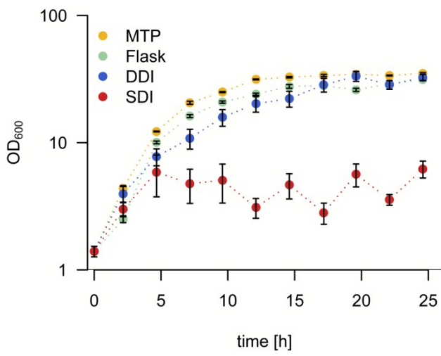
Fig. 4. E. coli growth kinetics in cultures grown in MTP, shaking flask, and in droplets with DDI and SDI. A minimum of 1800 droplets were re-injected and analyzed per time point for SDI and DDI. Gray values were transformed into absorbance values via calibration (Fig. S5 and S6). Error bars indicate one standard deviation.
