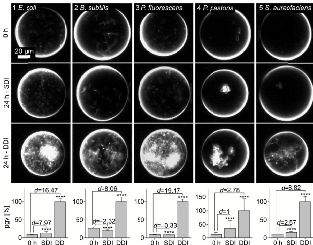
Fig. 3. Biomass yield of different microorganisms in droplets after 24 h (except S. aureofaciens – 72 h, humid chamber) of DDI and SDI. Population gray values (pgv) were compared with Welch corrected ANOVA and Dunnett's test (both \alpha = 0.05 ) in combination with a heteroscedastic consistent covariance estimation, **** significant with p < 0.0001 . Plotted pgv are standardized to the pgv of the corresponding DDI population. A minimum of 9500 single droplets were analyzed per droplet population. To indicate which effects are practically relevant, the effect size is given using Cohen's d, and 0 h control as reference.
