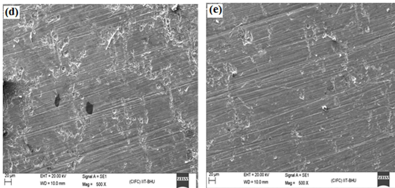
Fig.8 (a-e): SEM images of mild steel surfaces: abraded (a), in absence of AACs (b) in the presence of 40 \text{ mgL}^{-1} of AAC-1(c), AAC-2(d), and AAC-3(e)
