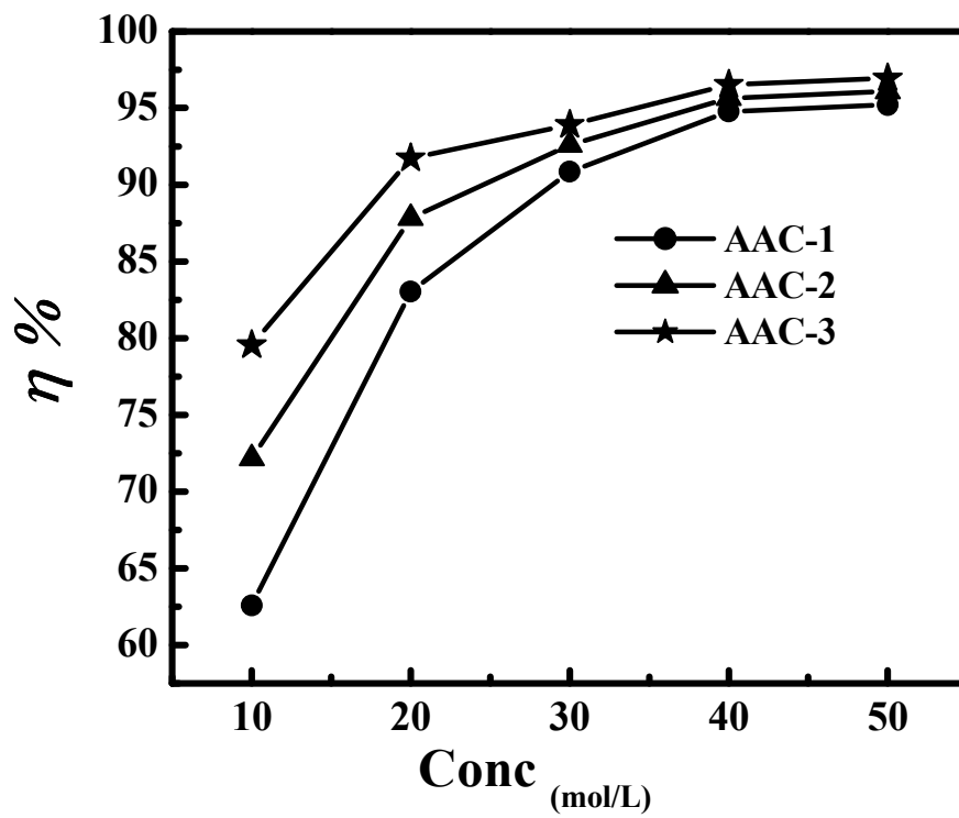
Fig.2: Variation of inhibition efficiency with AACs concentration
