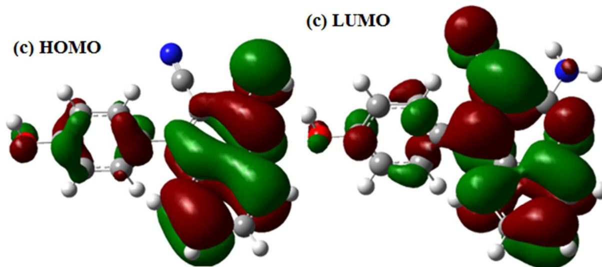
Fig. 12: The frontier molecular orbital of studied AACs (a) AAC-1 (left, HOMO; right, LUMO), (b) AAC-2 (left, HOMO; right, LUMO) and (c) AAC-3 (left, HOMO; right, LUMO)
