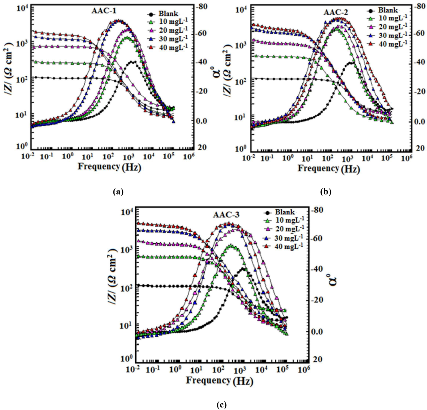
Fig. 7 a-c: Bode ( \log f vs \log |Z| ) and phase angle ( \log f vs \alpha^\circ ) plots for mild steel in 1 M HCl in absence and presence of different concentration of AACs.
