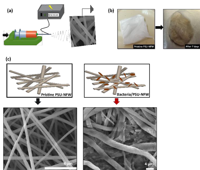
Figure 1. (a) Schematic representation of the electrospinning process for PSU-NFW. (b) Photos of attachment of free bacteria cells on PSU-NFW for seven days process. (c) SEM micrographs of pristine PSU/NFW and bacteria/PSU-NFW.
