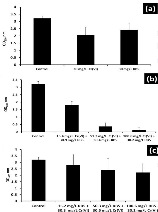
Figure 4. (a) Single and (b) binary effects of RB5 and Cr(VI) on the biomass growth of Lysinibacillus sp. NOSC (pH: 8.0; Temp: 30±1 °C; stirring rate: 100 rpm). Error bars represent the means of three independent replicates.
