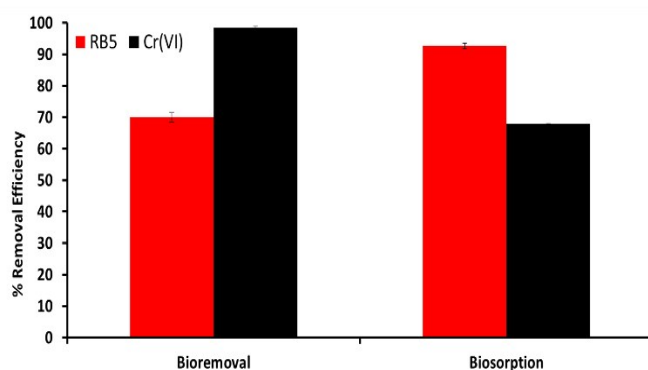
Figure 6. The comparison of bioremoval and biosorption of RB5 and Cr(VI) at 30 \text{ mg L}^{-1} initial dye and heavy metal concentrations after 24 h (pH: 8.0; Temp: 30 \pm 1^\circ \text{C} ; stirring rate: 100 rpm). Error bars represent the means of three independent replicates.
