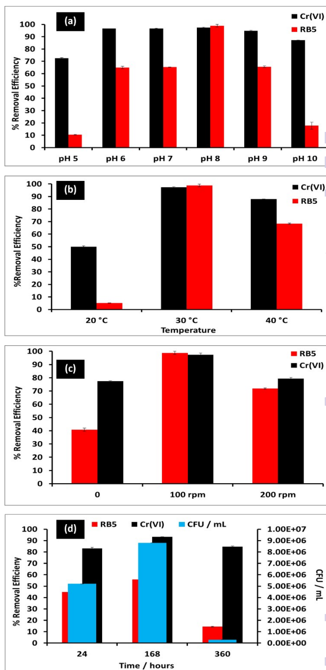
Figure 2. Effects of (a) various pH values (b) different temperatures (c) static/shaking conditions and (d) effect of bacterial counts after incubating PSU-NFW's for different time periods (24 h, 7 days and 15 days) on removal efficiency of RB5 and Cr(VI) by Lysinibacillus sp. NOSK after 24 h incubation. Error bars represent the means of three independent replicates.
