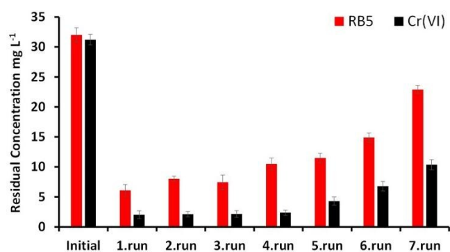
Figure 5. Reusability test results of the bacteria/PSU-NFW for 7 cycles of RB5 and Cr(VI) removal at an initial contaminants concentration of 30 \text{ mg L}^{-1} (pH: 8.0; Temp: 30 \pm 1^\circ \text{C} ; stirring rate: 100 rpm). Error bars represent the means of three independent replicates.
