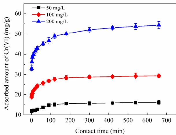
Fig. 3 Effect of contact time on Cr(VI) adsorption using CoFe 2 O 4 /MgAl-LDH for initial Cr(VI) concentrations of 50, 100 and 200 mg/L.
