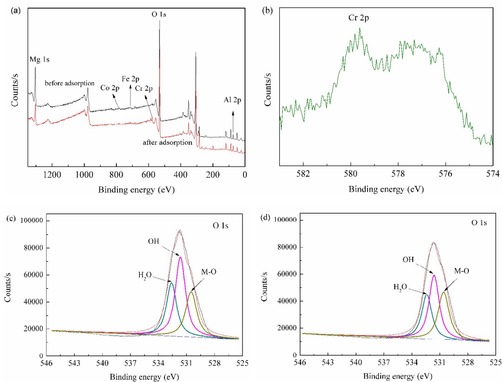
Fig. 7 Wide XPS spectra of (a) \text{CoFe}_2\text{O}_4/\text{MgAl-LDH} before and after \text{Cr(VI)} adsorption, (b) \text{Cr 2p} spectrum of \text{CoFe}_2\text{O}_4/\text{MgAl-LDH} after \text{Cr(VI)} adsorption, (c) \text{O 1s} spectrum of \text{CoFe}_2\text{O}_4/\text{MgAl-LDH} , and (d) \text{O 1s} spectrum of \text{CoFe}_2\text{O}_4/\text{MgAl-LDH} after \text{Cr(VI)} adsorption.
