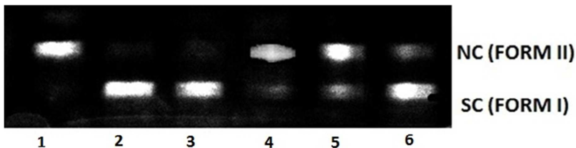
Fig. 10 Cleavage of supercoiled pUC 19 DNA ( 40 \mu\text{M} ) by complexes 1-5 in a buffer containing 5% DMF/5 mM Tris HCl/50 mM NaCl at pH = 7.2 and 37^\circ\text{C} with an incubation time of 3 h. lane 1, DNA control; lane 2, DNA + 1 ( 150 \mu\text{M} ); lane 3, DNA + 2 ( 150 \mu\text{M} ); lane 4, DNA + 3 ( 150 \mu\text{M} ); lane 5, DNA + 4 ( 150 \mu\text{M} ); lane 6, DNA + 5 ( 150 \mu\text{M} ). Forms SC and NC are supercoiled and nicked circular DNA, respectively.
