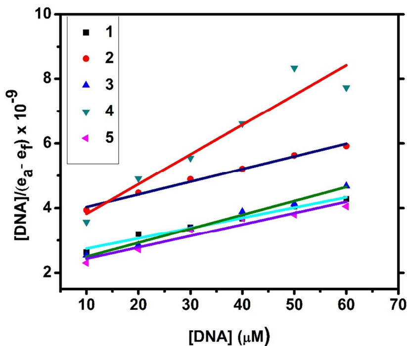
Fig. 7 Plots of [\text{DNA}]/(\epsilon_a - \epsilon_f) versus [\text{DNA}] for the titration of the complexes with CT DNA.
