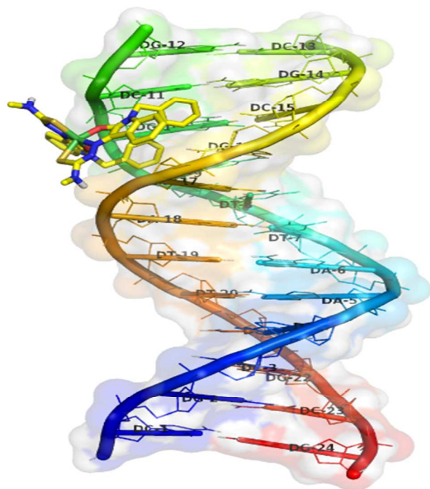
Fig. 18 Docking pose of nickel(II) complexes 2 and 4 with B-DNA (1BNA).
