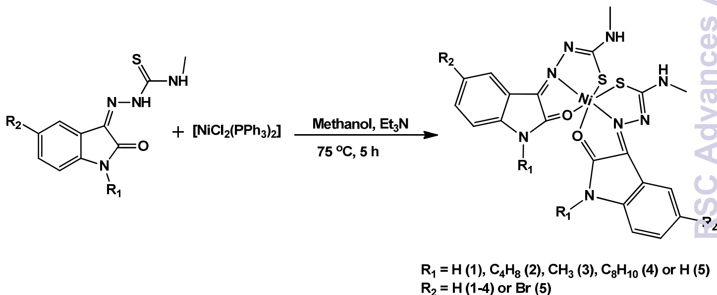
Scheme 2 Synthetic scheme of nickel(II) complexes.
