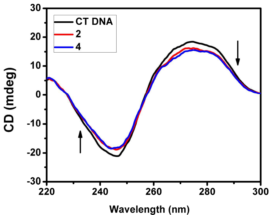
Fig. 9 CD spectra of CT DNA (200 \mu\text{M} ) in the absence and presence of 40 \mu\text{M} of complex 2 and 4.
