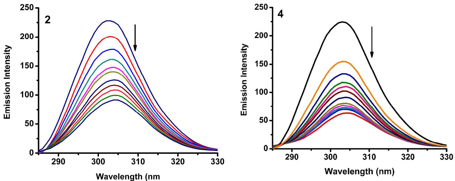
Fig. 16 Synchronous spectra of BSA (1 \mu\text{M} ) as a function of concentration of 2 and 4 (0-50 \mu\text{M} ) with \Delta\lambda = 15 nm.
