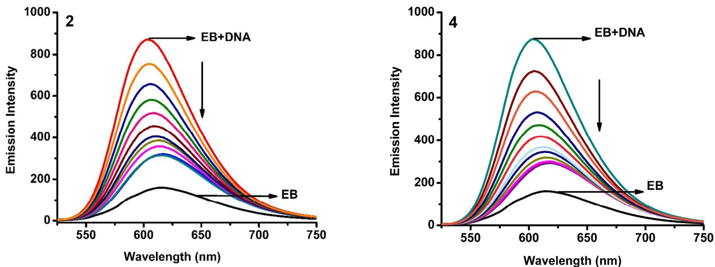
Fig. 6 Fluorescence quenching curves of EB bound to DNA in the presence of 2 and 4 . [\text{DNA}] = 5 \mu\text{M} , [\text{EB}] = 5 \mu\text{M} and [\text{complex}] = 0\text{-}50 \mu\text{M} .
