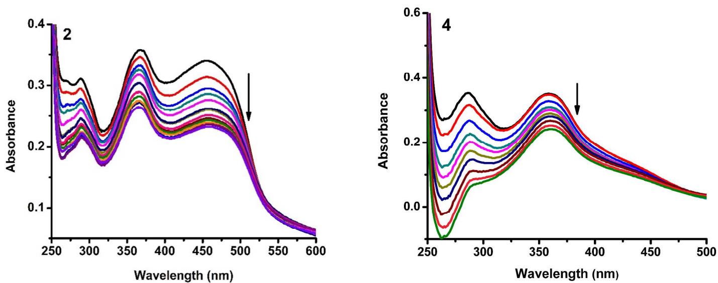
Fig. 5 Absorption spectra of complexes ( 2 and 4 ) in Tris-HCl buffer upon addition of CT DNA. [Complex] = 1.5 \times 10^{-5} M, [DNA] = 0-50 \mu M. Arrow shows that the absorption intensities decrease upon increasing DNA concentration.
