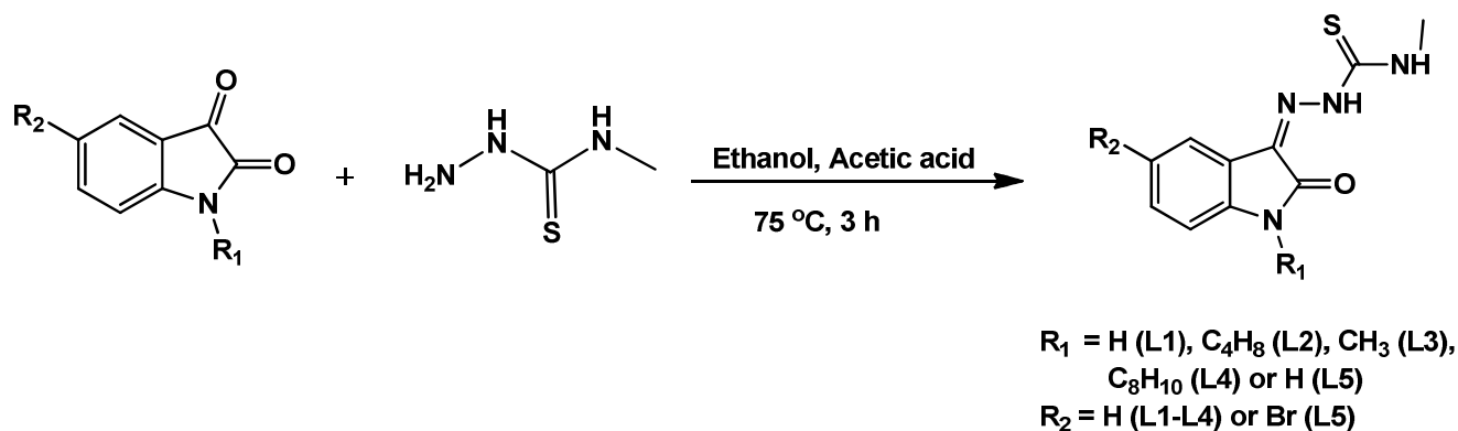
Scheme 1 Synthetic scheme of isatin thiosemicarbazone ligands.
