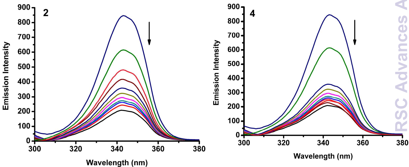
Fig. 15 Synchronous spectra of BSA (1 \mu\text{M} ) as a function of concentration of 2 and 4 (0-50 \mu\text{M} ) with \Delta\lambda = 60 nm.
