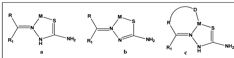
Fig. 1 Different coordination modes of thiosemicarbazone.
