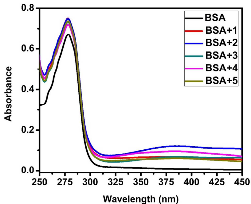
Fig. 12 The absorption spectra of BSA (10 μM) and BSA with 1-5 (4 μM).
