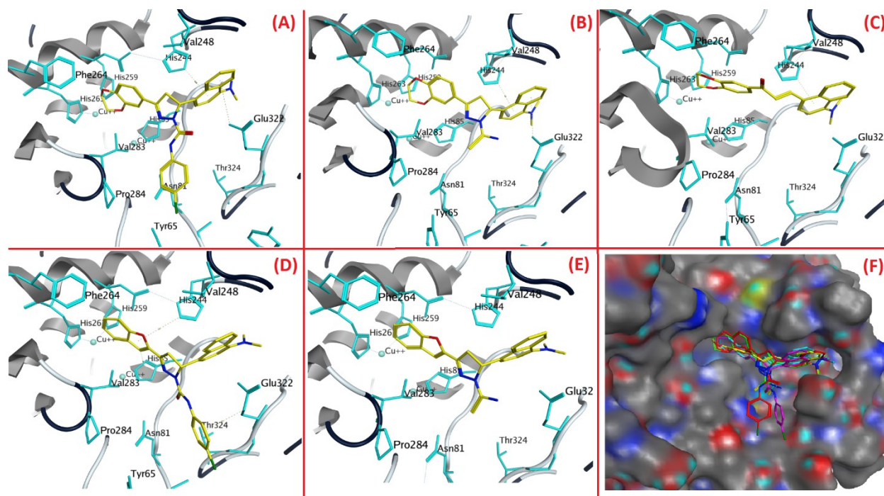
Figure 3: : The orientations of A) 4b , B) 4a , C) 4 , D) 1b and E) 1a in tyrosinase active site and F) superimposition of the best poses of compound 4b , 4a , 4 , 1b and 1a .
