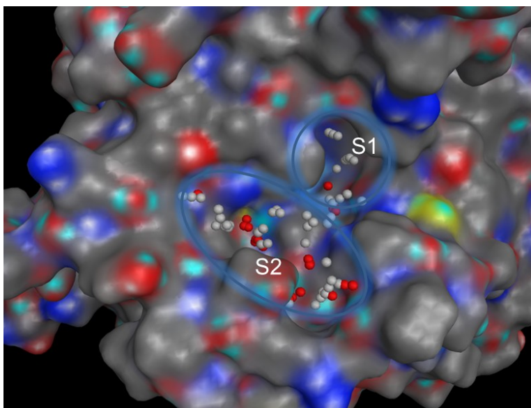
Figure 2: Binuclear copper binding site (S1) and its entrance (S2) region of mushroom tyrosinase enzyme.
