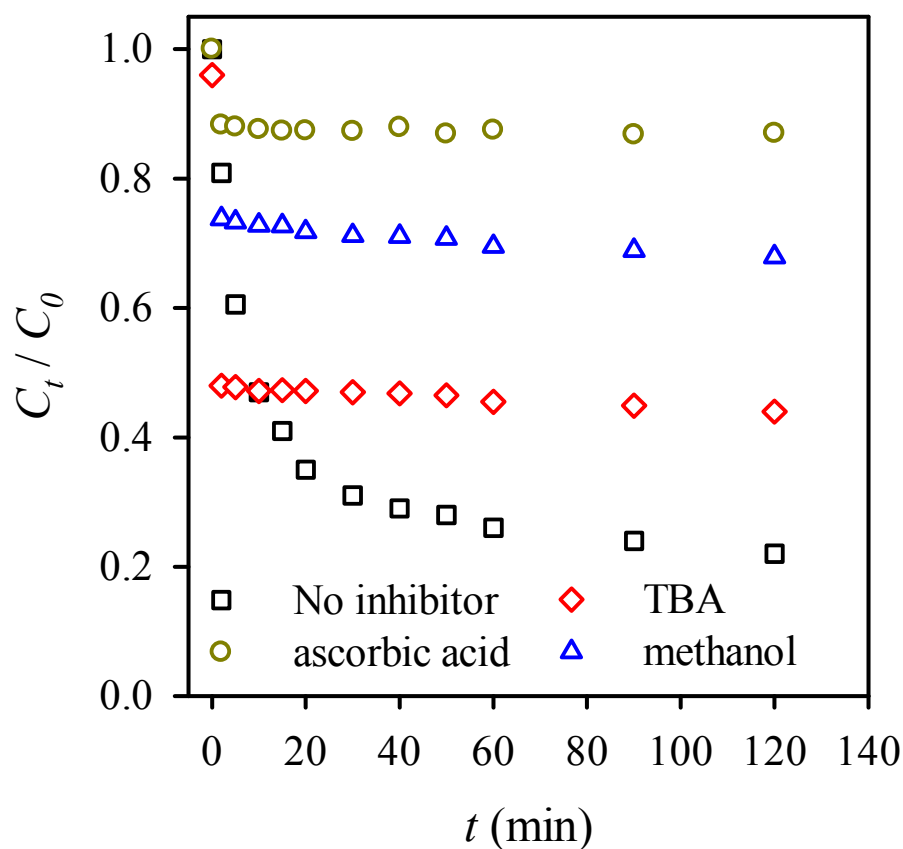
Fig. 12. Effects of inhibitors on the RB decolorization using persulfate activated by MIL-88A (Persulfate = 200 mg L -1 , MIL-88A = 500 mg L -1 , 40 °C, ascorbic acid = 280 mmol L -1 , tert -butyl alcohol (TBA) = 280 mmol L -1 , methanol = 280 mmol L -1 ).
