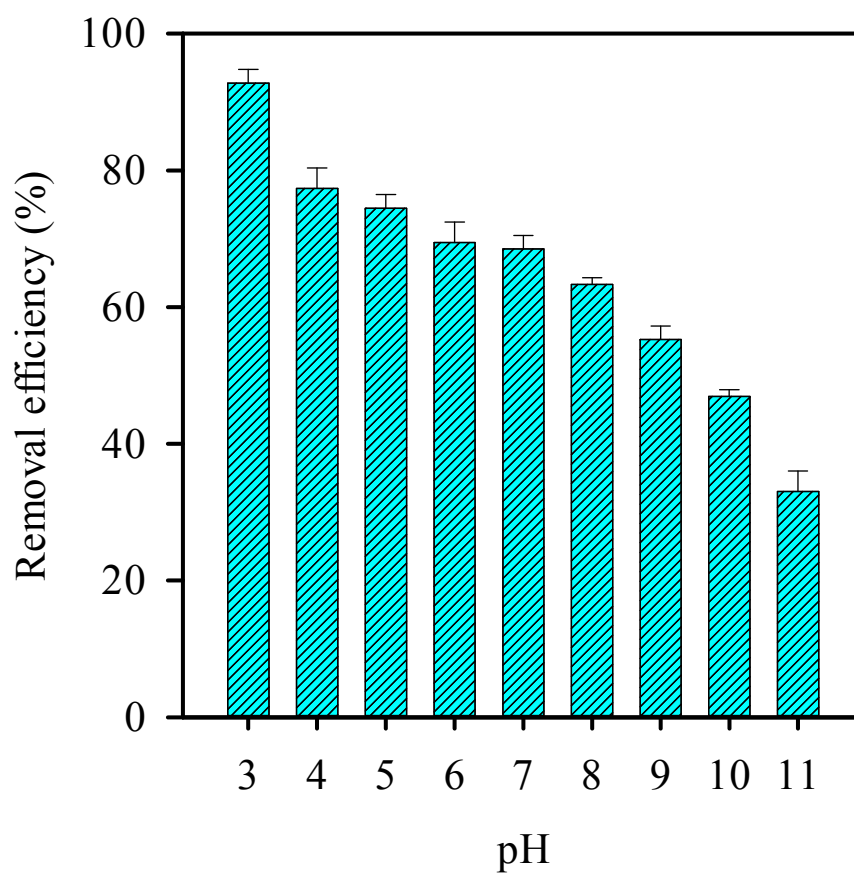
Fig. 10. Effect of pH on the RB decolorization using persulfate activated by MIL-88A (Persulfate = 200 mg L -1 , MIL-88A = 500 mg L -1 , 40 °C).
