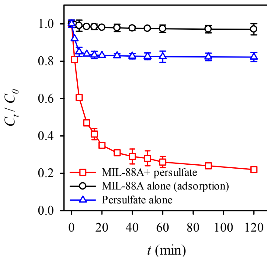
Fig. 5. RB removal by adsorption to MIL-88A, oxidation with persulfate and oxidation with persulfate activated by MIL-88A (Persulfate = 200 mg L -1 , MIL-88A = 500 mg L -1 , 40 °C).
