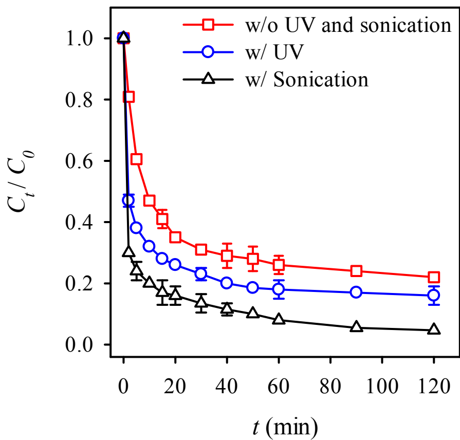
Fig. 11. Effects of UV and ultrasonication on the RB decolorization using persulfate activated by MIL-88A (Persulfate = 200 mg L -1 , MIL-88A = 500 mg L -1 , 40 °C).
