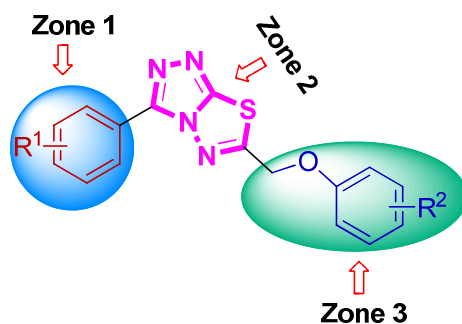
Fig. 11 The synthesized triazolothiadiazole structures ( 4a–l ) investigated herein.
