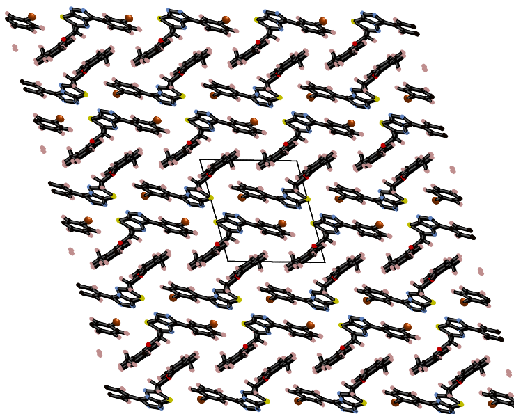
Fig. 8 Packing diagram of 4i in the yz plane stabilized by both N...S sigma-hole interactions and C-H... \pi interactions.
