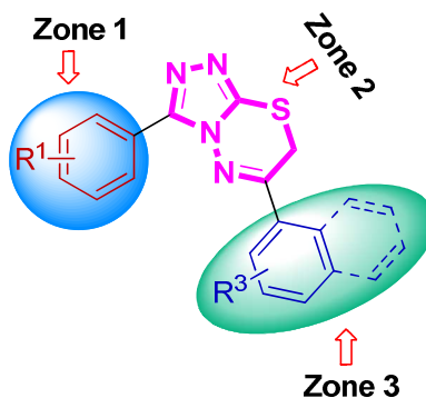
Fig. 12 The synthesized triazolothiadiazine structures ( 5a–p ) investigated herein.
