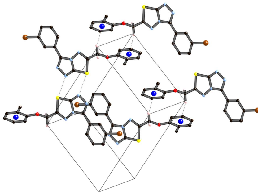
Fig. 6 Partial packing diagram illustrating the N...S sigma-hole interaction and the \pi - \pi and C-H... \pi interactions in crystals of 4i .
