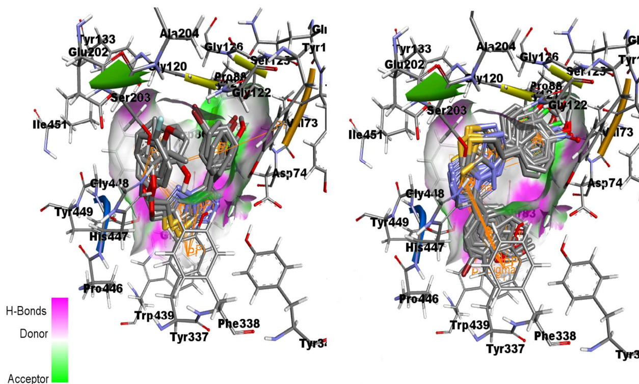
Fig. 15 Overlap of 4a , 4i , 4j , 4k and 4l inside active site of AChE (left) and overlap of 5a , 5b , 5g , 5h ,
