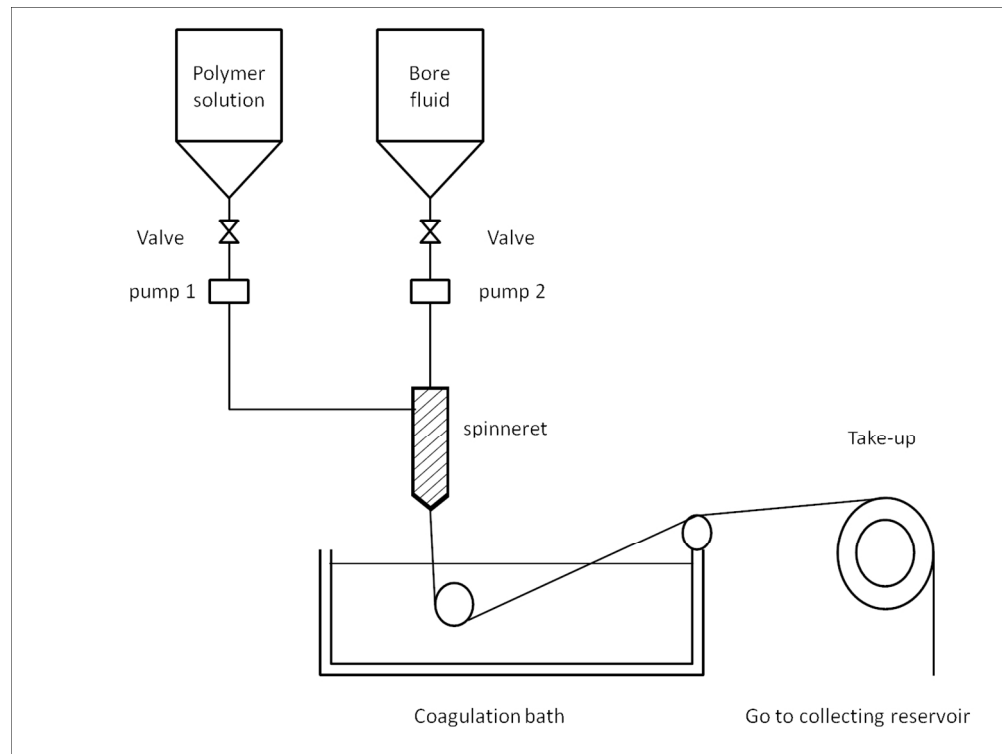
Fig.20. Schematic diagram of the spinning apparatus for hollow fiber membrane. 127x95mm (300 x 300 DPI)
