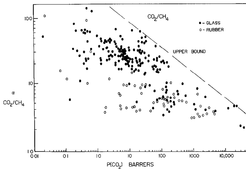
Fig.7. Literature data for CO 2 /CH 4 ideal selectivity versus CO 2 permeability (1991). 166x108mm (300 x 300 DPI)
