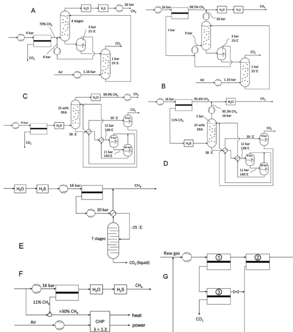
Fig. 32. Membrane hybrid processes for which gas permeation technology is combined with pressurized water scrubbing (PWS1-2: A-B), amine scrubbing (amine 1-2: C-D) equipment, a cryogenic separation (cryogen: E), and a Combined Heat and Power engine (CHP:F), three stage gas permeation process (G).
