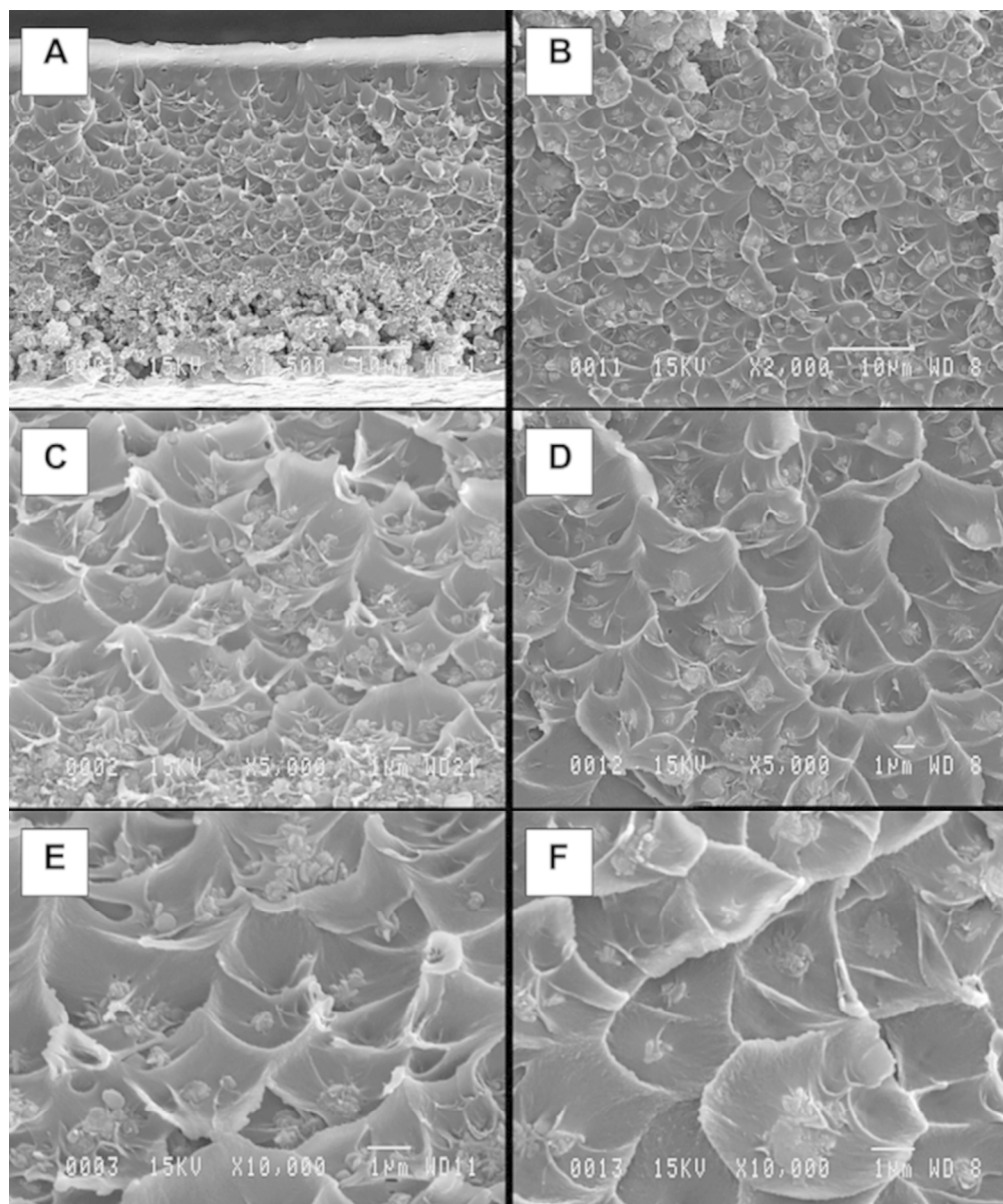
Fig.11. SEM micrographs of M-Zo Matrimid/non-amine-grafted zeolite (A, C, E) and M-IPA-3ET Matrimid/amine-grafted zeolite (B, D, F). 127x151mm (300 x 300 DPI)
