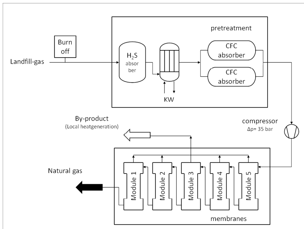
Fig.29. Flow chart diagram of the pilot plant. 127x95mm (300 x 300 DPI)
