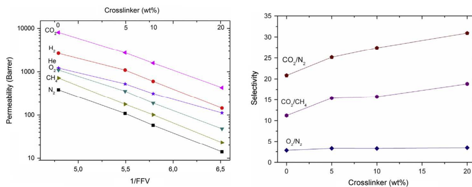
Fig.16. Permeability of N 2 , CH 4 , O 2 , He, H 2 , CO 2 and gas pair selectivity of CO 2 /N 2 , CO 2 /CH 4 and O 2 /N 2 in PIM-1 and crosslinked PIM-1 PEG-Biazide membranes as 1/FFV and ratio of crosslinker. 231x87mm (300 x 300 DPI)
