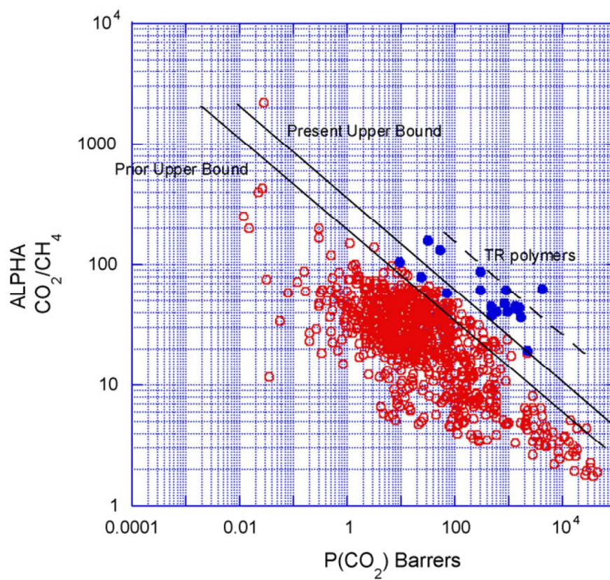
Fig.8. Robeson upper bound correlation for CO 2 /CH 4 separation 2008 (Alpha CO 2 /CH 4 is selectivity of CO 2 /CH 4 ; TR, thermally rearranged data refe.). 162x137mm (300 x 300 DPI)
