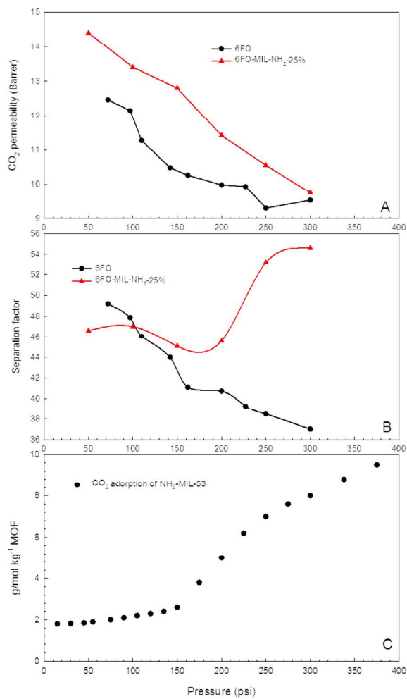
Fig.13. CO 2 permeability (A) and separation factor ( \alpha^* ) (B) for gas mixture (CO 2 :CH 4 = 50:50) as a function of feed pressure for 6FO (6FDA-ODA) and 6FO-MIL-NH 2 -25% membrane at 308 K. CO 2 adsorption isotherm of pure Al-MIL-53-NH 2 MOF (C). 119x123mm (300 x 300 DPI)
