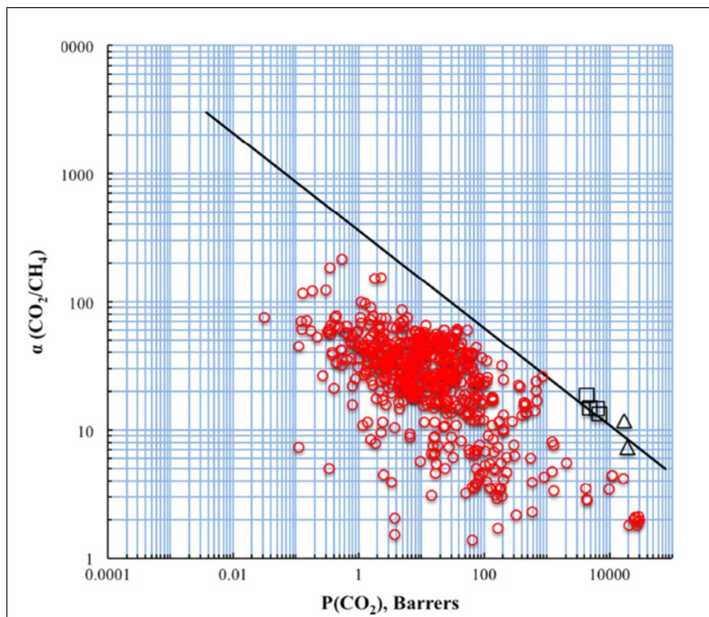
Fig.17. Correlation of permeability and permselectivity for CO 2 /CH 4 gas pair. The solid line is the Robeson upper bound of 2008. Triangles indicate PIM-1/ZIF-8 films after ethanol treatment, squares PIM-1/ZIF-8 films as cast. 111x95mm (300 x 300 DPI)
