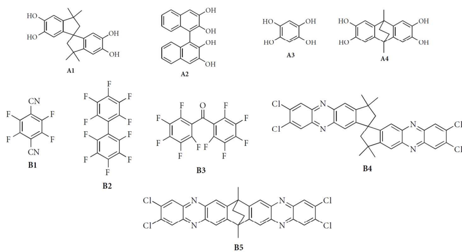
Fig.14. Structure of monomers for the synthesis of PIMs 1-10. 211x117mm (300 x 300 DPI)
