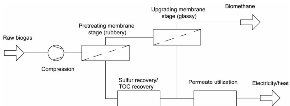
Fig. 31. A simplified process scheme including process integration of the hybrid membrane system for the desulfurization and upgrading of biogas. 254x105mm (300 x 300 DPI)
