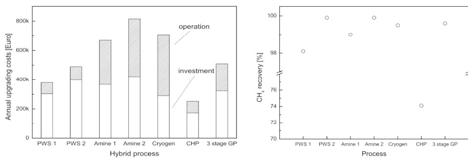
Fig. 33. Annual operation costs splitted in annual operation costs and annual costs for investment (A) and CH 4 recovery for the different hybrid processes at a feed flow rate of 1000 m 3 (STP)/h (B). The CH 4 recovery of the hybrid combined heat and power process (CHP) is significantly lower compared to the other process configuration.
