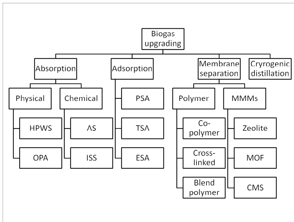
Fig.4. Current technologies for biogas upgrading. 127x95mm (300 x 300 DPI)
