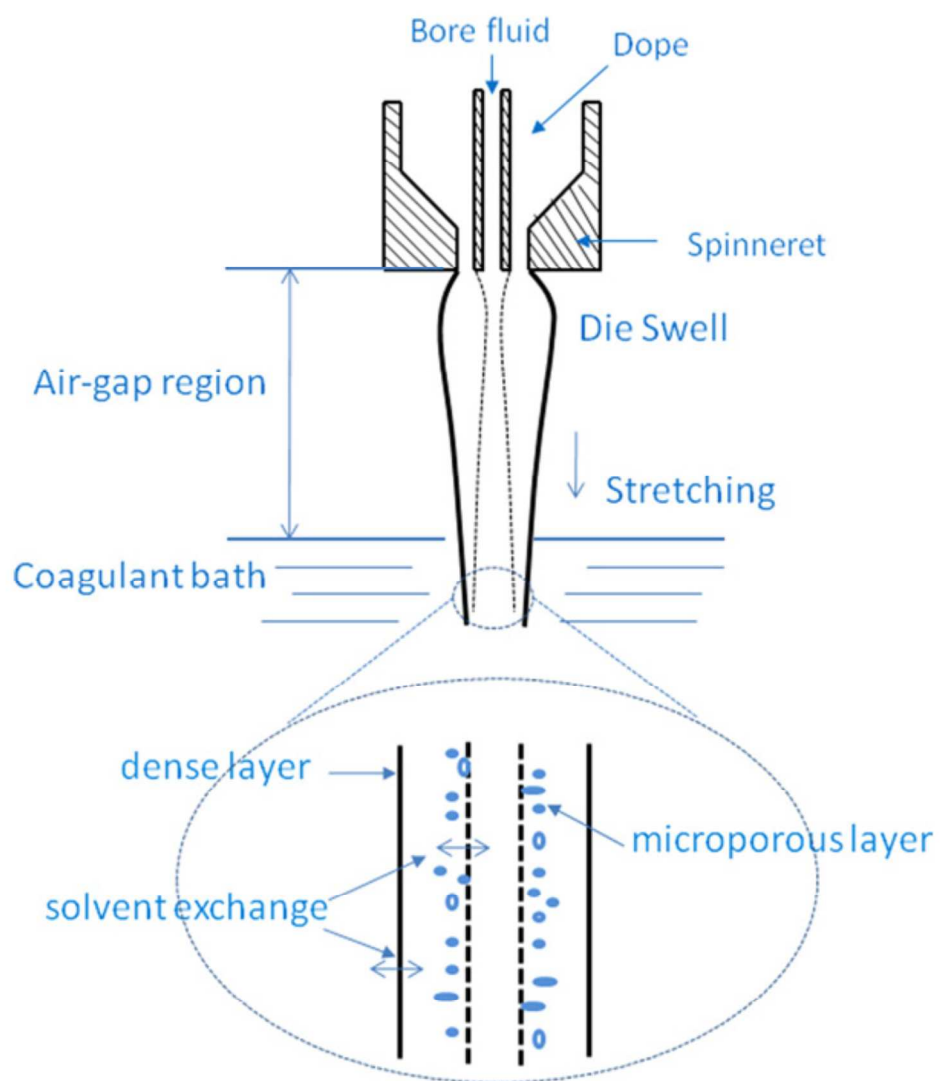
Fig.21. Schematic diagram of area nearby the spinneret and the formation of nascent hollow fiber during phase inversion. 137x158mm (300 x 300 DPI)
