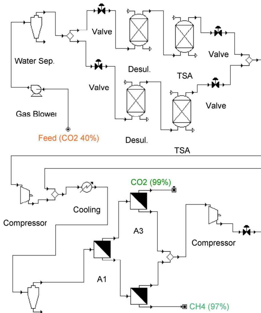
Fig.30. Flow-chart of a membrane process designed for upgrading biogas from wastewater plant digesters, with the adsorption and temperature-swing-adsorption as the pre-treatment. 236x260mm (300 x 300 DPI)
