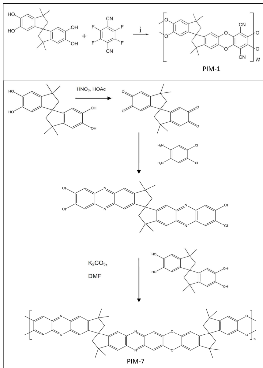
Fig.15. Preparation and structures of polymers PIM-1 and PIM-7. Reagents and conditions: (i) \text{K}_2\text{CO}_3 , \text{DMF} , 65\text{ }^\circ\text{C} ; (ii) \text{Conc. HNO}_3 , \text{HOAc} ; (iii) \text{HOAc} , reflux; (iv) 18-crown-6, \text{K}_2\text{CO}_3 , \text{DMF} , 150\text{ }^\circ\text{C} . 180x251mm (300 x 300 DPI)
