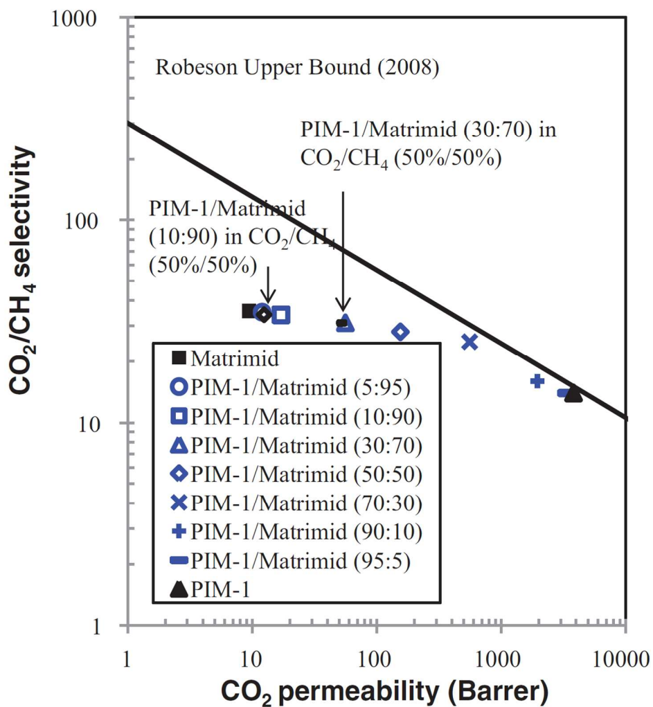
Fig.19. Comparison with Robeson upper bound of PIM-1/Matrimid polymer blends of \text{CO}_2/\text{CH}_4 . 235x250mm (300 x 300 DPI)
