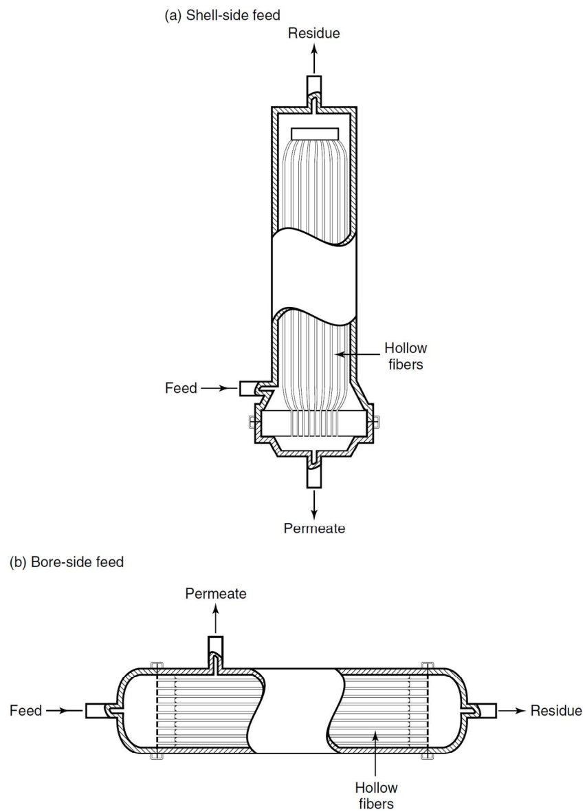
Fig.24. Two types of hollow-fibre modules used for gas separation applications. 155x198mm (300 x 300 DPI)
