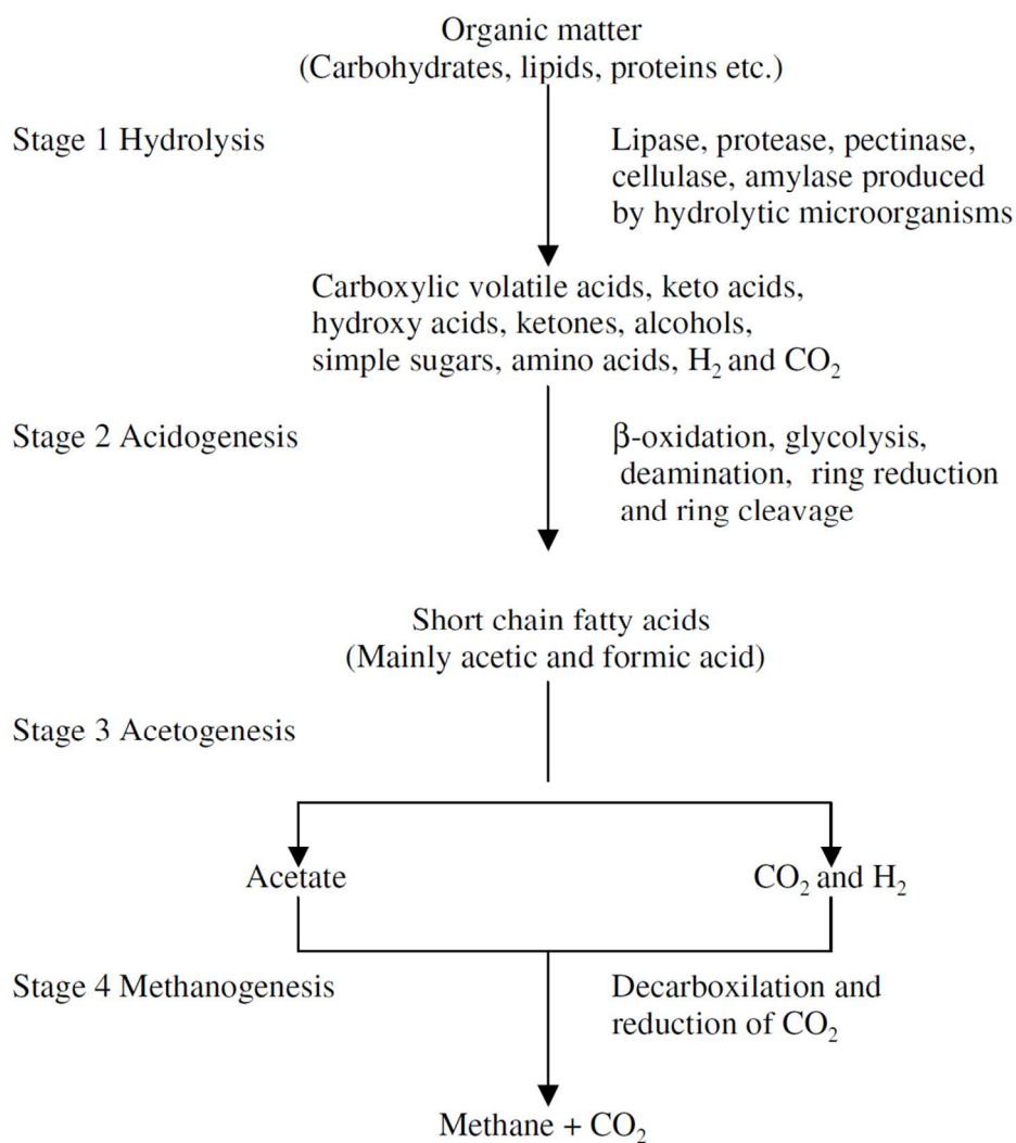
Fig.3. Metabolic route for the conversion of organic matter to the methanogenic substrates (acetate, CO 2 and H 2 ) and finally to CH 4 and CO 2 . 113x124mm (300 x 300 DPI)
