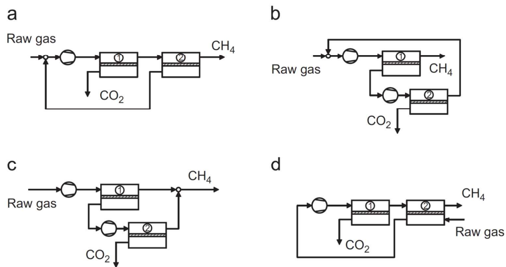
Fig.27. Two stage processes for biogas upgrading. 189x100mm (300 x 300 DPI)
