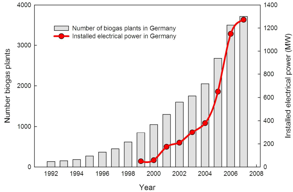
Fig.2. Development of biogas plants in in Germany between 1992 and 2007. 162x118mm (300 x 300 DPI)
