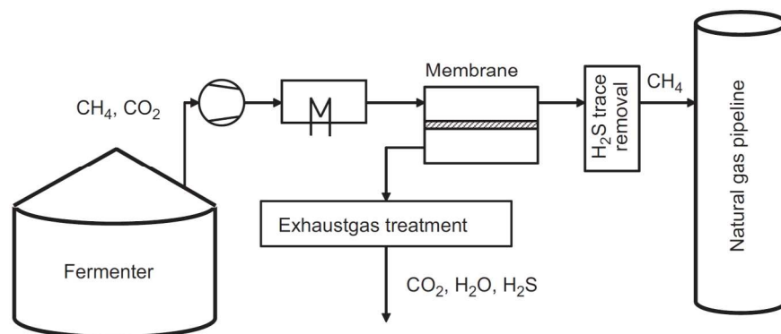
Fig.25. The process equipment for a membrane-based upgrading process. 216x89mm (300 x 300 DPI)
