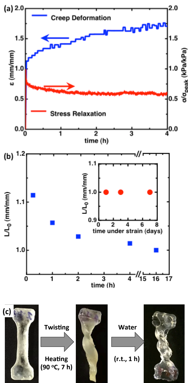
Figure 2. a) Stress-relaxation and creep data for a PHEA-FMIDA-UPyA based self-healing material monitored over 4 hours. b) Kinetic plot of measured length after extension ( L ) compared to length before extension ( L_0 ) L/L_0 as a function of time after the PHEA-FMIDA-UPyA material was released from 7 days at 100% strain (inset shows the L/L_0 16 h after being released from 100% extension that was maintained for 1, 3 and 7 days). c) Photograph of the shape of the PHEA-FMIDA-UPyA material directly after synthesis (left), after being heated for 7h at 90 °C (middle), and after being placed in a room temperature water bath for 1h (right).
