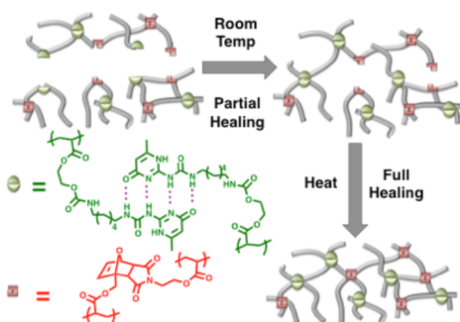
Scheme 1. Synthesis and proposed healing mechanism of the PHEA-FMIDA-UPyA material. Initially the hydrogen bonded UPyA units join to partially heal the material. With thermal stimulus the covalently linked FMIDA units join across the interface.
