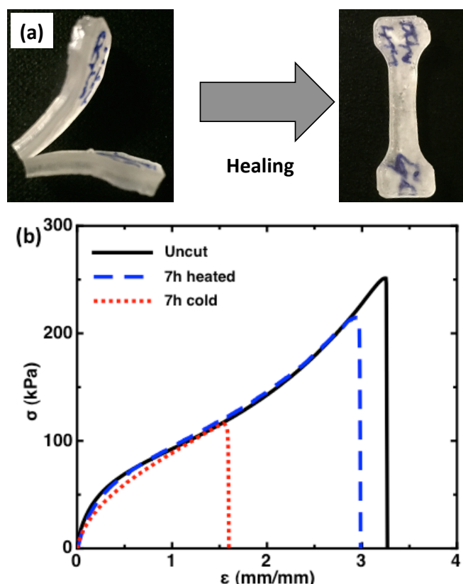
Figure 1. a) Left shows the PHEA-FMIDA-UPyA material directly after being cut with a razor. Right shows the same material with the scratch being much less prominent after 7h of room temperature healing. b) Comparison between the uncut and the PHEA-FMIDA-UPyA materials that were cut and healed under cold conditions for 7h (room temperature) and cut and heated at 90 °C for 7h.
