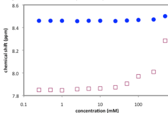
Figure 1. Change in the N-H chemical shifts for ortho-fluoro 8 (●) and ortho-chloro 10 (□) with varying concentration.
