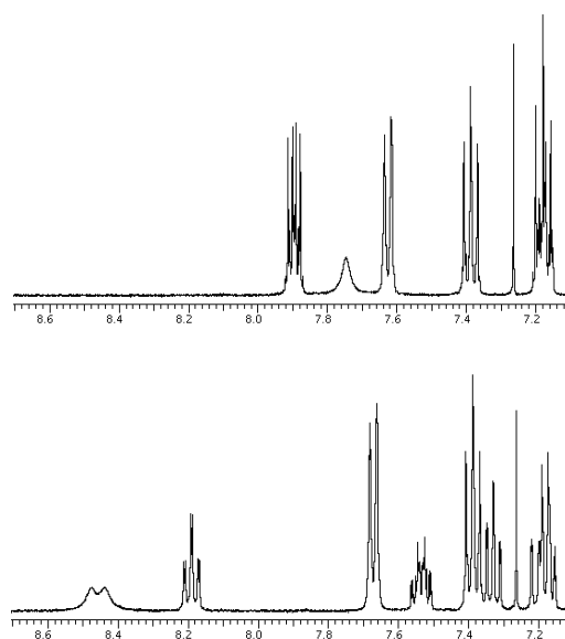
Figure 2. NMR of para-fluoro 9 (top) and ortho-fluoro 8 (bottom) in CDCl 3 (400 MHz, 22°C). Coupling can be observed in the NH signal at the bottom left.
