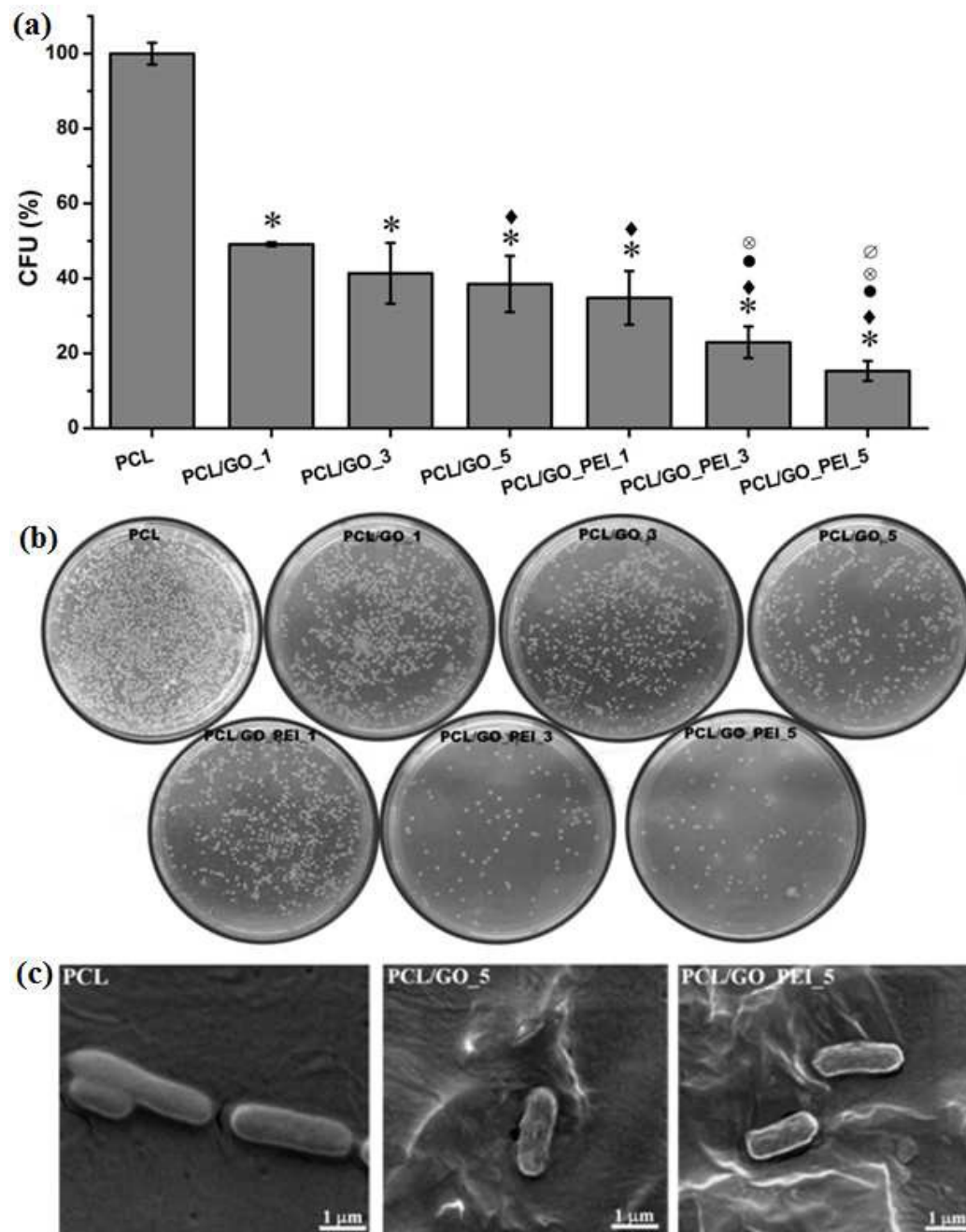
Figure 7: Antibacterial study showing (a) Colony count of E. coli on the different composites with respect to neat PCL. (b) Photographs of viable E. coli colonies grown on LB agar plates. (c) SEM micrographs of bacterial morphology on PCL, PCL/GO_5 and PCL/GO_PEI_5 surfaces.
