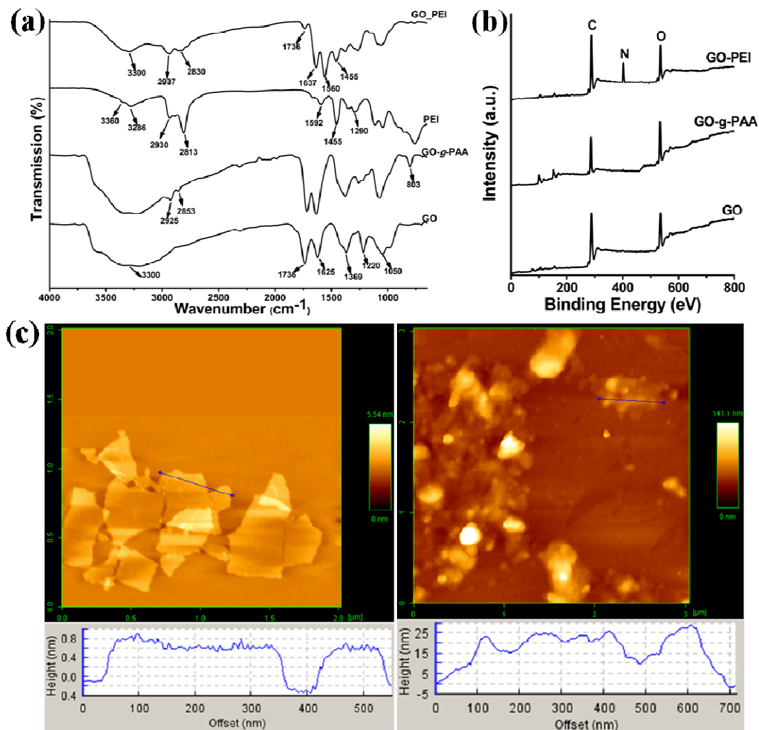
Figure 2: Characterization of the synthesized nanoparticles (a) FTIR spectra of GO, GO-g-PAA, PEI and GO-PEI, (b) XPS spectra for GO, GO-g-PAA and GO-PEI, (c) AFM images with flake thickness profile of GO and GO-PEI,
