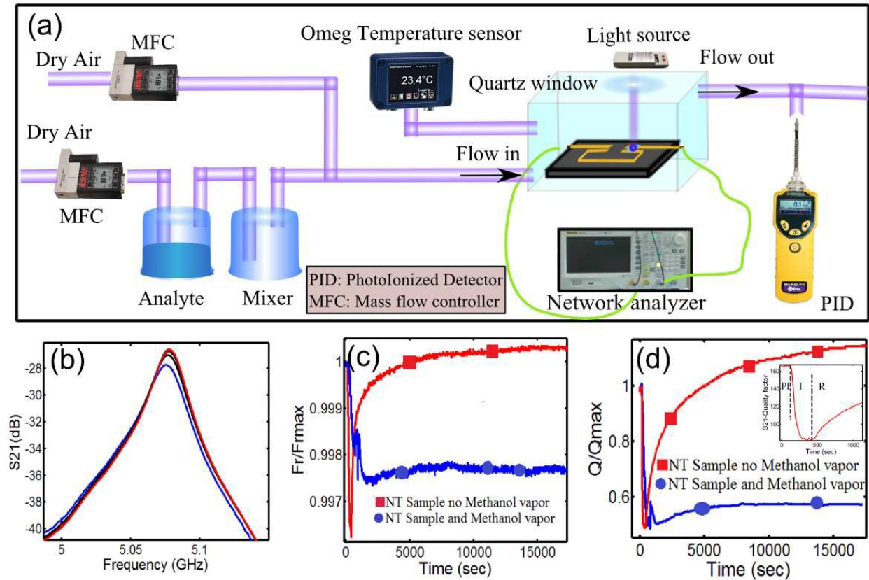
Fig. 3 (a) Schematics of the Experiment setup, (b) S21 profile of the resonator with nanotube and during the illumination time, (c) Normalized resonance frequency variation to the initial resonance frequency of the sensor, (d) Normalized quality factor variation to the initial quality factor of the sensor during the time period of 5 hours; with an inset of Q variation with no methanol vapor illustrating a clear transitions between the following phases: prior to illumination (PI) , during illumination (I) and relaxation (R)
