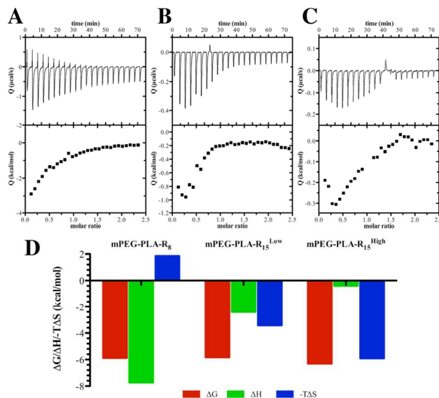
Figure 4. Thermodynamic profiles of single stranded miRNA binding to micelles indicate different interactions occur dependent upon oligoarginine length and density. (A) mPEG-PLA-R 8 (B) mPEG-PLA-R 15 Low (C) mPEG-PLA-R 15 High (D) Thermodynamic parameters, derived from ITC, of miRNA binding to mPEG-PLA-R 8 , mPEG-PLA-R 15 Low , and mPEG-PLA-R 15 High micelles.
