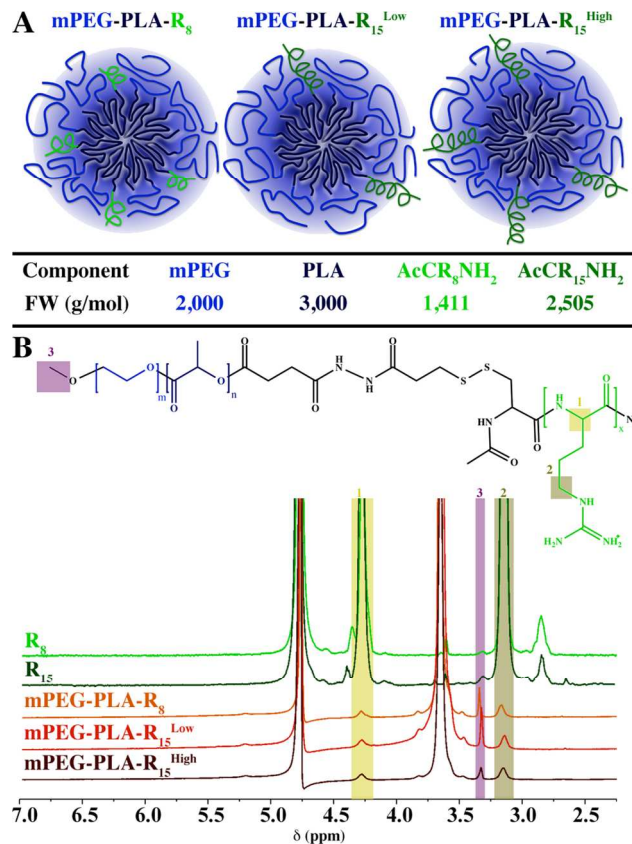
Figure 1. Micelles properties and surface oligoarginine presence. (A) Schematic representation of the micelles formed and the relevant molecular weights of the components. (B) 1 H NMR analysis of the peptides (CR 8 and CR 15 ) and micelles (mPEG-PLA-R 8 , mPEG-PLA-R 15 Low , and mPEG-PLA-R 15 High ) showing the arginine \alpha proton (1; \delta = 4.40 ppm, 1H), \delta protons (2; \delta = 3.20 ppm, 2H), or \omega -terminal methoxyl protons (arrow; \delta = 3.40 ppm, 3H).
