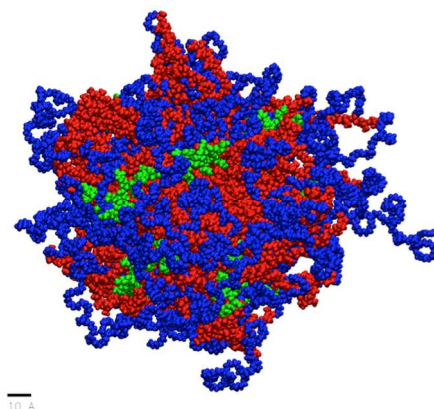
Figure 2. Molecular dynamics simulation of mPEG-PLA-R 8 micelle. Each monomer consisted of a methoxy-poly(ethylene-glycol)(mPEG; MW ~ 2,000 g/mol; blue) block coupled to the \alpha -hydroxide of poly(lactide) (PLA; MW ~ 3,000 g/mol; red). As in the experiments, 28% of total monomers were modified with oligoarginine (R 8 ; green) on the \omega -carboxylate of the PLA block. The micelles were prepared with total 60 monomers.
