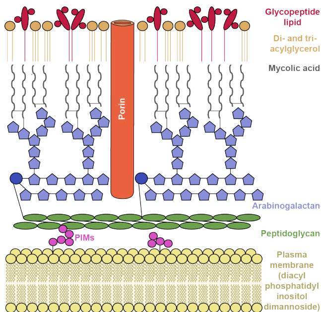
Fig. 7. Mycobacterium cell wall.
