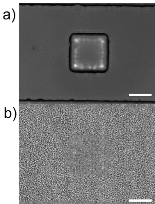
Figure 1: (a) Bright field image of 200 nm polystyrene particles (concentration 0.05% by weight) dispersed in deionized water flowing through a microchannel containing a square pillar (80 μm × 80 μm). The average volumetric flow rate is 10 μl/min and the flow direction is from left to right. (b) Speckle pattern of the bright field image obtained by subtraction of the median image. Scale bars are 50 μm.
