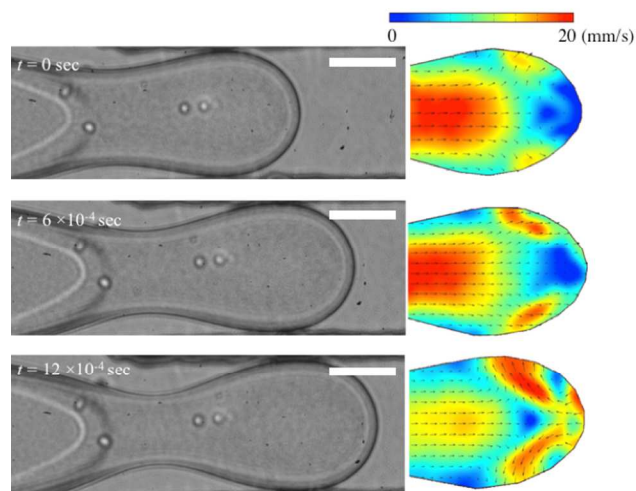
Figure 34: (Left) Bright field images of an aqueous phase seeded with 200 nm polystyrene particles (0.05% by weight) necking in the drop making junction at time intervals of 600 \mu\text{s} and at the channel mid-plane prior to pinch-off. (Right) Comparison of the corresponding velocity distributions in the aqueous phase. Scale bars are 50 \mu\text{m} . The focal plane considered is the mid-plane.
