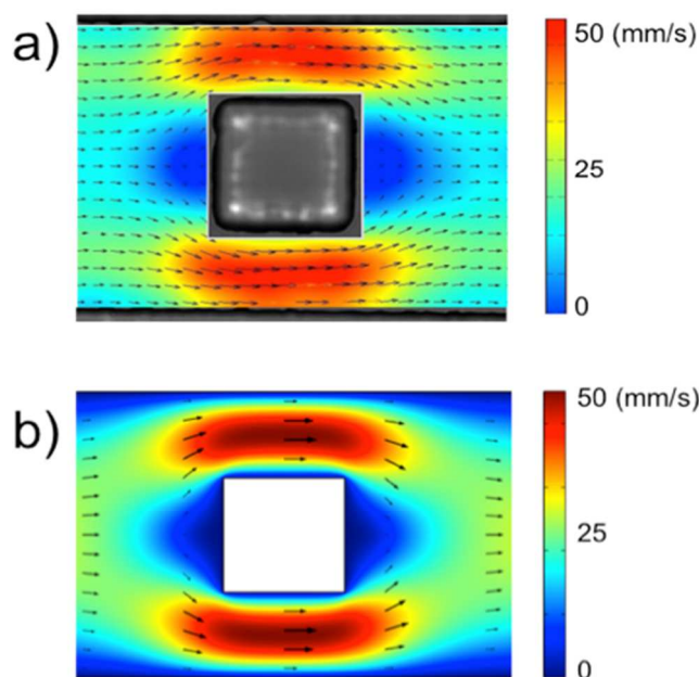
Figure 2: Comparison of the flow velocity field around a 80 μm × 80 μm pillar within a microchannel obtained experimentally (a) and via a finite element simulation (b).
