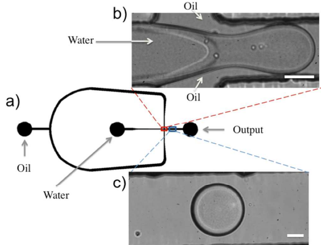
Figure 43: Droplet Generation at a flow focusing geometry. (a) The microfluidic device is made by standard soft-lithography in PDMS and contains rectangular cross-section channels with a height of 50 \mu\text{m} . To produce droplets, fluorinated oil (FC-40) containing 2% w/w surfactant is used as the continuous phase and deionized (DI) water seeded with 200 nm polystyrene particles as the dispersed phase (0.05% by weight). (b) Bright field image of drop formation at a generation rate of 600 Hz. (c) A bright field image of a droplet 300 microns downstream of the formation point. Scale bars are 25 \mu\text{m} . The focal plane considered is the mid-plane.
