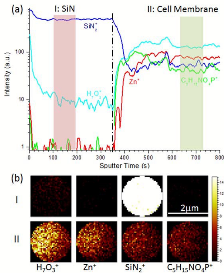
Fig. 3. ToF-SIMS depth profiling and 2D imaging of C10 cell. (a) ToF-SIMS depth profile of a hydrated C10 cell in SALVI. Two time regions indicating different depths are highlighted and defined as I (100-200 s) or before SiN punch-through and II (650-750 s) or in the cell membrane. The black dashed line indicates the beginning of SiN punch-through. (b) 2D ToF-SIMS images of \text{H}_7\text{O}_3^+ (m/z 55), \text{SiN}_2^+ (m/z 56), \text{Zn}^+ (m/z 64), and phosphorylcholine \text{C}_5\text{H}_{15}\text{NO}_4\text{P}^+ (m/z 184) reconstructed corresponding to regions I and II in (a), respectively.
