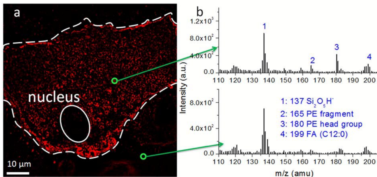
Fig. 2. Correlative imaging of C10 cells by SIM and ToF-SIMS. (a) Fluorescence SIM image of a C10 cell in SALVI. (b) ToF-SIMS negative m/z spectra acquired at the corresponding locations highlighted in green circles in (a).
