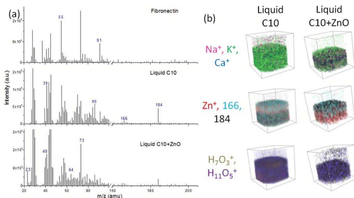
Fig. 4. (a) ToF-SIMS positive spectra of the fibronectin coated SiN and water interface, liquid C10 cell and liquid C10 cells treated with ZnO NPs in SALVI. (b) 3D images of several key m/z components of C10 and C10 cells exposed to ZnO NPs. 3D images were reconstructed from 0-800 s from the depth profiling time series in Fig. 3.
