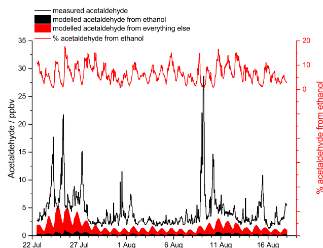
Fig. 7 Modelling results of the impacts of current levels of ethanol observed in London. The measured acetaldehyde during the summer campaign (black), acetaldehyde formed in the model from the reaction of OH and ethanol (black filled area) and other photochemical acetaldehyde sources in the model (red filled area) are plotted on the left y axis. The percentage of the measured acetaldehyde that was directly formed from ethanol (red) is plotted on the right y axis
