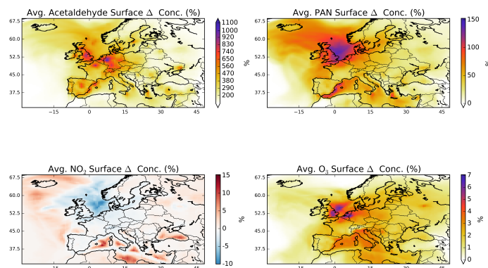
Fig. 9 Average fractional increases in surface acetaldehyde, PAN, NO_2 and O_3 concentrations with the inclusion of both a primary ethanol emissions and an increase in acetaldehyde emissions, ('GEOS-Chem+EOH+ALD2'). Shown averaged over the summer period.
