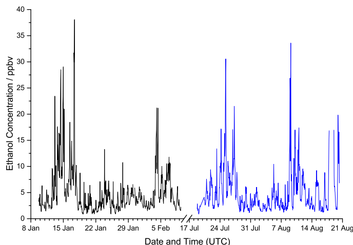
Fig. 2 Time series of ethanol in the winter (left panel, black) and summer (right panel, blue)
