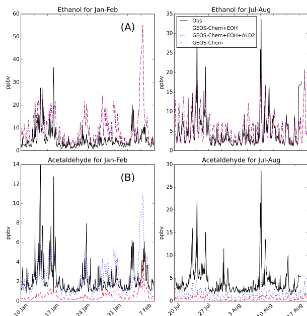
Fig. 8 Comparison between modelled values and observed for ethanol (A) and acetaldehyde (B) for winter (left) and summer (right) observation periods. Plots show the base model simulation without increased ethanol or aldehyde emissions ('GEOS-Chem') in magenta, with added ethanol emissions ('GEOS-Chem+EOH') in red, and with both additional ethanol and acetaldehyde emissions ('GEOS-Chem+EOH+ALD2') in blue.
