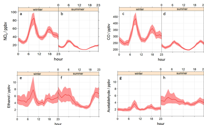
Fig. 3 Diurnal profiles of \text{NO}_x (a and b), CO (c and d), ethanol (e and f) and acetaldehyde (g and g) in winter (left-hand side of each plot) and summer (right-hand side of each plot). Each compound has the winter and summer plots on the same y-axis to aid direct comparison. This figure was constructed using the OpenAir project for R where the solid line represents the mean daily concentration and the shaded regions show the 95% confidence intervals surrounding the mean. 33–35
