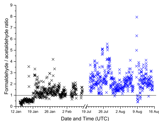
Fig. 6 Time series of the formaldehyde/acetaldehyde ratio from the winter (left, black) and summer (right, blue) campaigns, the black line indicates an f/a ratio of 1.
