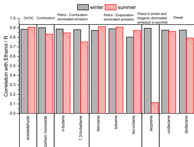
Fig. 5 Correlation of selected compounds with ethanol in winter (left column) and summer (right column), grouped by emission source and ordered by carbon number
