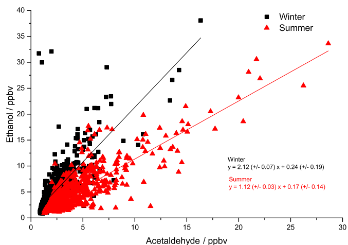
Fig. 4 Linear regression of ethanol and acetaldehyde in the winter (black squares) and summer (red triangles) campaigns
