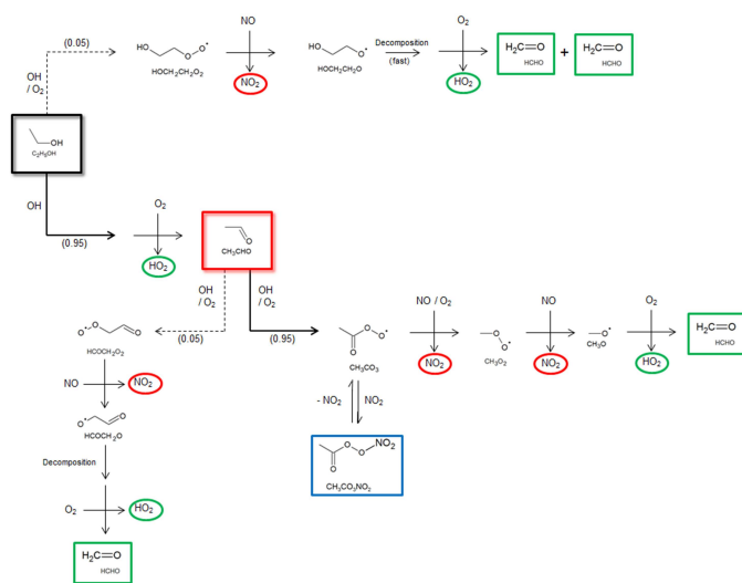
Fig. 1 Simplified schematic mechanism for the photo-oxidation of ethanol initiated by the OH radical taken from MCM. 25 Ethanol is boxed in black, with acetaldehyde in red, PAN (peroxyacetyl nitrate) in blue and formaldehyde in green. The NO to NO 2 conversions, highlighted by red circles, correspond to routes to photochemical ozone formation. HO 2 formation (highlighted in green circles) can also lead to NO to NO 2 conversions.
