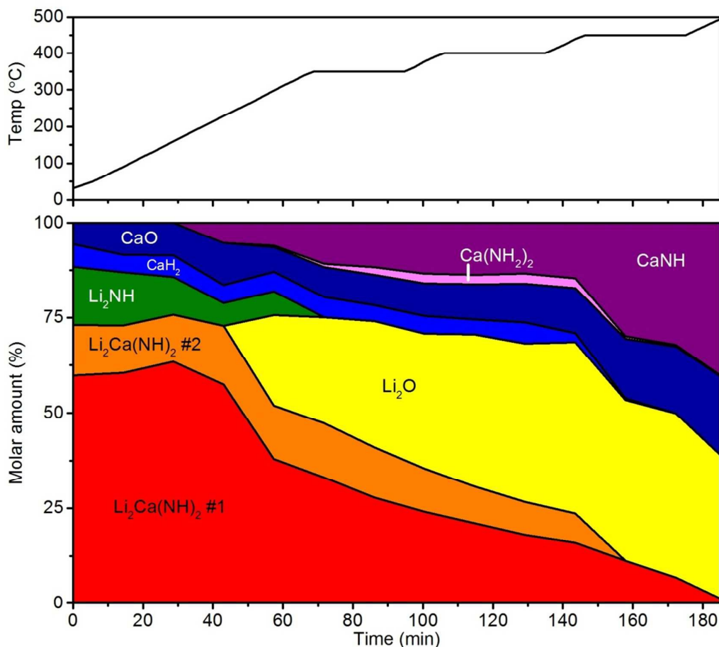
Figure 8 - Molar percentages of the crystalline phases present during exposure of lithium-calcium imide to ammonia, as extracted from Rietveld analysis of every fifth synchrotron X-ray powder diffraction data set. \text{Li}_2\text{Ca}(\text{NH})_2 #1 is the major component of the lithium-calcium imide peak; \text{Li}_2\text{Ca}(\text{NH})_2 #2 is the minor component.
