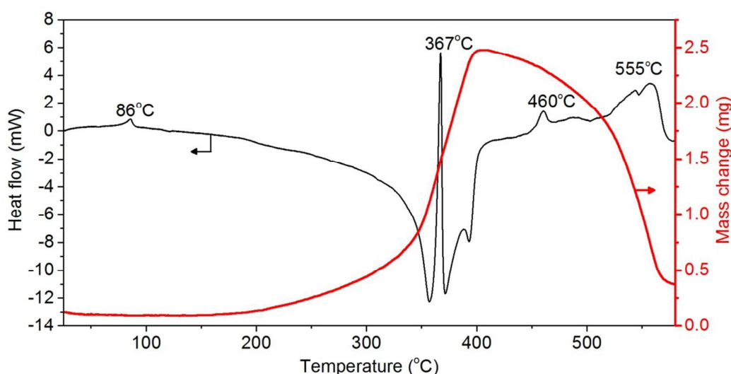
Figure 10 - Combined DSC-TGA experiment on lithium-calcium imide under 20 sccm flowing ammonia gas.
