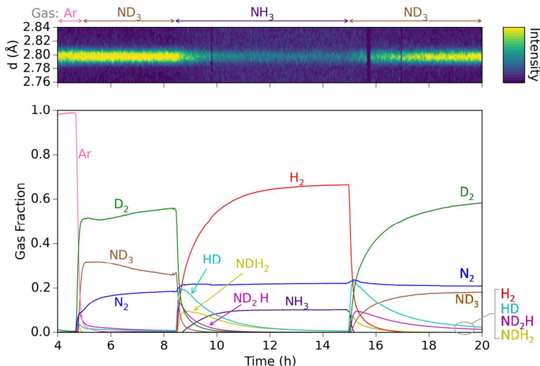
Figure 13 - Mass spectroscopy data during the isotope exchange reaction, with the neutron diffraction (011) Bragg peak of lithium-calcium imide shown for reference.
