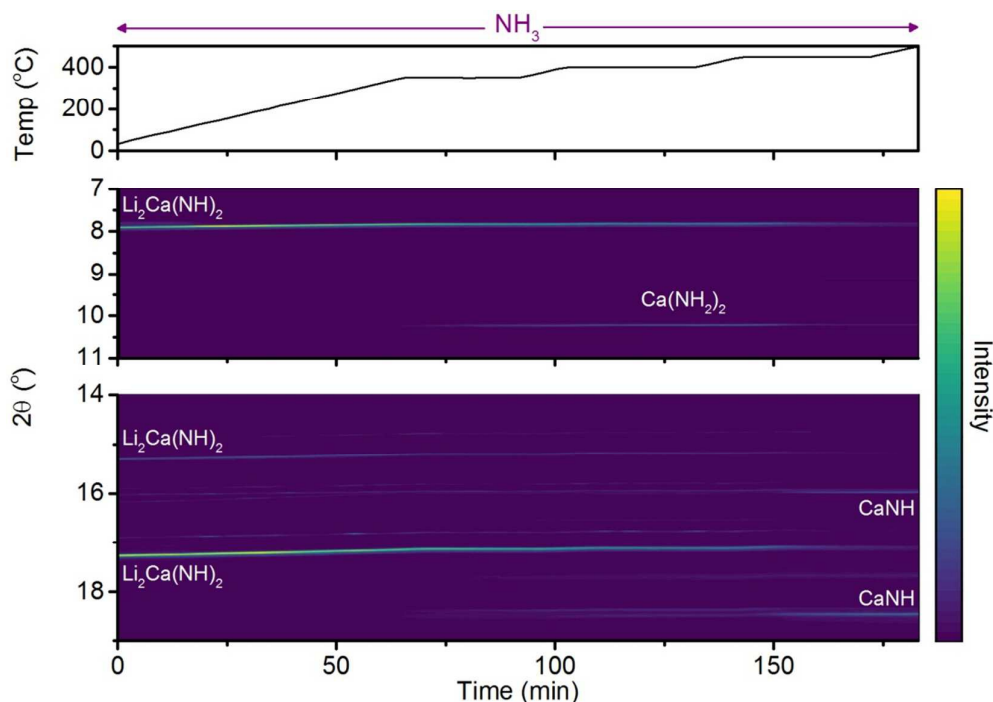
Figure 7 – Selected contour plots of synchrotron X-ray powder diffraction data for lithium-calcium imide heated under 1 sccm flowing ammonia gas.
