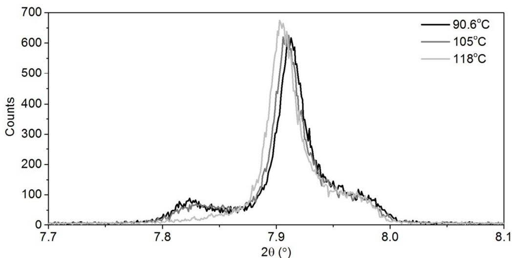
Figure 5 - The synchrotron X-ray powder diffraction (001) peak of lithium-calcium imide, showing the disappearance of the low-angle shoulder with heating under 1 sccm flowing helium, and the presence of high-angle asymmetry.
