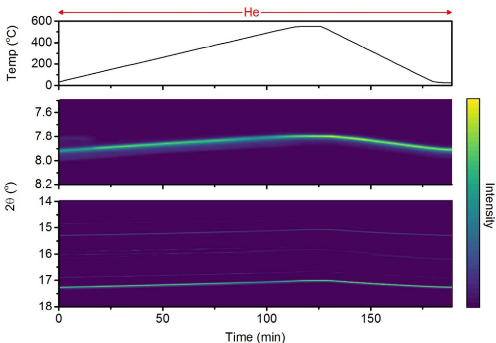
Figure 4 - Contour plot of sections of the in-situ synchrotron X-ray powder diffraction data for lithium-calcium imide. The sample was heated at 5 °C/min under 1 sccm flowing helium gas.
