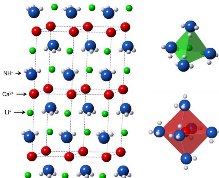
Figure 3 - Crystal structure of lithium-calcium imide, with lithium atoms shown in green, calcium in red, nitrogen in blue and hydrogen in grey. The local geometries of the \text{Li}(\text{NH})_4 tetrahedron and \text{Ca}(\text{NH})_6 octahedron are shown to the right.
