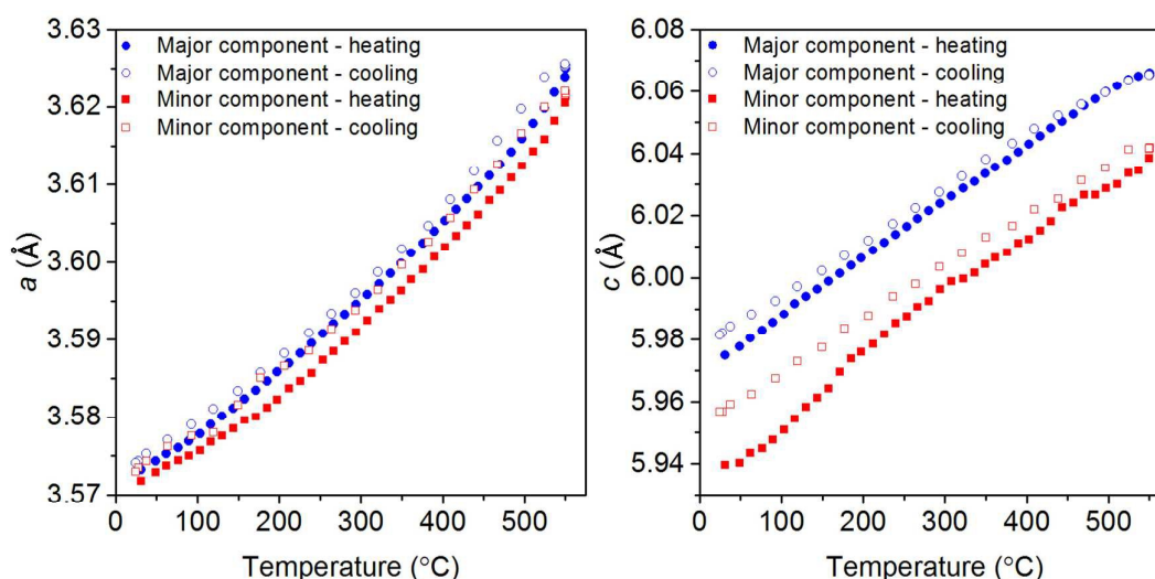
Figure 6 – Lattice parameters a and c for the two lithium-calcium imide components included in the refinement of the synchrotron diffraction data for the heating of lithium-calcium imide under flowing helium gas. Errors in the lattice parameter values are 1\text{-}2 \times 10^{-4} Å.
