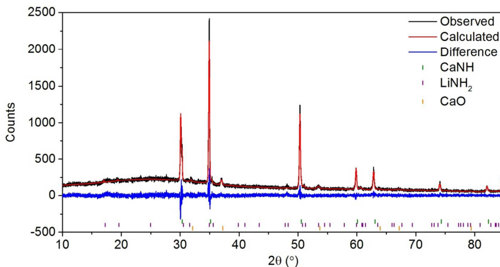
Figure 2 - X-ray powder diffraction pattern of the lithium-calcium imide catalyst after the ammonia decomposition reaction.
