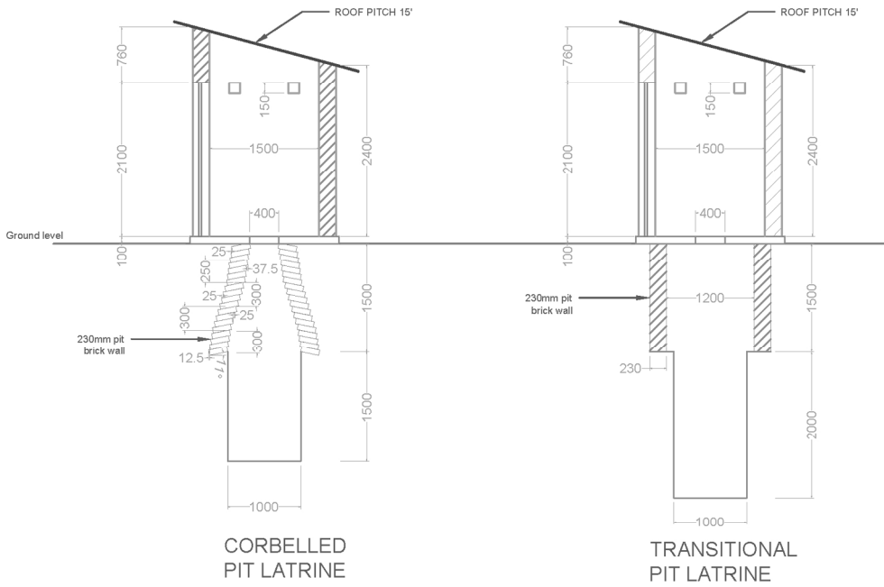
Corbelled and improved transitional pit latrine representation 221x172mm (200 x 200 DPI)
