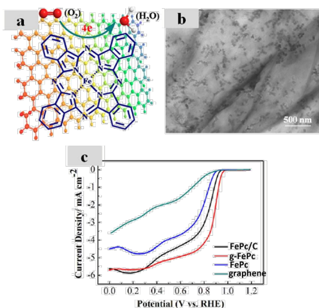
Figure 8. (a) Schematic of the interaction between FePc and graphene (g-FePc) and the ORR happening on g-FePc (b) TEM of g-Fe-Pc and (c) comparison of FePc/C and g-FePc in 0.1 M KOH at 1600 rpm. Reprinted in adapted form with permission from 115 copyright (2013)
