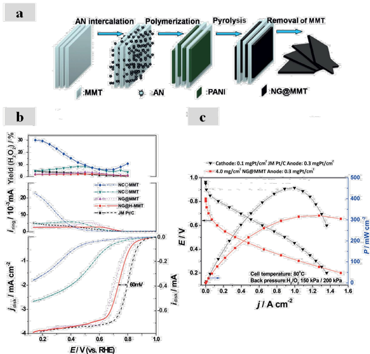
Figure 12. (a) Schematic of the synthesis of NG@MMT. (b) ORR polarization, ring current, and peroxide yield in 0.1 M HClO 4 . (c) Power densities and corresponding polarization curves of MEA prepared from NG@MMT. Reprinted from 154 with permission from John Wiley and Sons.
