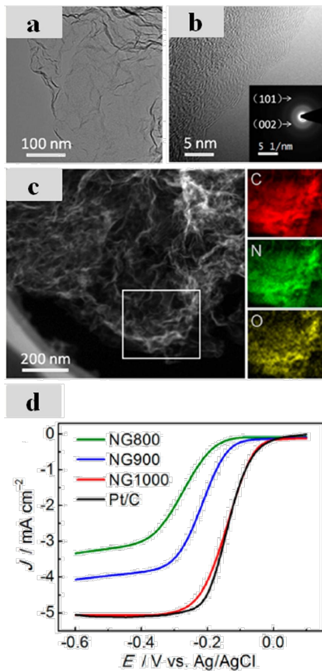
Figure 11. (a) TEM, (b) HRTEM and (c) STEM images of NG1000. (d) ORR polarization curves of different samples and Pt/C at 1600 rpm in 0.1 M KOH. Reprinted with permission from 144 . Copyright (2013) American Chemical Society.
