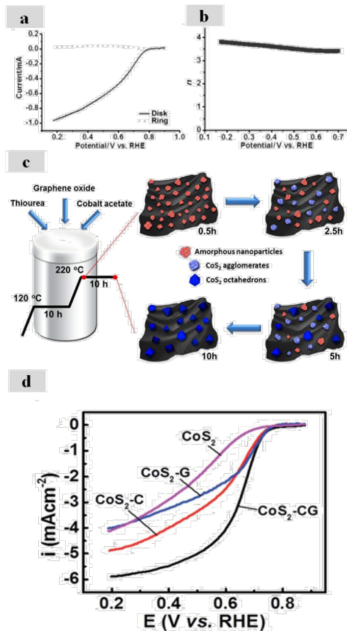
Figure 9. (a) RRDE results and (b) electron transfer number n of \text{Co}_{1-x}\text{S}/\text{RGO} in oxygen saturated 0.5 M \text{H}_2\text{SO}_4 . Reprinted from 119 with permission from John Wiley and Sons. Copyright (2011). (c) Schematic of the growth of \text{CoS}_2 octahedron nanoparticles supported on N and S doped graphene. (d) ORR curves of \text{CoS}_2 catalysts supported on different nanostructured carbon supports at 1600 rpm in 0.1 M \text{HClO}_4 . Reproduced in adapted form from 120 by permission of The Royal Society of Chemistry
