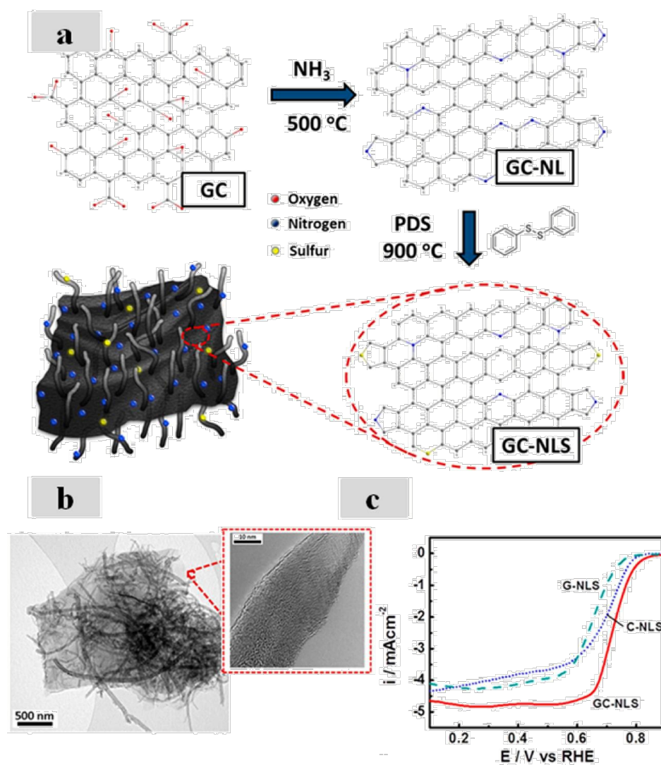
Figure 16. (a) Schematic of the step-wise doping process to fabricate GC-NLS nanocomposites.
