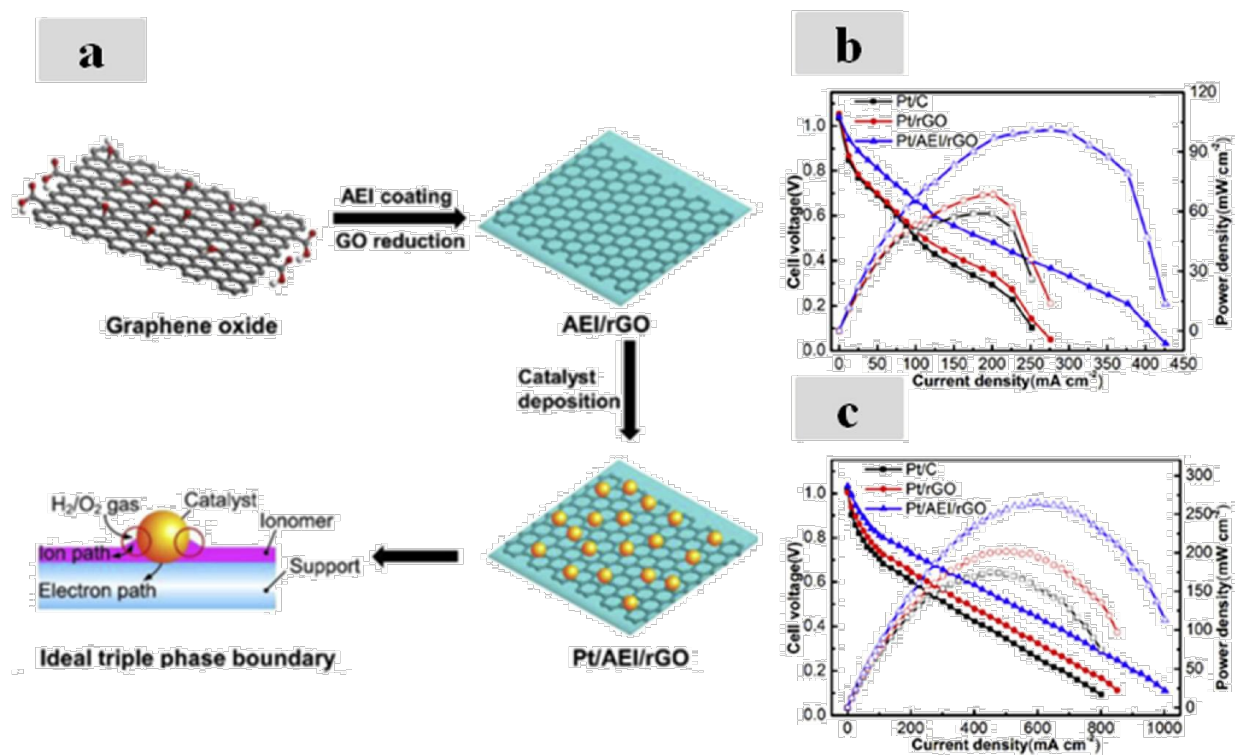
Figure 2. (a) Schematic of Pt/AEI/rGO catalyst preparation with ideal triple phase boundary. (b) power densities (empty symbols) and polarization (filled symbols) curves for a H 2 /O 2 AEM fuel cell without additional ionomer and (c) the catalyst layers with a total of 20 wt% ionomer.
