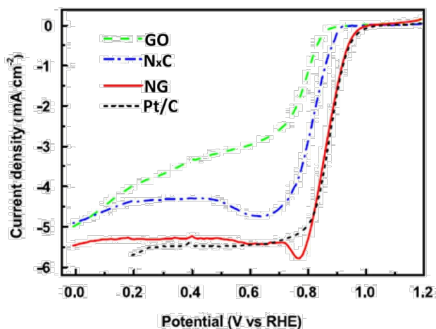
Figure 15. ORR polarization plot for of GO, N x C, NG and Pt/C catalysts in 0.1 M KOH at 1600 rpm. Reprinted in adapted form from 198 , Copyright (2015), with permission from Elsevier.
