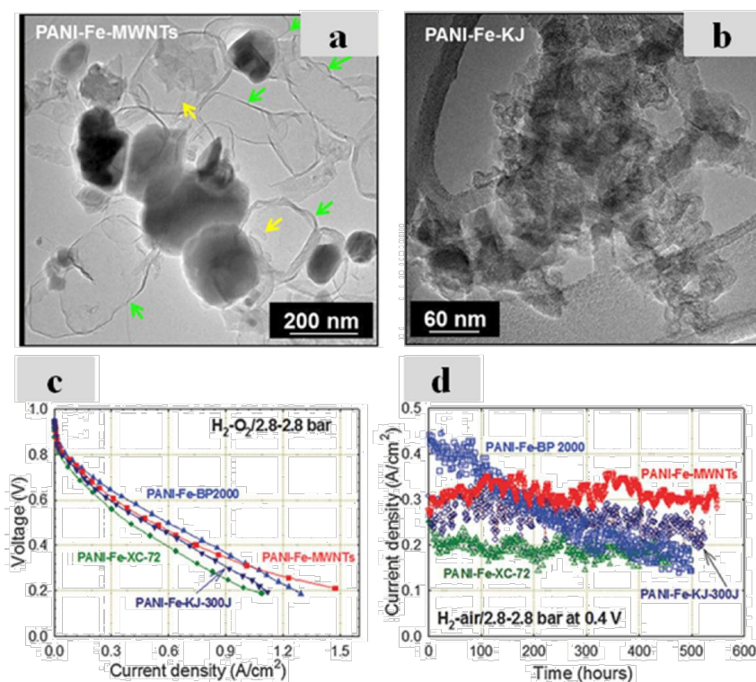
Figure 6. TEM images of (a) PANI-Fe-MWNTs and (b) PANI-Fe-KJ. (c) Initial H 2 -O 2 MEA polarization plots and (d) fuel cell durability testing. Reproduced from 97 with permission of The Royal Society of Chemistry.
