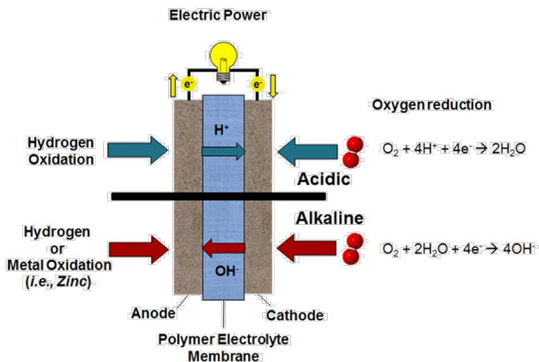
Figure 1. Schematic of typical pathways of oxygen reduction in (top) acidic PEFCs and (bottom) alkaline operating fuel cells or metal-air batteries during discharge.
