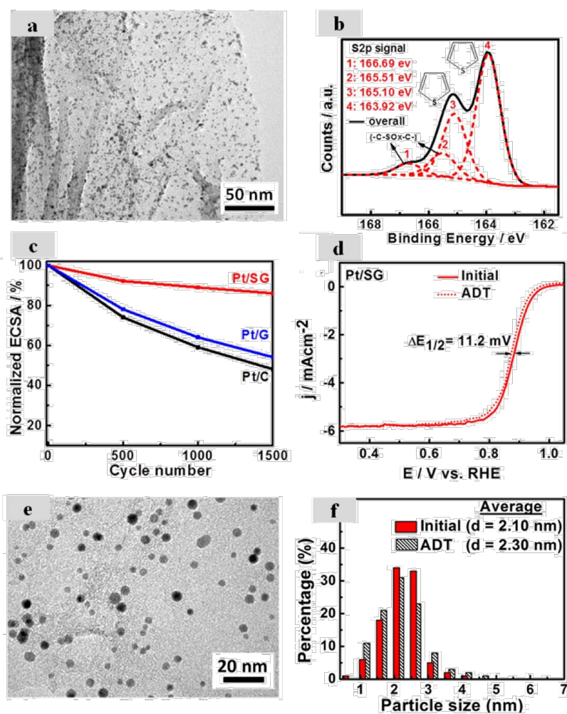
Figure 5. (a) TEM image of Pt/SG and (b) S2p spectra of SG. (c) normalized ECSA remaining through durability testing. (d) ORR polarization curves initially and after durability testing for Pt/SG. (e) TEM image after durability testing and (f) particle size distribution initially and after ADT for Pt/SG. Reprinted from 19 with permission from John Wiley and Sons. Copyright (2014).
