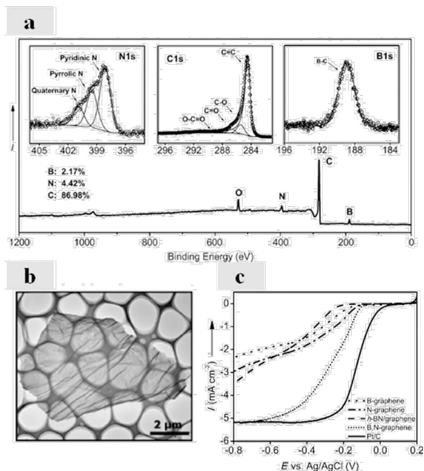
Figure 14. (a) XPS spectra of nitrogen, carbon and boron (B 1s) core levels in B,N-graphene. (b) TEM image of B,N-graphene and (c) linear sweep voltammetry (LSV) of different catalysts in oxygen saturated 0.1 M KOH. Reprinted from 187 with permission from John Wiley and Sons.
