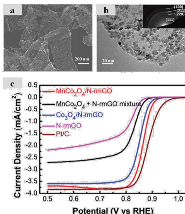
Figure 10. Low magnification (a) scanning electron microscopy (SEM) and (b) TEM image of \text{MnCo}_2\text{O}_4/\text{N-rmGO} hybrid. (c) RDE results of \text{MnCo}_2\text{O}_4/\text{N-rmGO} hybrid, \text{MnCo}_2\text{O}_4 + \text{N-rmGO} mixture, \text{Co}_3\text{O}_4/\text{N-rmGO} hybrid and Pt/C in oxygen saturated 1 M KOH. Reprinted with permission from 126 . Copyright (2012) American Chemical Society.
