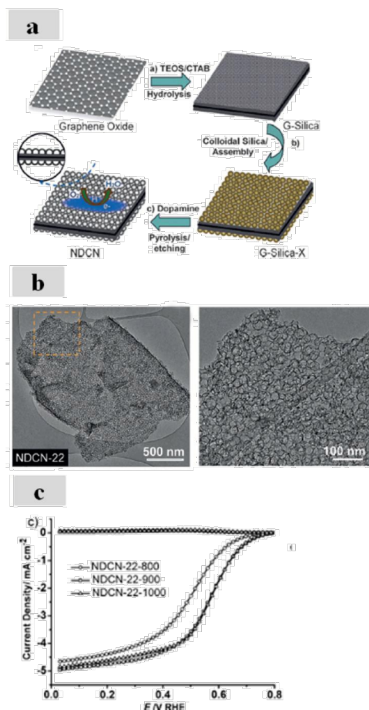
Figure 13. (a) Schematic of NDCN synthesis. (b) TEM images of NDCN-22. (c) RRDE results in O 2 -saturated 0.5 M sulfuric acid of NDCN-22 synthesized at different pyrolysis temperatures.
