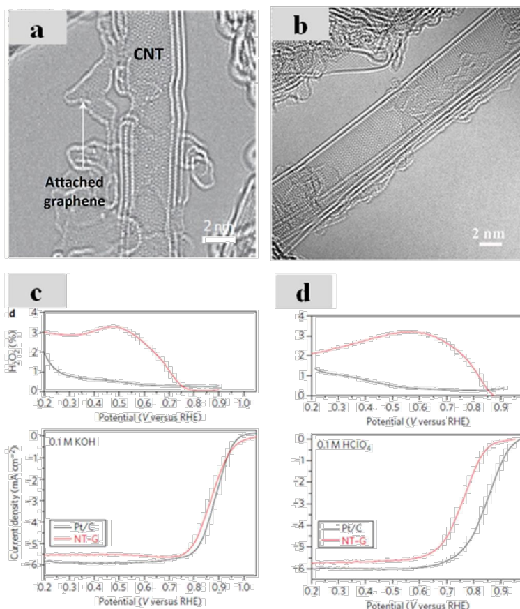
Figure 7. (a, b) TEM images of NT-G catalysts showing the exfoliated graphene pieces attached to CNTs. Rotating ring disk electrode (RRDE) polarization curves and peroxide yield of NT-G in (c) 0.1 M KOH and (d) 0.1 M HClO 4 . Reprinted in adapted form by permission from Macmillan Publishers Ltd 98 copyright (2012).
