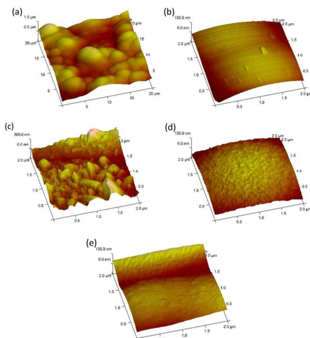
Figure 7: AFM images of electroless nickel substrate at (a) 20 \mu\text{m}^2 and (b) 2 \mu\text{m}^2 and the ENIG coatings at 2 \mu\text{m}^2 for (c) sample 1, (d) sample 2 and (e) sample 3, Figure 5 .
