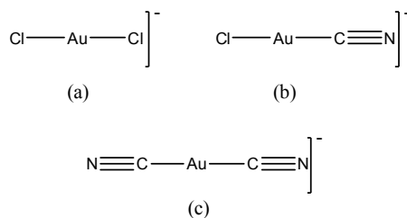
Figure 2: Proposed speciation of Au + in Ethaline 200 from the gold salts (a) AuCl, (b) AuCN and (c) KAu(CN) 2 .
