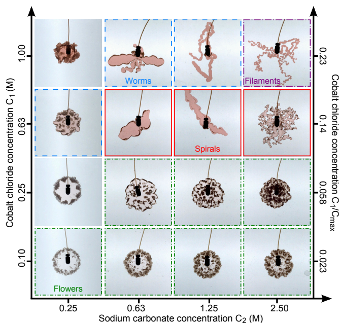
Fig. 6 Phase diagram for \text{CoCl}_2 injected into \text{Na}_2\text{CO}_3 . The injection flow rate is 0.11 mL/s and the field of view is 15 cm \times 15 cm. The images are obtained 15 s after the beginning of the injection.
