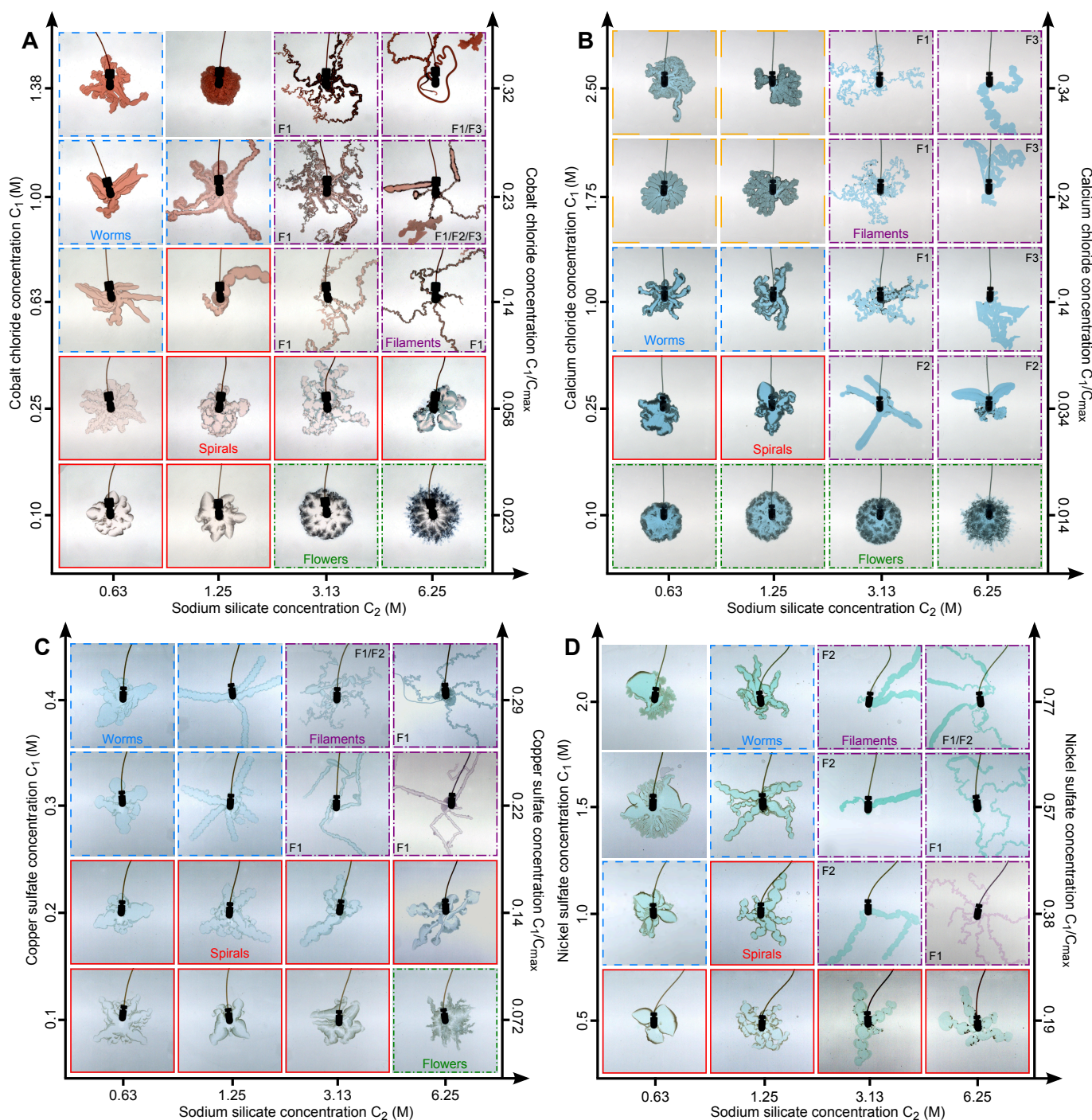
Fig. 2 Phase diagram for \text{CoCl}_2 (A), \text{CaCl}_2 with food colouring (B), \text{CuSO}_4 (C) and \text{NiSO}_4 (D) injected into sodium silicate. A diagram similar to (A) has been published in Ref. 22 The left and right vertical axes show the concentration of the metallic salt solution and this concentration normalized by C_{\text{max}} , the limit of solubility for the metallic salt in water, respectively. C_{\text{max}} = 4.33 M for \text{CoCl}_2 , 7.32 M for \text{CaCl}_2 , 1.38 M for \text{CuSO}_4 and 2.61 M for \text{NiSO}_4 . 23 The horizontal axis shows the concentration of sodium silicate. The injection flow rate is 0.11 mL/s and the field of view is 15 cm \times 15 cm. The images are obtained 15 s after the beginning of the injection, which is the typical time needed to obtain well developed macroscopic patterns in the cell.
